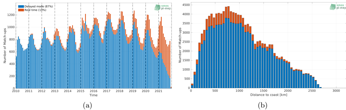
Figure 1: Number of match-ups between Argo and SMOS SSS L3 v7 - 9 Days (CATDS-CECOS-LOCEAN) SSS as a function of time (a) and as function of the distance to coast (b) over the Southern Ocean Pi-MEP region and for the full satellite product period.
