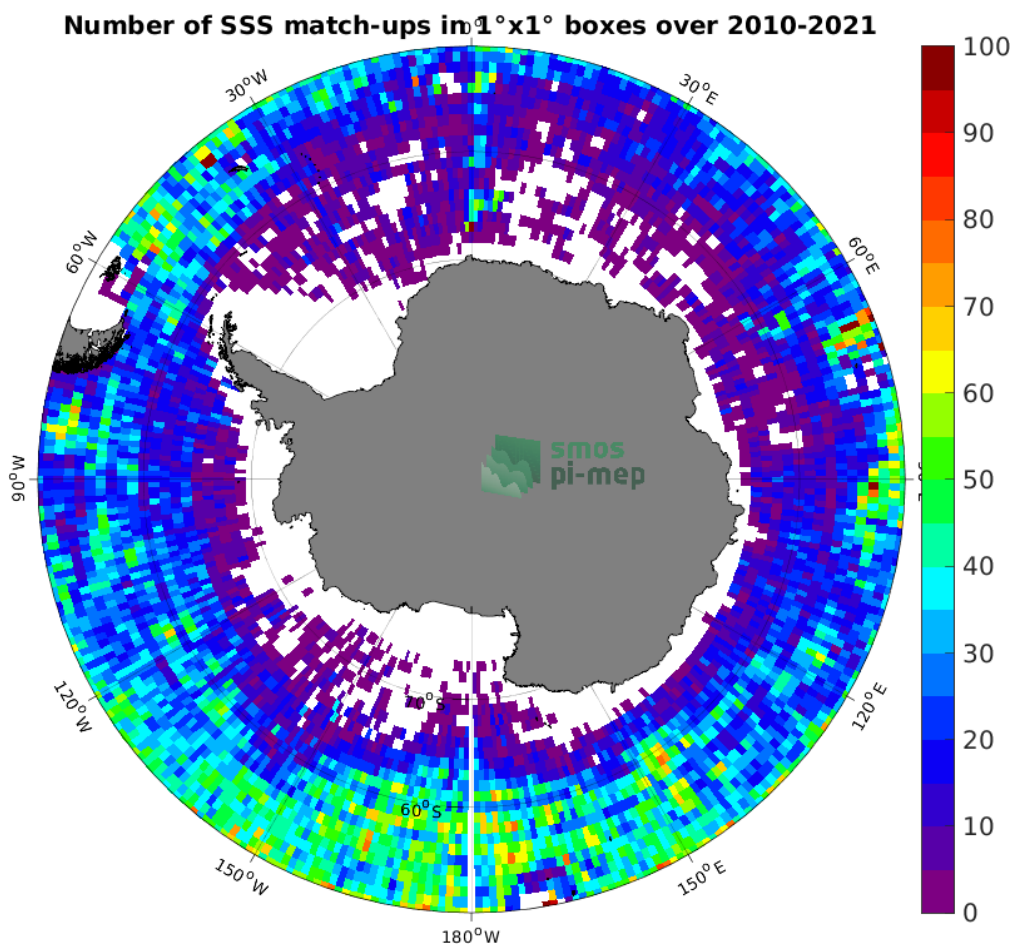
Figure 4: Number of SSS match-ups between Argo SSS and the SMOS SSS L3 v7 - 9 Days (CATDS-CECOS-LOCEAN) SSS product for the Southern Ocean Pi-MEP region over 1^\circ \times 1^\circ boxes and for the full satellite product period.
