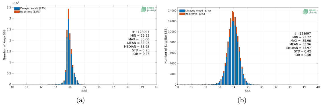
Figure 2: Histograms of SSS from Argo (a) and SMOS SSS L3 v7 - 9 Days (CATDS-CECOS-LOCEAN) (b) considering all match-up pairs per bins of 0.1 over the Southern Ocean Pi-MEP region and for the full satellite product period.
