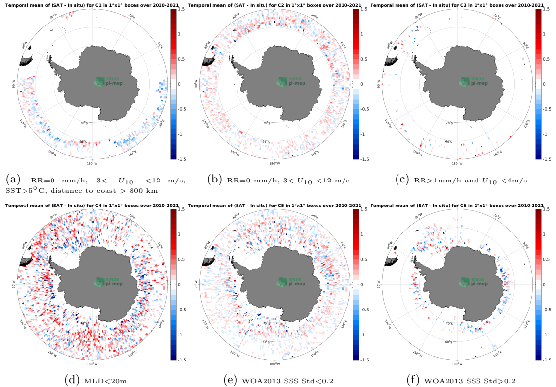
Figure 12: Temporal mean gridded over spatial boxes of size 1^{\circ}\times 1^{\circ} of \Delta\text{SSS} (SMOS SSS L3 v7 - 9 Days (CATDS-CECOS-LOCEAN) - Argo) for 6 different subdatasets corresponding to:RR=0 mm/h, 3 < U_{10} < 12 m/s, SST > 5^{\circ}\text{C} , distance to coast > 800 km (a), RR=0 mm/h, 3 < U_{10} < 12 m/s (b), RR > 1\text{mm/h} and U_{10} < 4\text{m/s} (c),MLD < 20\text{m} (d),WOA2013 SSS Std < 0.2 (e),WOA2013 SSS Std > 0.2 (f).
