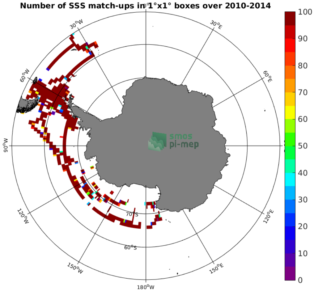
Figure 4: Number of SSS match-ups between TSG (SAMOS) SSS and the SMOS SSS L3 v7 - 18 Days (CATDS-CECOS-LOCEAN) SSS product for the Southern Ocean Pi-MEP region over 1^\circ \times 1^\circ boxes and for the full satellite product period.
