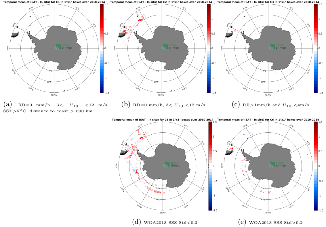
Figure 12: Temporal mean gridded over spatial boxes of size 1^{\circ}\times 1^{\circ} of \Delta\text{SSS} (SMOS SSS L3 v7 - 18 Days (CATDS-CECOS-LOCEAN) - TSG (SAMOS)) for 5 different subdatasets corresponding to:RR=0 mm/h, 3 < U_{10} < 12 m/s, SST >5^{\circ}\text{C} , distance to coast > 800 km (a), RR=0 mm/h, 3 < U_{10} < 12 m/s (b), RR >1 mm/h and U_{10} < 4 m/s (c), WOA2013 SSS Std <0.2 (d), WOA2013 SSS Std >0.2 (e).
