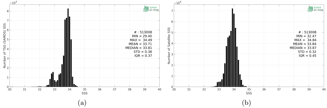
Figure 2: Histograms of SSS from TSG (SAMOS) (a) and SMOS SSS L3 v7 - 18 Days (CATDS-CECOS-LOCEAN) (b) considering all match-up pairs per bins of 0.1 over the Southern Ocean Pi-MEP region and for the full satellite product period.
