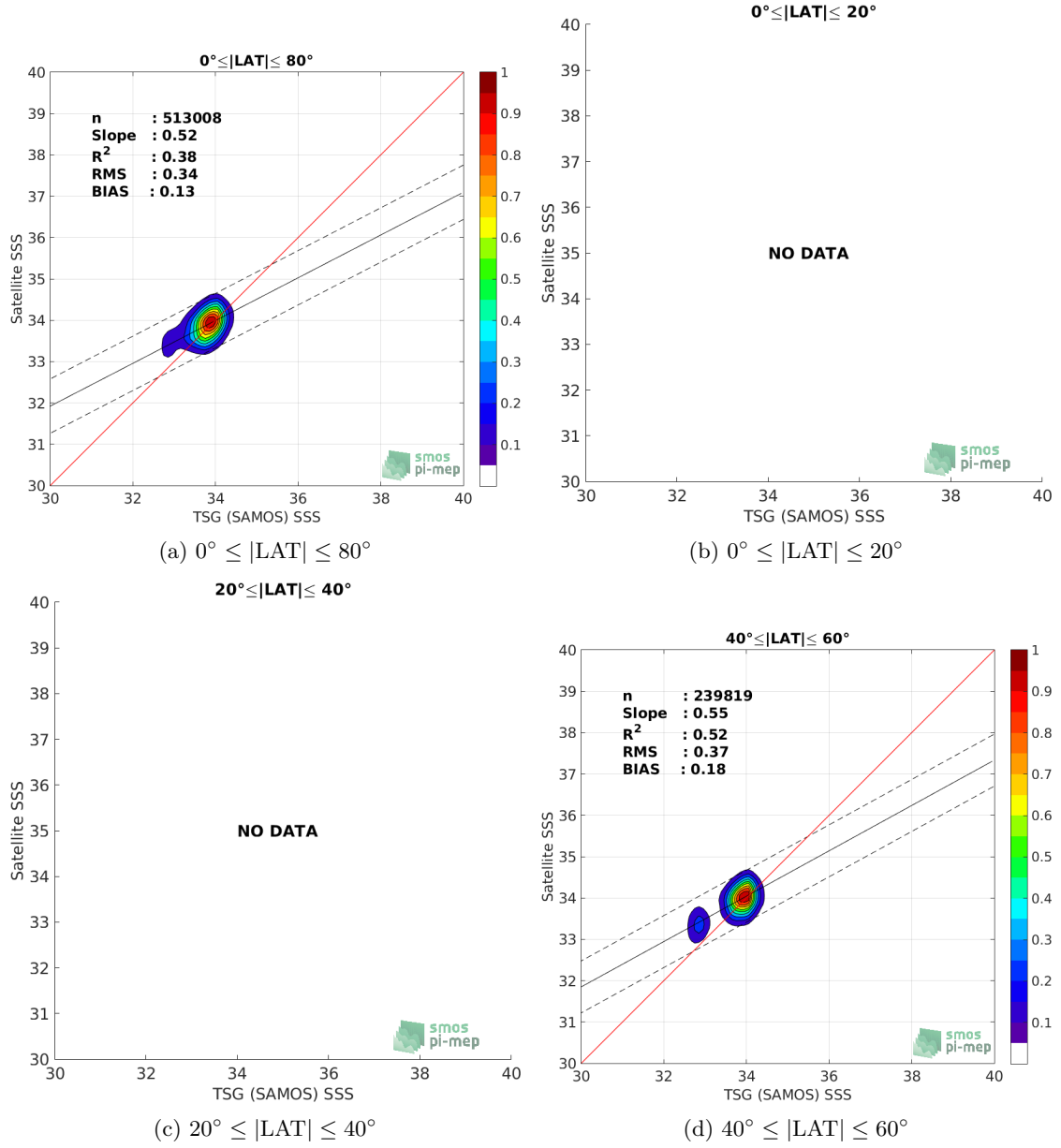
Figure 9: Contour maps of the concentration of SMOS SSS L3 v7 - 18 Days (CATDS-CECOS-LOCEAN) SSS (y-axis) versus TSG (SAMOS) SSS (x-axis) at match-up pairs for different latitude bands. For each plot, the red line shows x=y . The black thin and dashed lines indicate a linear fit through the data cloud and the \pm 95\% confidence levels, respectively. The number match-up pairs n , the slope and R^2 coefficient of the linear fit, the root mean square (RMS) and the mean bias between satellite and in situ data are indicated for each latitude band in each plots.
