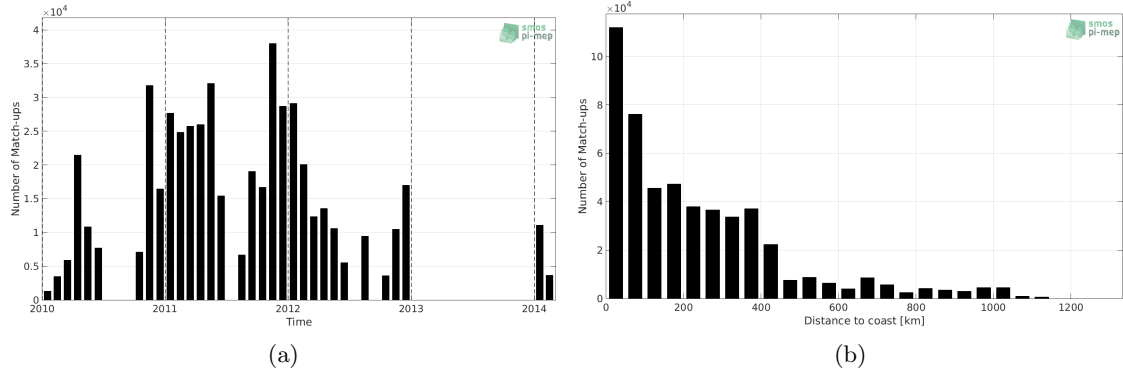
Figure 1: Number of match-ups between TSG (SAMOS) and SMOS SSS L3 v7 - 18 Days (CATDS-CECOS-LOCEAN) SSS as a function of time (a) and as function of the distance to coast (b) over the Southern Ocean Pi-MEP region and for the full satellite product period.
