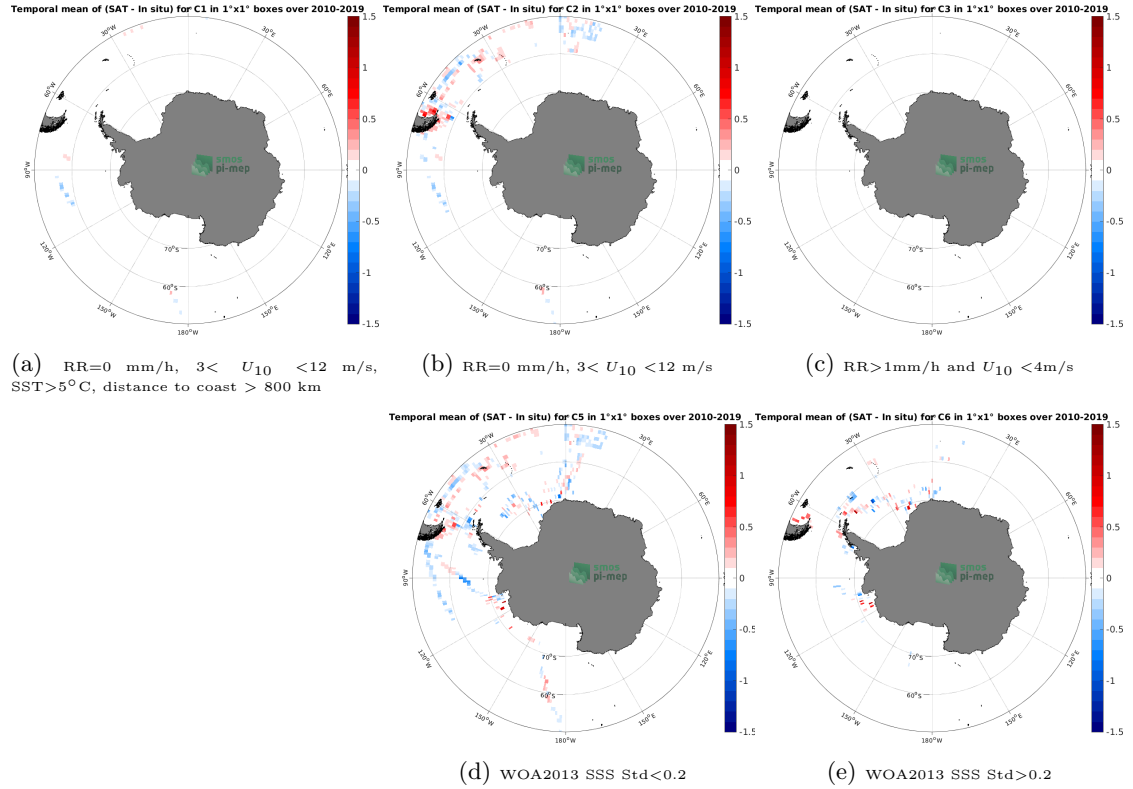
Figure 12: Temporal mean gridded over spatial boxes of size 1^{\circ}\times 1^{\circ} of \Delta\text{SSS} (SMOS SSS L3 v7 - 18 Days (CATDS-CECOS-LOCEAN) - TSG (Polarstern)) for 5 different subdatasets corresponding to:RR=0 mm/h, 3 < U_{10} < 12 m/s, SST >5^{\circ}\text{C} , distance to coast > 800 km (a), RR=0 mm/h, 3 < U_{10} < 12 m/s (b), RR >1 mm/h and U_{10} < 4 m/s (c), WOA2013 SSS Std <0.2 (d), WOA2013 SSS Std >0.2 (e).
