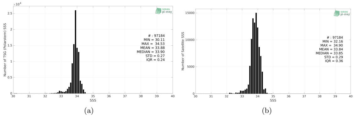
Figure 2: Histograms of SSS from TSG (Polarstern) (a) and SMOS SSS L3 v7 - 18 Days (CATDS-CECOS-LOCEAN) (b) considering all match-up pairs per bins of 0.1 over the Southern Ocean Pi-MEP region and for the full satellite product period.
