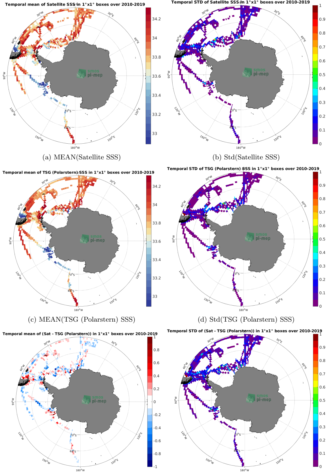
Figure 6: Temporal mean (left) and Std (right) of SSS from SMOS SSS L3 v7 - 18 Days (CATDS-CECOS-LOCEAN) (top), TSG (Polarstern) (middle), and of \Delta SSS (Satellite - TSG (Polarstern)). Only match-up pairs are used to generate these maps.
