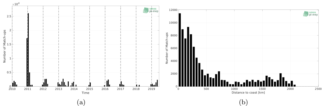
Figure 1: Number of match-ups between TSG (Polarstern) and SMOS SSS L3 v7 - 18 Days (CATDS-CECOS-LOCEAN) SSS as a function of time (a) and as function of the distance to coast (b) over the Southern Ocean Pi-MEP region and for the full satellite product period.
