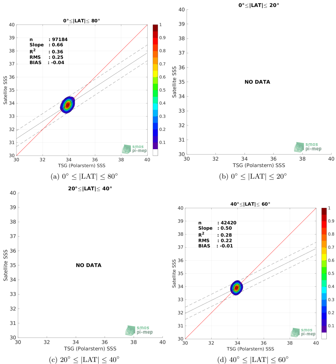
Figure 9: Contour maps of the concentration of SMOS SSS L3 v7 - 18 Days (CATDS-CECOS-LOCEAN) SSS (y-axis) versus TSG (Polarstern) SSS (x-axis) at match-up pairs for different latitude bands. For each plot, the red line shows x=y . The black thin and dashed lines indicate a linear fit through the data cloud and the \pm 95\% confidence levels, respectively. The number match-up pairs n , the slope and R^2 coefficient of the linear fit, the root mean square (RMS) and the mean bias between satellite and in situ data are indicated for each latitude band in each plots.
