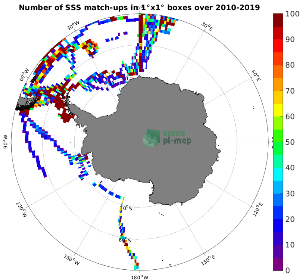
Figure 4: Number of SSS match-ups between TSG (Polarstern) SSS and the SMOS SSS L3 v7 - 18 Days (CATDS-CECOS-LOCEAN) SSS product for the Southern Ocean Pi-MEP region over 1^\circ \times 1^\circ boxes and for the full satellite product period.
