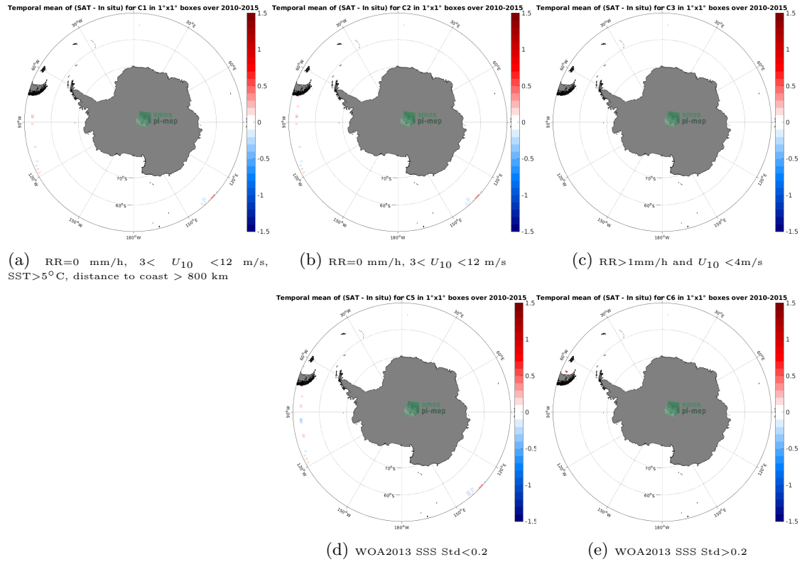
Figure 12: Temporal mean gridded over spatial boxes of size 1^\circ \times 1^\circ of \Delta SSS (SMOS SSS L3 v7 - 18 Days (CATDS-CECOS-LOCEAN) - TSG (GOSUD-Research-vessel)) for 5 different sub-datasets corresponding to: RR=0 mm/h, 3 < U_{10} < 12 m/s, SST>5°C, distance to coast > 800 km (a), RR=0 mm/h, 3 < U_{10} < 12 m/s (b), RR>1mm/h and U_{10} < 4 m/s (c), WOA2013 SSS Std<0.2 (d), WOA2013 SSS Std>0.2 (e).
