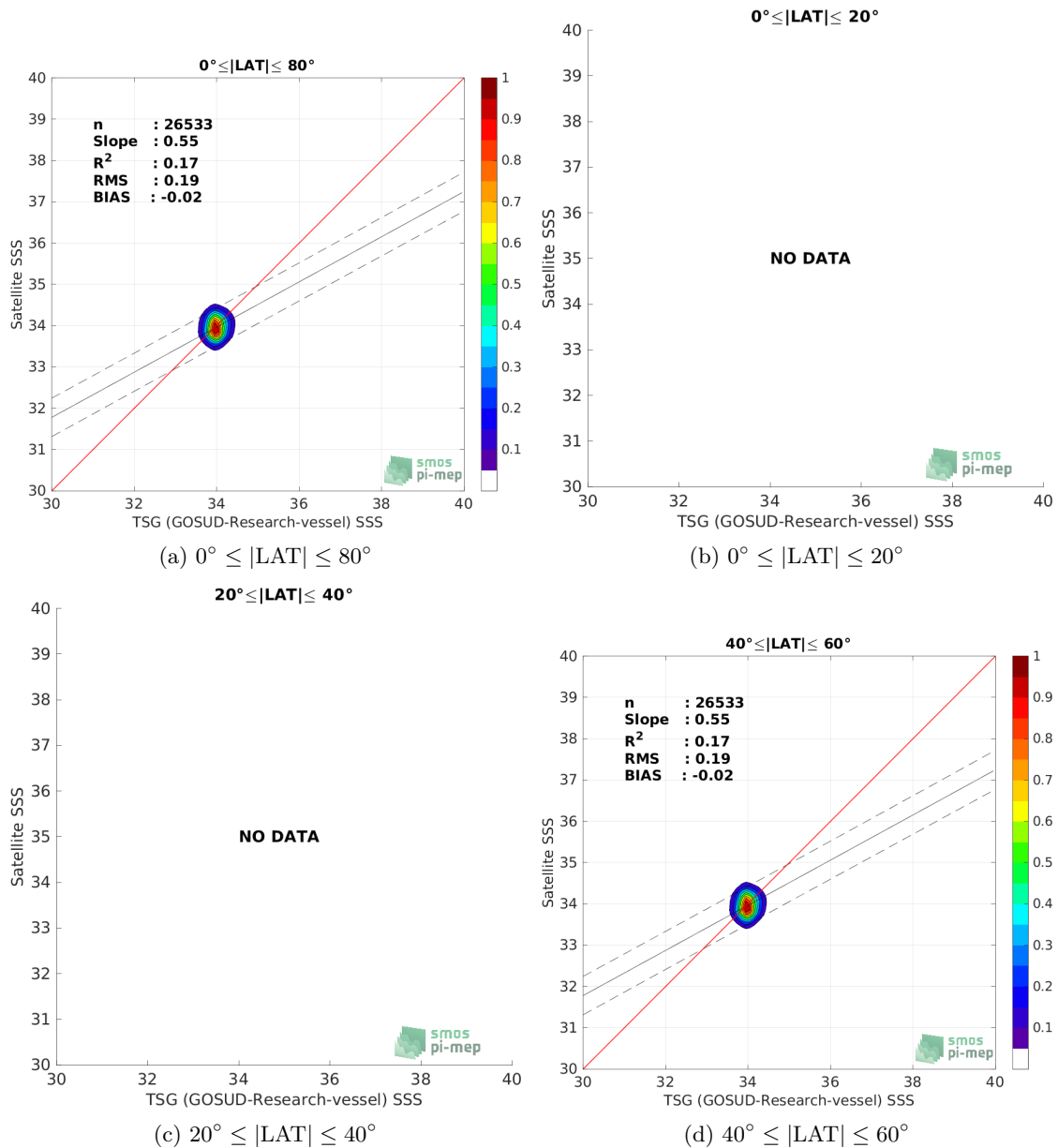
Figure 9: Contour maps of the concentration of SMOS SSS L3 v7 - 18 Days (CATDS-CECOS-LOCEAN) SSS (y-axis) versus TSG (GOSUD-Research-vessel) SSS (x-axis) at match-up pairs for different latitude bands. For each plot, the red line shows x=y . The black thin and dashed lines indicate a linear fit through the data cloud and the \pm 95\% confidence levels, respectively. The number match-up pairs n , the slope and R^2 coefficient of the linear fit, the root mean square (RMS) and the mean bias between satellite and in situ data are indicated for each latitude band in each plots.
