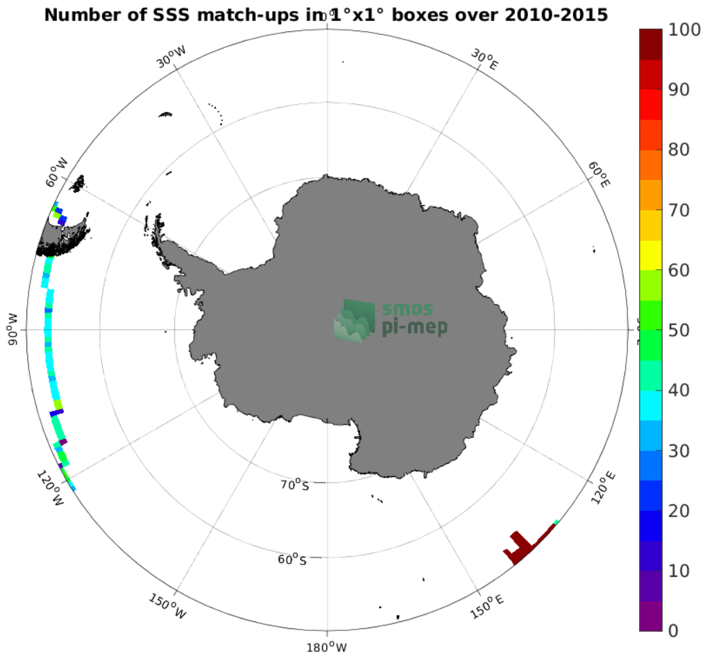
Figure 4: Number of SSS match-ups between TSG (GOSUD-Research-vessel) SSS and the SMOS SSS L3 v7 - 18 Days (CATDS-CECOS-LOCEAN) SSS product for the Southern Ocean Pi-MEP region over 1^\circ \times 1^\circ boxes and for the full satellite product period.
