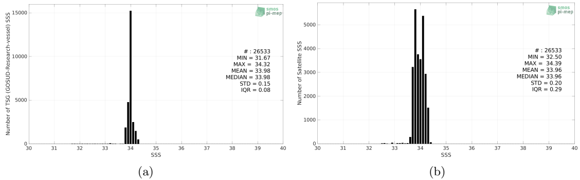
Figure 2: Histograms of SSS from TSG (GOSUD-Research-vessel) (a) and SMOS SSS L3 v7 - 18 Days (CATDS-CECOS-LOCEAN) (b) considering all match-up pairs per bins of 0.1 over the Southern Ocean Pi-MEP region and for the full satellite product period.
