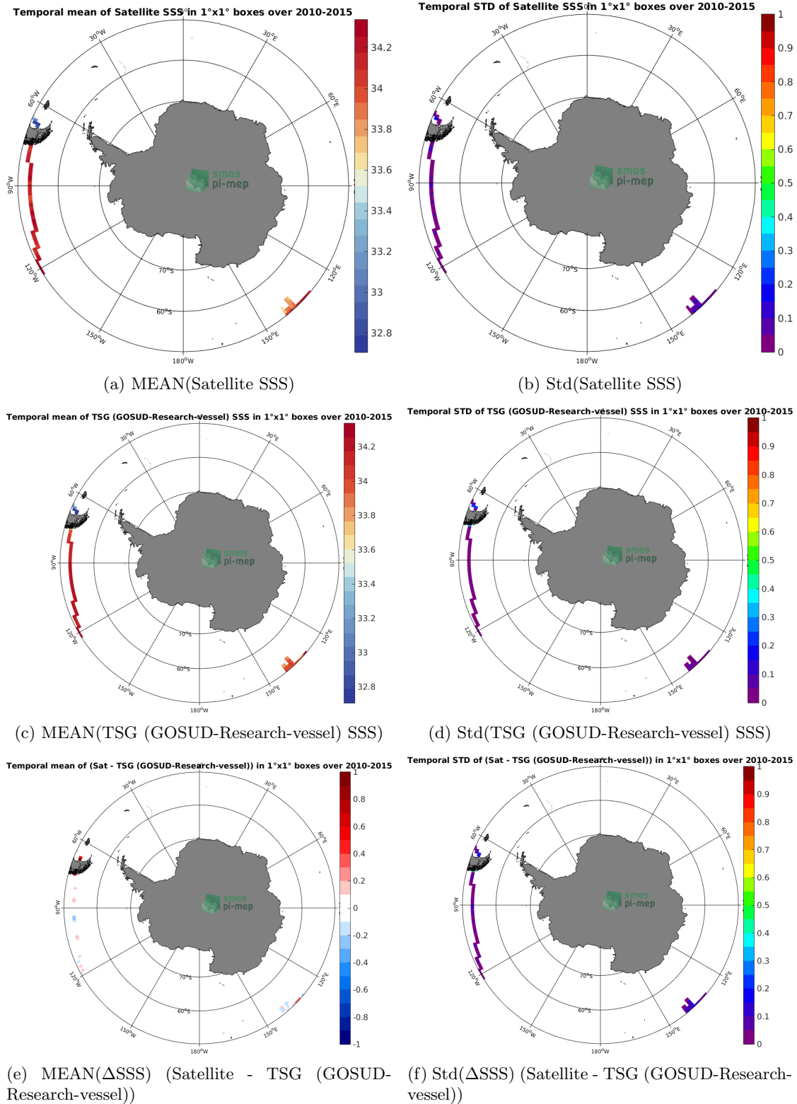
Figure 6: Temporal mean (left) and Std (right) of SSS from SMOS SSS L3 v7 - 18 Days (CATDS-CECOS-LOCEAN) (top), TSG (GOSUD-Research-vessel) (middle), and of \Delta SSS (Satellite - TSG (GOSUD-Research-vessel)). Only match-up pairs are used to generate these maps.
