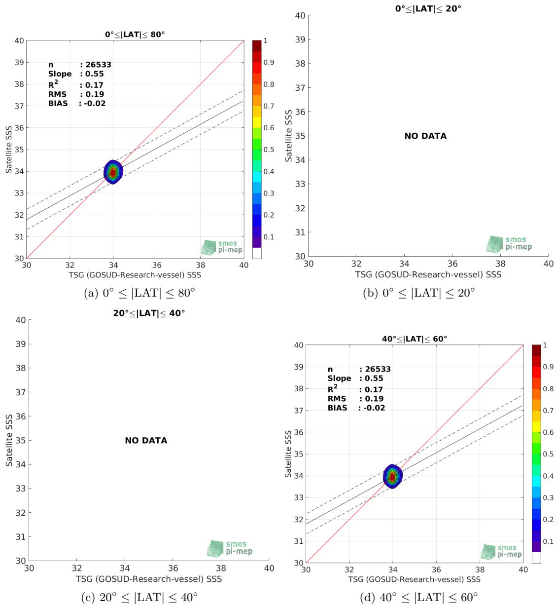
Figure 9: Contour maps of the concentration of SMOS SSS L3 v7 - 18 Days (CATDS-CECOS-LOCEAN) SSS ( y -axis) versus TSG (GOSUD-Research-vessel) SSS ( x -axis) at match-up pairs for different latitude bands. For each plot, the red line shows x=y . The black thin and dashed lines indicate a linear fit through the data cloud and the \pm 95\% confidence levels, respectively. The number match-up pairs n , the slope and R^2 coefficient of the linear fit, the root mean square (RMS) and the mean bias between satellite and in situ data are indicated for each latitude band in each plots.
