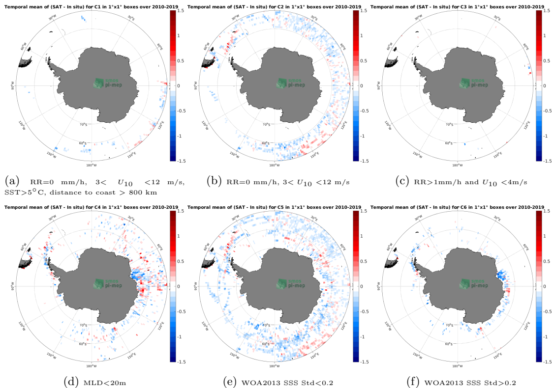
Figure 12: Temporal mean gridded over spatial boxes of size 1^{\circ}\times 1^{\circ} of \Delta\text{SSS} (SMOS SSS L3 v7 - 18 Days (CATDS-CECOS-LOCEAN) - Marine mammals) for 6 different subdatasets corresponding to:RR=0 mm/h, 3 < U_{10} < 12 m/s, SST >5^{\circ}\text{C} , distance to coast > 800 km (a), RR=0 mm/h, 3 < U_{10} < 12 m/s (b), RR >1 mm/h and U_{10} < 4 m/s (c),MLD <20 m (d),WOA2013 SSS Std <0.2 (e),WOA2013 SSS Std >0.2 (f).
