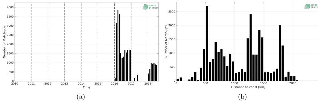
Figure 1: Number of match-ups between Surface drifters and SMOS SSS L3 v7 - 18 Days (CATDS-CECOS-LOCEAN) SSS as a function of time (a) and as function of the distance to coast (b) over the Southern Ocean Pi-MEP region and for the full satellite product period.
