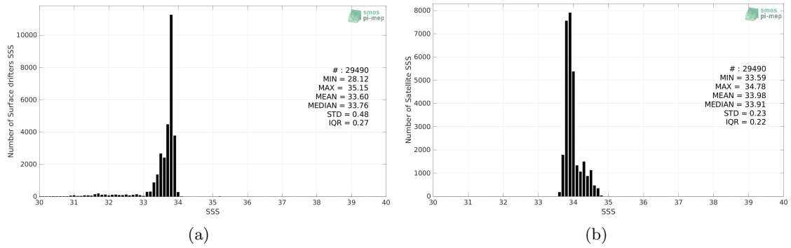
Figure 2: Histograms of SSS from Surface drifters (a) and SMOS SSS L3 v7 - 18 Days (CATDS-CECOS-LOCEAN) (b) considering all match-up pairs per bins of 0.1 over the Southern Ocean Pi-MEP region and for the full satellite product period.
