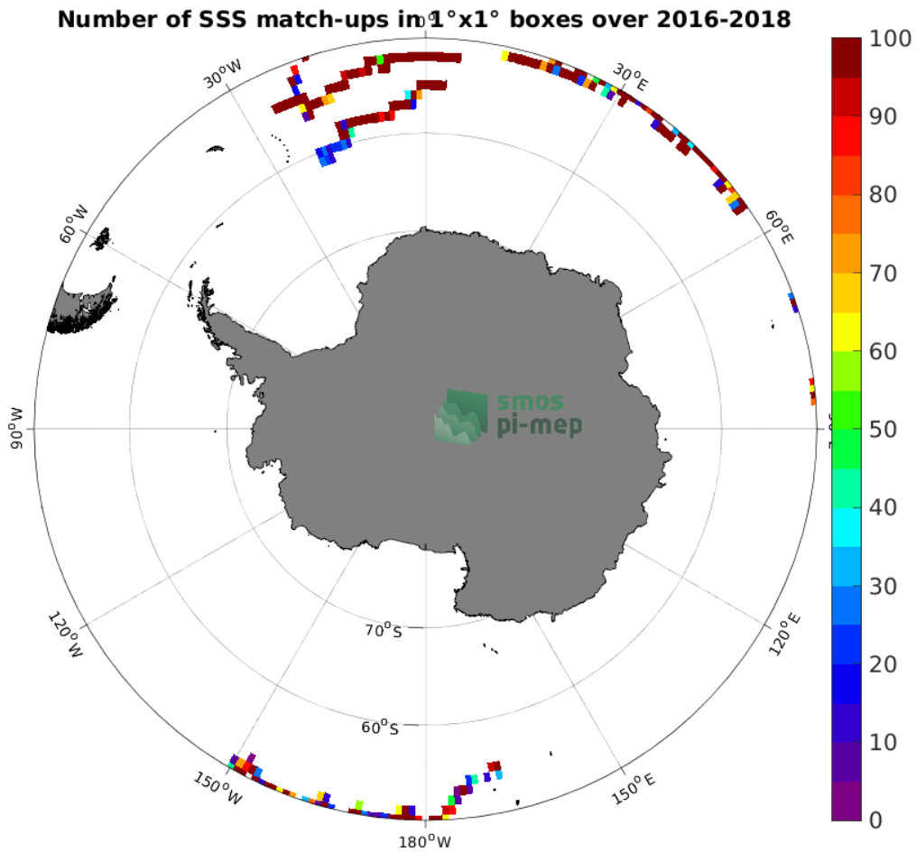
Figure 3: Number of SSS match-ups between Surface drifters SSS and the SMOS SSS L3 v7 - 18 Days (CATDS-CECOS-LOCEAN) SSS product for the Southern Ocean Pi-MEP region over 1^\circ \times 1^\circ boxes and for the full satellite product period.
