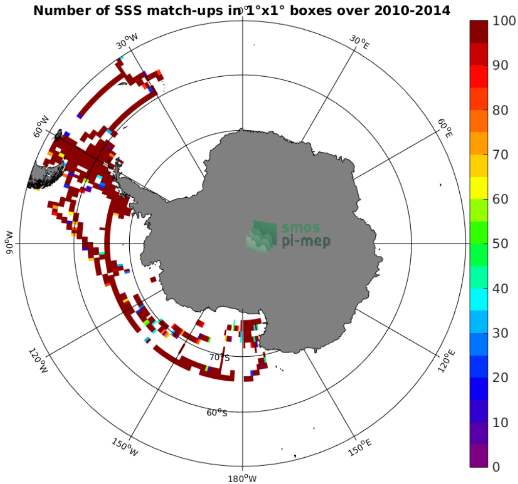
Figure 4: Number of SSS match-ups between TSG (SAMOS) SSS and the SMOS SSS L3 v5 - 9 Days (CATDS-CECOS-LOCEAN) SSS product for the Southern Ocean Pi-MEP region over 1^\circ \times 1^\circ boxes and for the full satellite product period.
