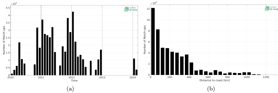
Figure 1: Number of match-ups between TSG (SAMOS) and SMOS SSS L3 v5 - 9 Days (CATDS-CECOS-LOCEAN) SSS as a function of time (a) and as function of the distance to coast (b) over the Southern Ocean Pi-MEP region and for the full satellite product period.
