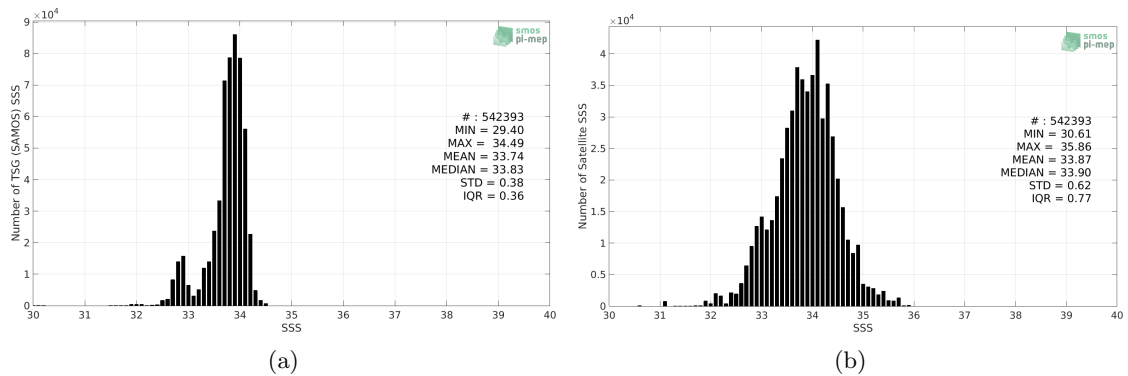
Figure 2: Histograms of SSS from TSG (SAMOS) (a) and SMOS SSS L3 v5 - 9 Days (CATDS-CECOS-LOCEAN) (b) considering all match-up pairs per bins of 0.1 over the Southern Ocean Pi-MEP region and for the full satellite product period.
