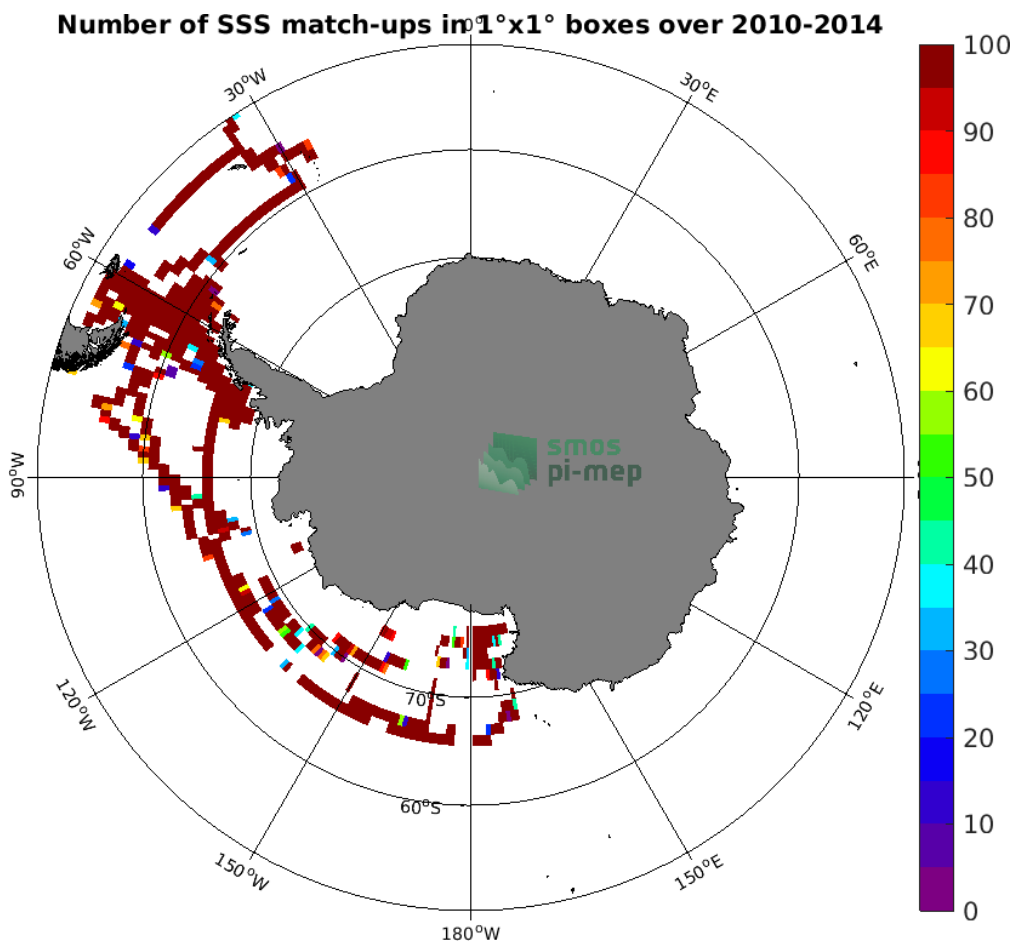
Figure 4: Number of SSS match-ups between TSG (SAMOS) SSS and the SMOS SSS L3 v5 - 9 Days (CATDS-CECOS-LOCEAN) SSS product for the Southern Ocean Pi-MEP region over 1°x1° boxes and for the full satellite product period.
