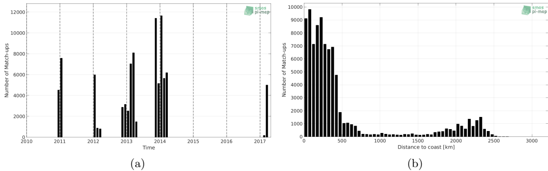
Figure 1: Number of match-ups between TSG (GOSUD-Sailing-ship) and SMOS SSS L3 v5 - 9 Days (CATDS-CECOS-LOCEAN) SSS as a function of time (a) and as function of the distance to coast (b) over the Southern Ocean Pi-MEP region and for the full satellite product period.
