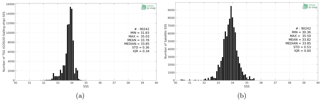
Figure 2: Histograms of SSS from TSG (GOSUD-Sailing-ship) (a) and SMOS SSS L3 v5 - 9 Days (CATDS-CECOS-LOCEAN) (b) considering all match-up pairs per bins of 0.1 over the Southern Ocean Pi-MEP region and for the full satellite product period.
