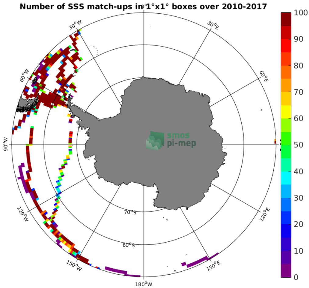
Figure 4: Number of SSS match-ups between TSG (GOSUD-Sailing-ship) SSS and the SMOS SSS L3 v5 - 9 Days (CATDS-CECOS-LOCEAN) SSS product for the Southern Ocean Pi-MEP region over 1^\circ \times 1^\circ boxes and for the full satellite product period.
