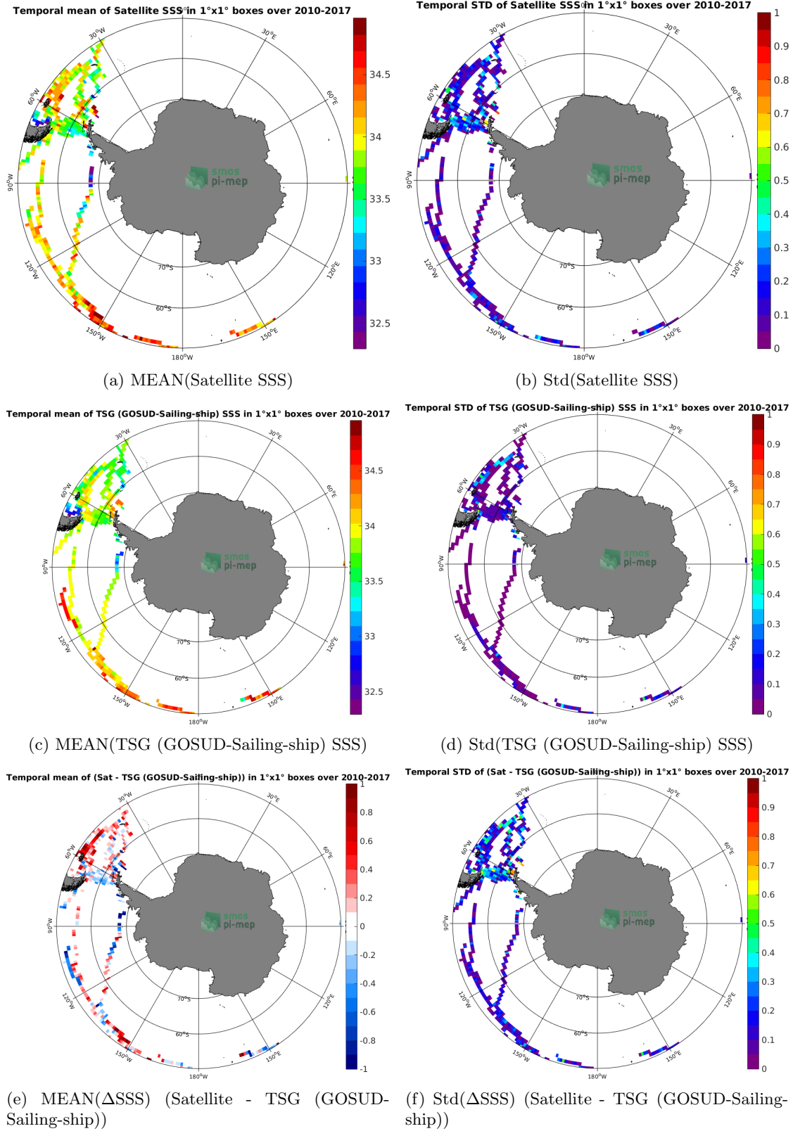
Figure 6: Temporal mean (left) and Std (right) of SSS from SMOS SSS L3 v5 - 9 Days (CATDS-CECOS-LOCEAN) (top), TSG (GOSUD-Sailing-ship) (middle), and of \Delta SSS (Satellite - TSG (GOSUD-Sailing-ship)). Only match-up pairs are used to generate these maps.
