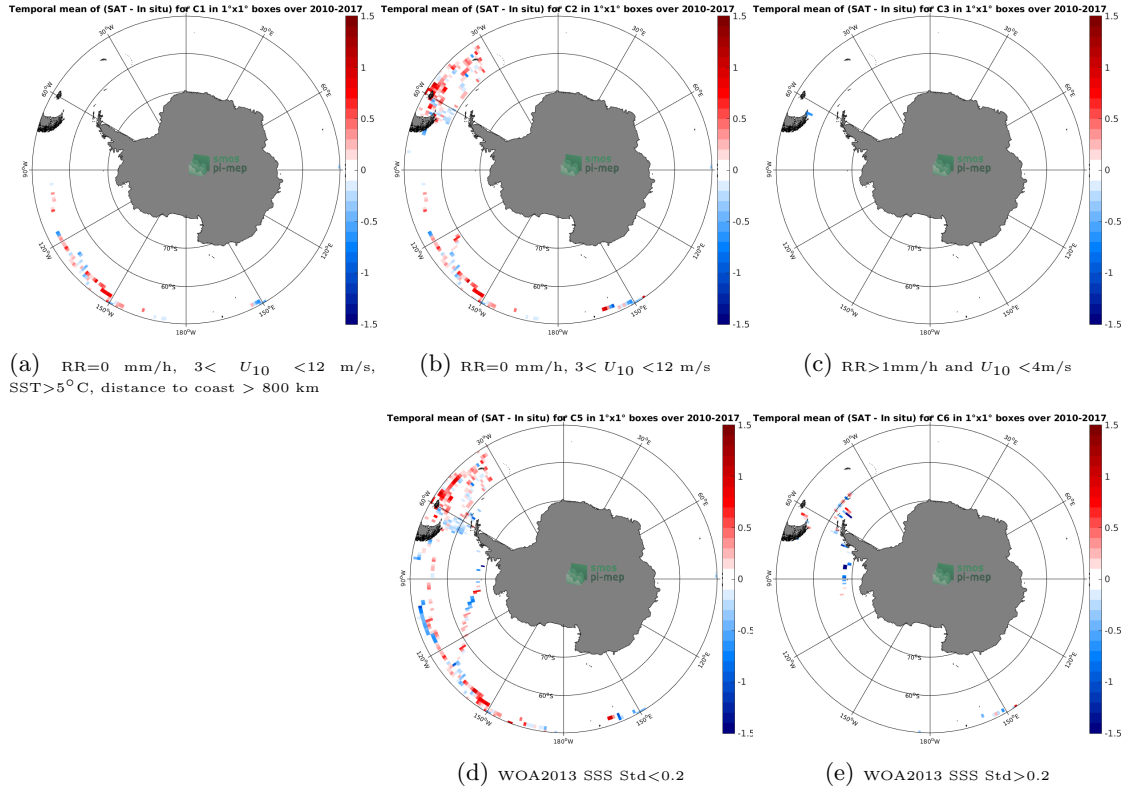
Figure 12: Temporal mean gridded over spatial boxes of size 1°x1° of \Delta SSS (SMOS SSS L3 v5 - 9 Days (CATDS-CECOS-LOCEAN) - TSG (GOSUD-Sailing-ship)) for 5 different subdatasets corresponding to: RR=0 mm/h, 3 < U_{10} < 12 m/s, SST > 5°C, distance to coast > 800 km (a), RR=0 mm/h, 3 < U_{10} < 12 m/s (b), RR > 1mm/h and U_{10} < 4 m/s (c), WOA2013 SSS Std < 0.2 (d), WOA2013 SSS Std > 0.2 (e).
