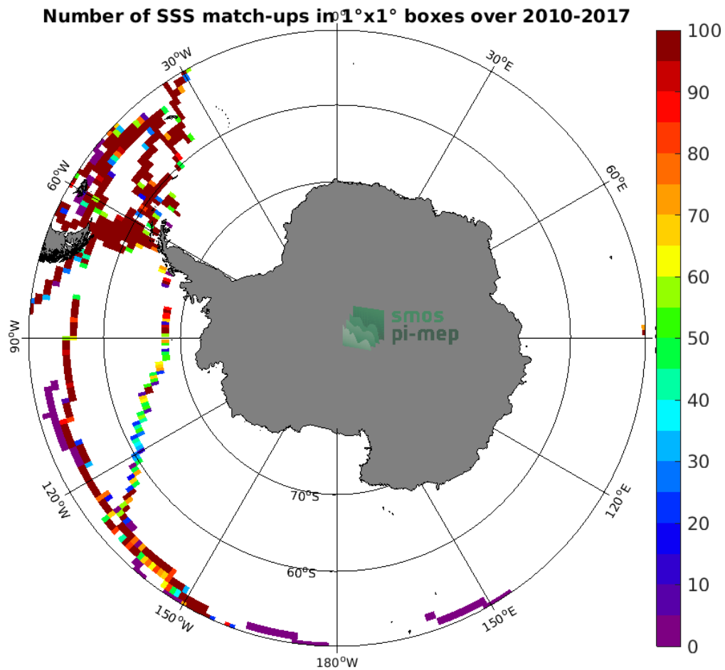
Figure 4: Number of SSS match-ups between TSG (GOSUD-Sailing-ship) SSS and the SMOS SSS L3 v5 - 9 Days (CATDS-CECOS-LOCEAN) SSS product for the Southern Ocean Pi-MEP region over 1°x1° boxes and for the full satellite product period.
