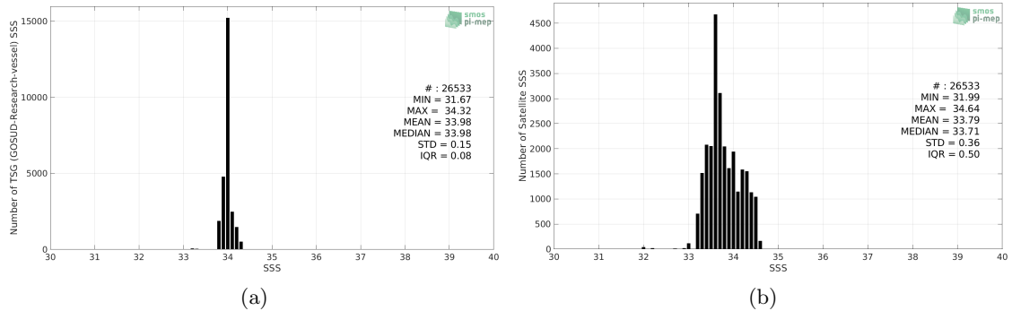
Figure 2: Histograms of SSS from TSG (GOSUD-Research-vessel) (a) and SMOS SSS L3 v5 - 9 Days (CATDS-CECOS-LOCEAN) (b) considering all match-up pairs per bins of 0.1 over the Southern Ocean Pi-MEP region and for the full satellite product period.
