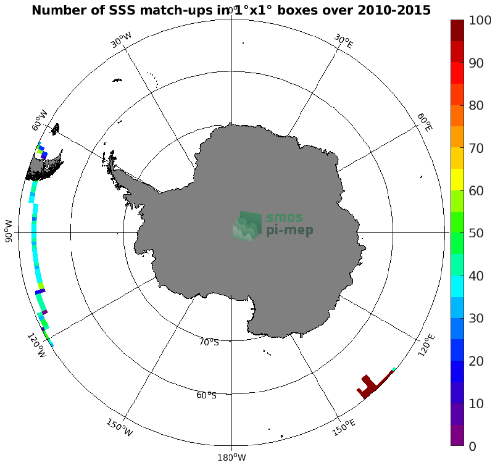
Figure 4: Number of SSS match-ups between TSG (GOSUD-Research-vessel) SSS and the SMOS SSS L3 v5 - 9 Days (CATDS-CECOS-LOCEAN) SSS product for the Southern Ocean Pi-MEP region over 1^\circ \times 1^\circ boxes and for the full satellite product period.
