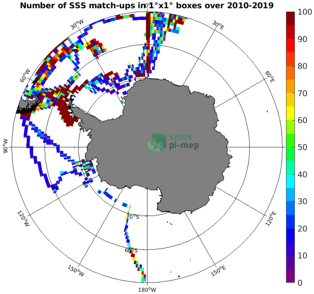
Figure 4: Number of SSS match-ups between TSG (Polarstern) SSS and the SMOS SSS L3 v5 - 18 Days (CATDS-CECOS-LOCEAN) SSS product for the Southern Ocean Pi-MEP region over 1^\circ \times 1^\circ boxes and for the full satellite product period.
