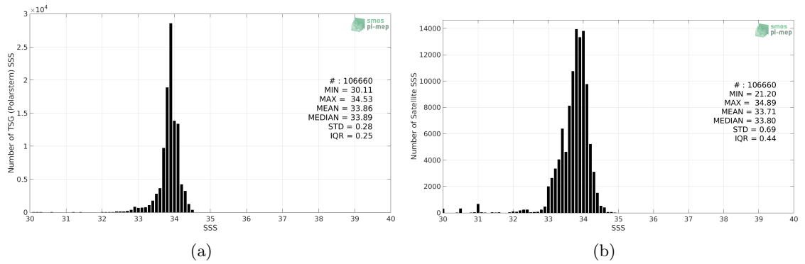
Figure 2: Histograms of SSS from TSG (Polarstern) (a) and SMOS SSS L3 v5 - 18 Days (CATDS-CECOS-LOCEAN) (b) considering all match-up pairs per bins of 0.1 over the Southern Ocean Pi-MEP region and for the full satellite product period.
