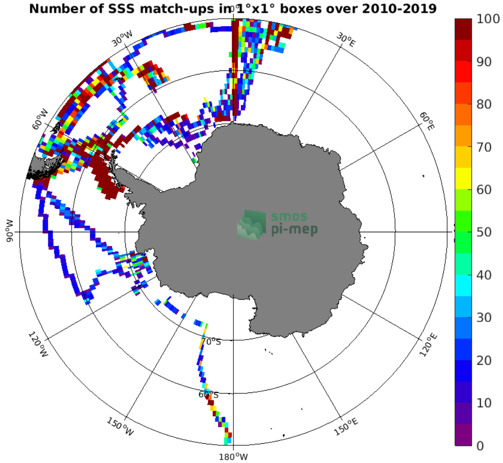
Figure 4: Number of SSS match-ups between TSG (Polarstern) SSS and the SMOS SSS L3 v5 - 18 Days (CATDS-CECOS-LOCEAN) SSS product for the Southern Ocean Pi-MEP region over 1^\circ \times 1^\circ boxes and for the full satellite product period.
