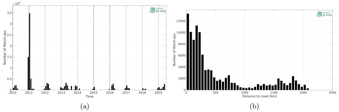
Figure 1: Number of match-ups between TSG (Polarstern) and SMOS SSS L3 v5 - 18 Days (CATDS-CECOS-LOCEAN) SSS as a function of time (a) and as function of the distance to coast (b) over the Southern Ocean Pi-MEP region and for the full satellite product period.
