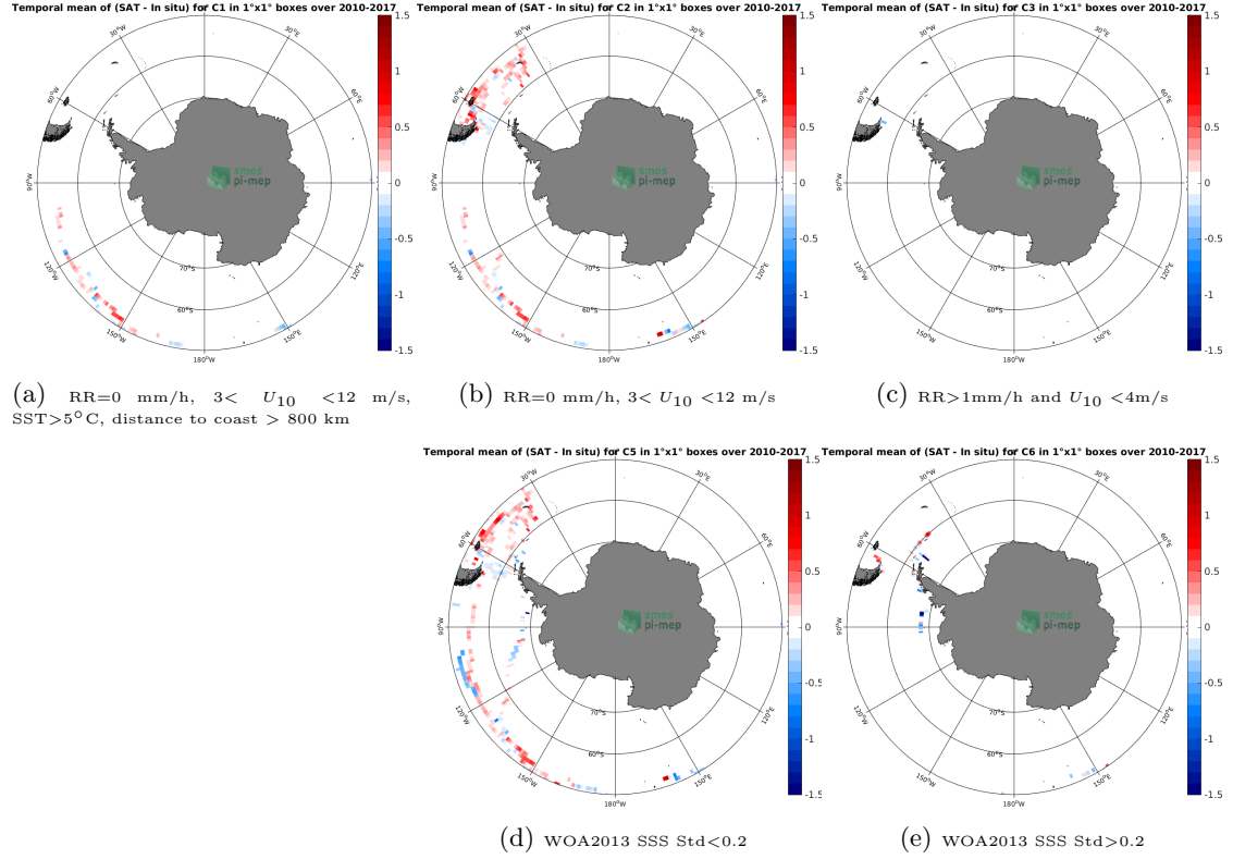
Figure 12: Temporal mean gridded over spatial boxes of size 1^\circ \times 1^\circ of \Delta SSS (SMOS SSS L3 v5 - 18 Days (CATDS-CECOS-LOCEAN) - TSG (GOSUD-Sailing-ship)) for 5 different subdatasets corresponding to: RR=0 mm/h, 3 < U_{10} < 12 m/s, SST>5°C, distance to coast > 800 km (a), RR=0 mm/h, 3 < U_{10} < 12 m/s (b), RR>1mm/h and U_{10} < 4 m/s (c), WOA2013 SSS Std<0.2 (d), WOA2013 SSS Std>0.2 (e).
