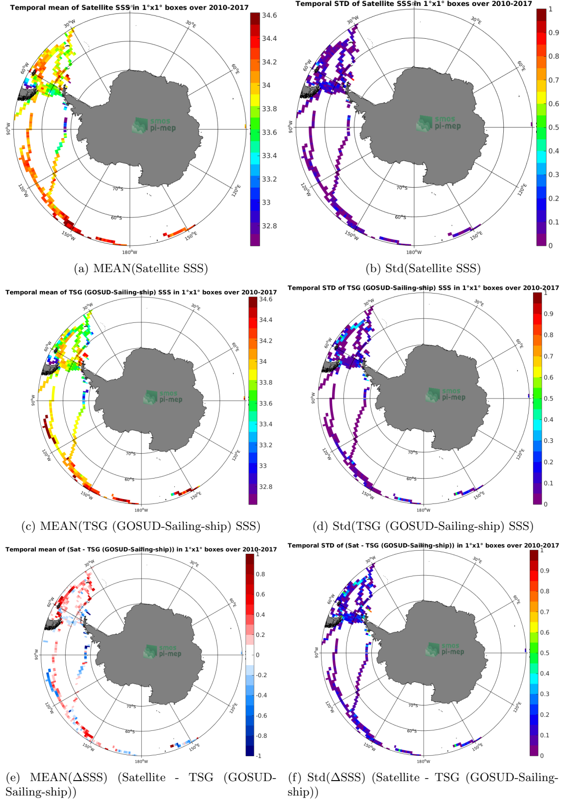
Figure 6: Temporal mean (left) and Std (right) of SSS from SMOS SSS L3 v5 - 18 Days (CATDS-CECOS-LOCEAN) (top), TSG (GOSUD-Sailing-ship) (middle), and of \Delta SSS (Satellite - TSG (GOSUD-Sailing-ship)). Only match-up pairs are used to generate these maps.
