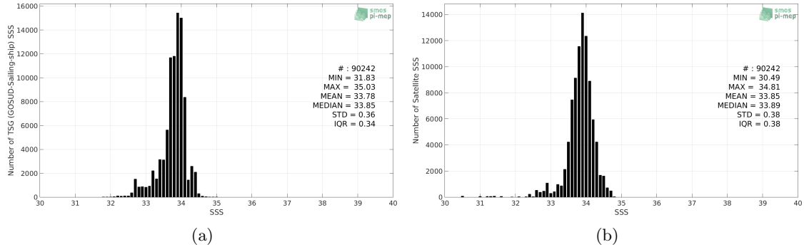
Figure 2: Histograms of SSS from TSG (GOSUD-Sailing-ship) (a) and SMOS SSS L3 v5 - 18 Days (CATDS-CECOS-LOCEAN) (b) considering all match-up pairs per bins of 0.1 over the Southern Ocean Pi-MEP region and for the full satellite product period.
