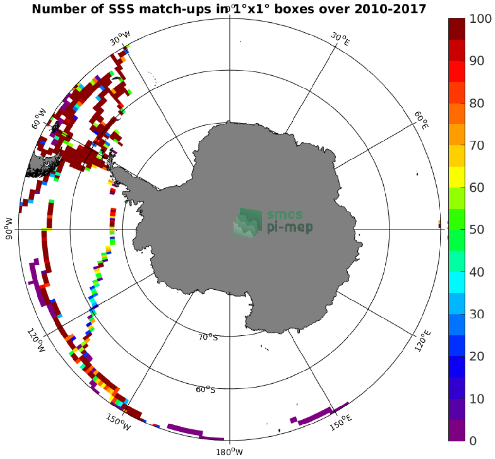
Figure 4: Number of SSS match-ups between TSG (GOSUD-Sailing-ship) SSS and the SMOS SSS L3 v5 - 18 Days (CATDS-CECOS-LOCEAN) SSS product for the Southern Ocean Pi-MEP region over 1^\circ \times 1^\circ boxes and for the full satellite product period.
