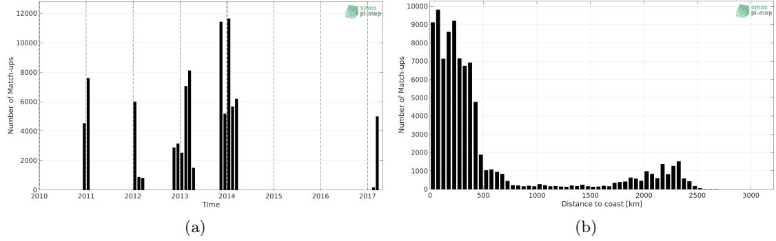
Figure 1: Number of match-ups between TSG (GOSUD-Sailing-ship) and SMOS SSS L3 v5 - 18 Days (CATDS-CECOS-LOCEAN) SSS as a function of time (a) and as function of the distance to coast (b) over the Southern Ocean Pi-MEP region and for the full satellite product period.
