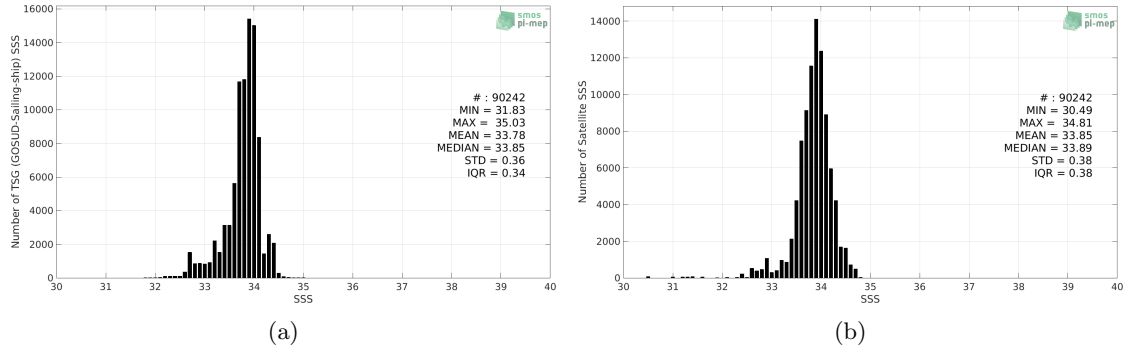
Figure 2: Histograms of SSS from TSG (GOSUD-Sailing-ship) (a) and SMOS SSS L3 v5 - 18 Days (CATDS-CECOS-LOCEAN) (b) considering all match-up pairs per bins of 0.1 over the Southern Ocean Pi-MEP region and for the full satellite product period.
