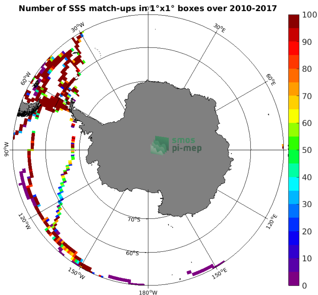
Figure 4: Number of SSS match-ups between TSG (GOSUD-Sailing-ship) SSS and the SMOS SSS L3 v5 - 18 Days (CATDS-CECOS-LOCEAN) SSS product for the Southern Ocean Pi-MEP region over 1^\circ \times 1^\circ boxes and for the full satellite product period.
