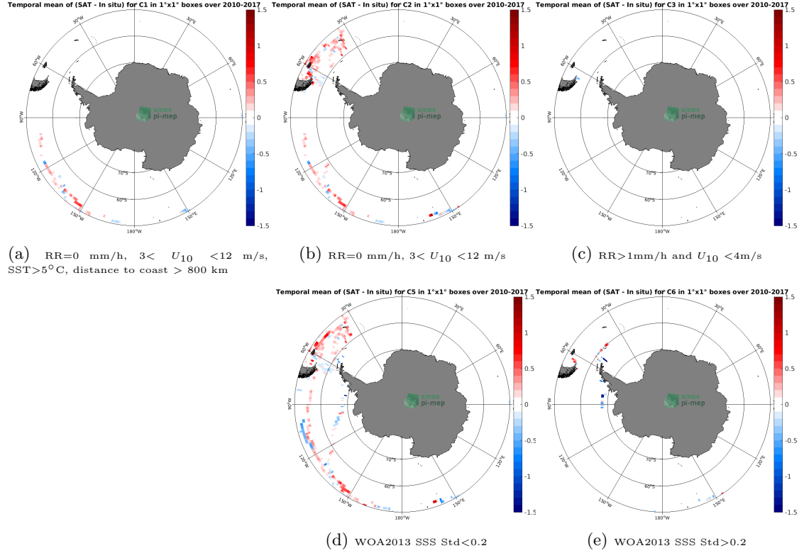
Figure 12: Temporal mean gridded over spatial boxes of size 1°x1° of \Delta\text{SSS} (SMOS SSS L3 v5 - 18 Days (CATDS-CECOS-LOCEAN) - TSG (GOSUD-Sailing-ship)) for 5 different subdatasets corresponding to: RR=0 mm/h, 3 < U_{10} < 12 m/s, SST > 5^\circ\text{C} , distance to coast > 800 km (a), RR=0 mm/h, 3 < U_{10} < 12 m/s (b), RR > 1 mm/h and U_{10} < 4 m/s (c), WOA2013 SSS Std < 0.2 (d), WOA2013 SSS Std > 0.2 (e).
