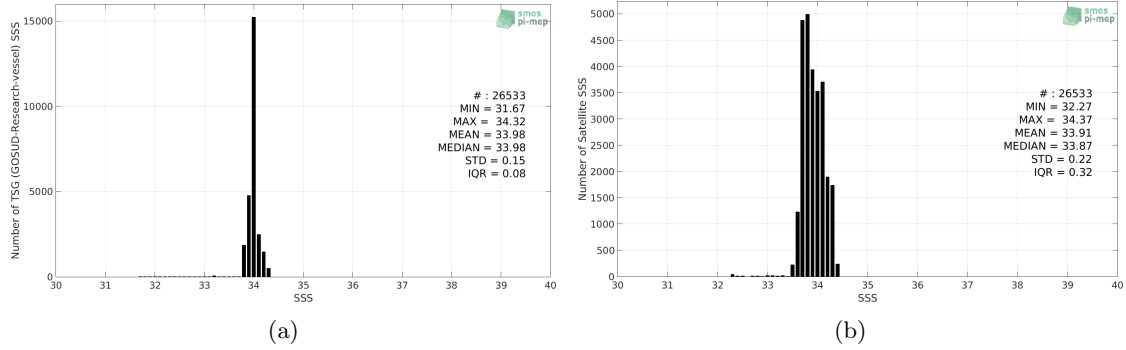
Figure 2: Histograms of SSS from TSG (GOSUD-Research-vessel) (a) and SMOS SSS L3 v5 - 18 Days (CATDS-CECOS-LOCEAN) (b) considering all match-up pairs per bins of 0.1 over the Southern Ocean Pi-MEP region and for the full satellite product period.
