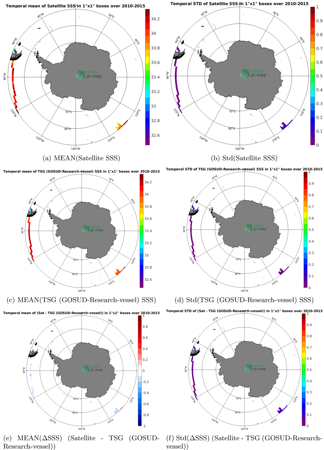
Figure 6: Temporal mean (left) and Std (right) of SSS from SMOS SSS L3 v5 - 18 Days (CATDS-CECOS-LOCEAN) (top), TSG (GOSUD-Research-vessel) (middle), and of \Delta SSS (Satellite - TSG (GOSUD-Research-vessel)). Only match-up pairs are used to generate these maps.
