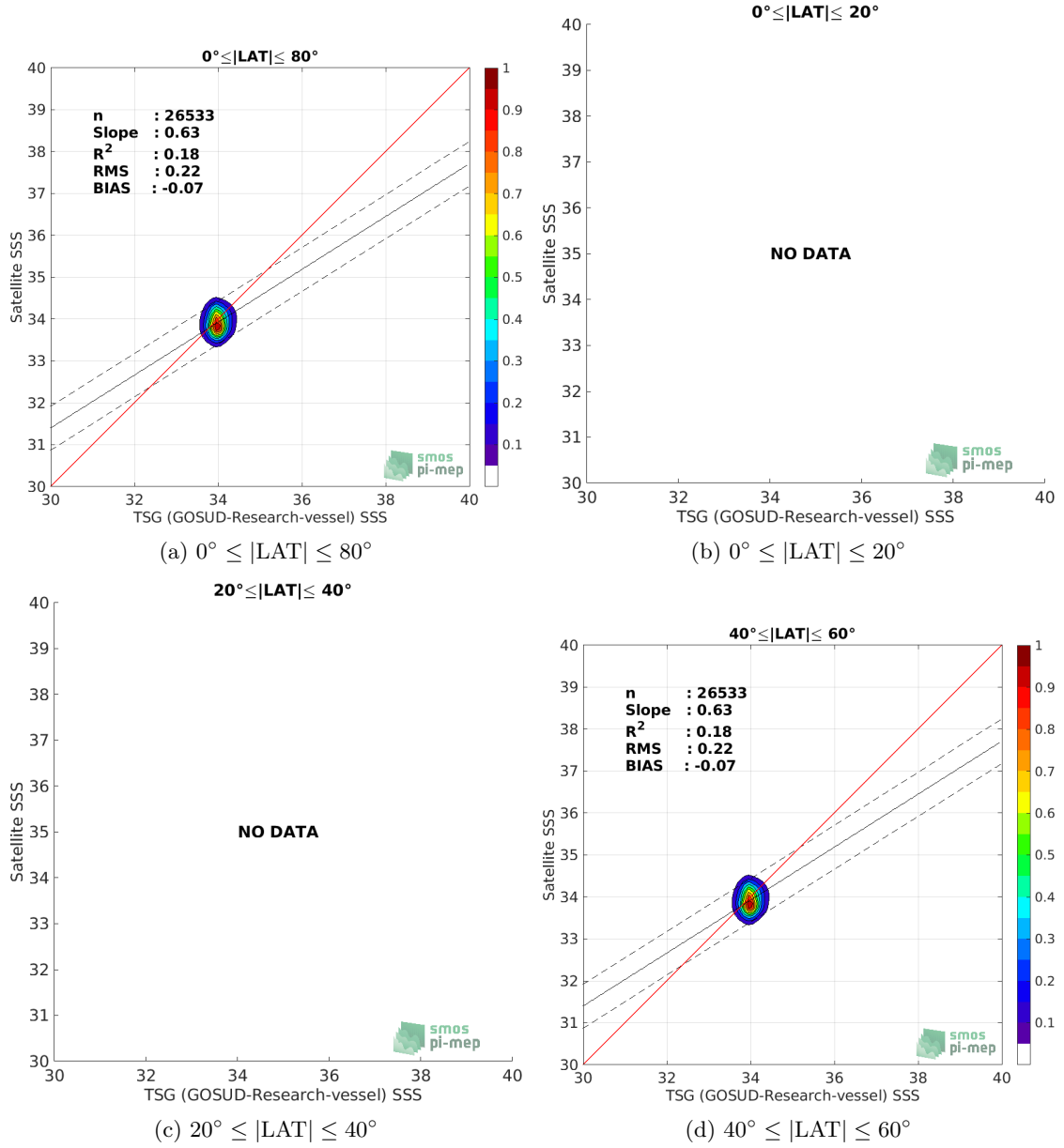
Figure 9: Contour maps of the concentration of SMOS SSS L3 v5 - 18 Days (CATDS-CECOS-LOCEAN) SSS (y-axis) versus TSG (GOSUD-Research-vessel) SSS (x-axis) at match-up pairs for different latitude bands. For each plot, the red line shows x=y . The black thin and dashed lines indicate a linear fit through the data cloud and the \pm 95\% confidence levels, respectively. The number match-up pairs n , the slope and R^2 coefficient of the linear fit, the root mean square (RMS) and the mean bias between satellite and in situ data are indicated for each latitude band in each plots.
