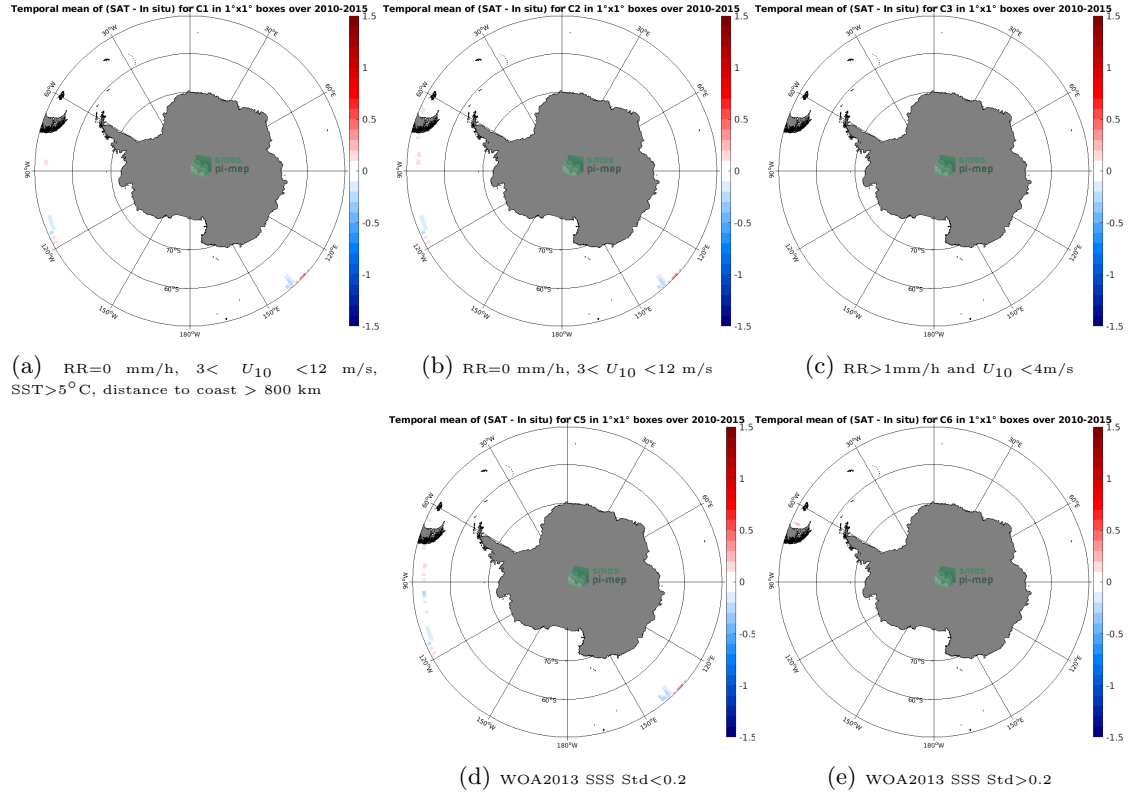
Figure 12: Temporal mean gridded over spatial boxes of size 1°x1° of \Delta\text{SSS} (SMOS SSS L3 v5 - 18 Days (CATDS-CECOS-LOCEAN) - TSG (GOSUD-Research-vessel)) for 5 different subdatasets corresponding to: RR=0 mm/h, 3 < U_{10} < 12 m/s, SST > 5^{\circ}\text{C} , distance to coast > 800 km (a), RR=0 mm/h, 3 < U_{10} < 12 m/s (b), RR > 1 mm/h and U_{10} < 4 m/s (c), WOA2013 SSS Std < 0.2 (d), WOA2013 SSS Std > 0.2 (e).
