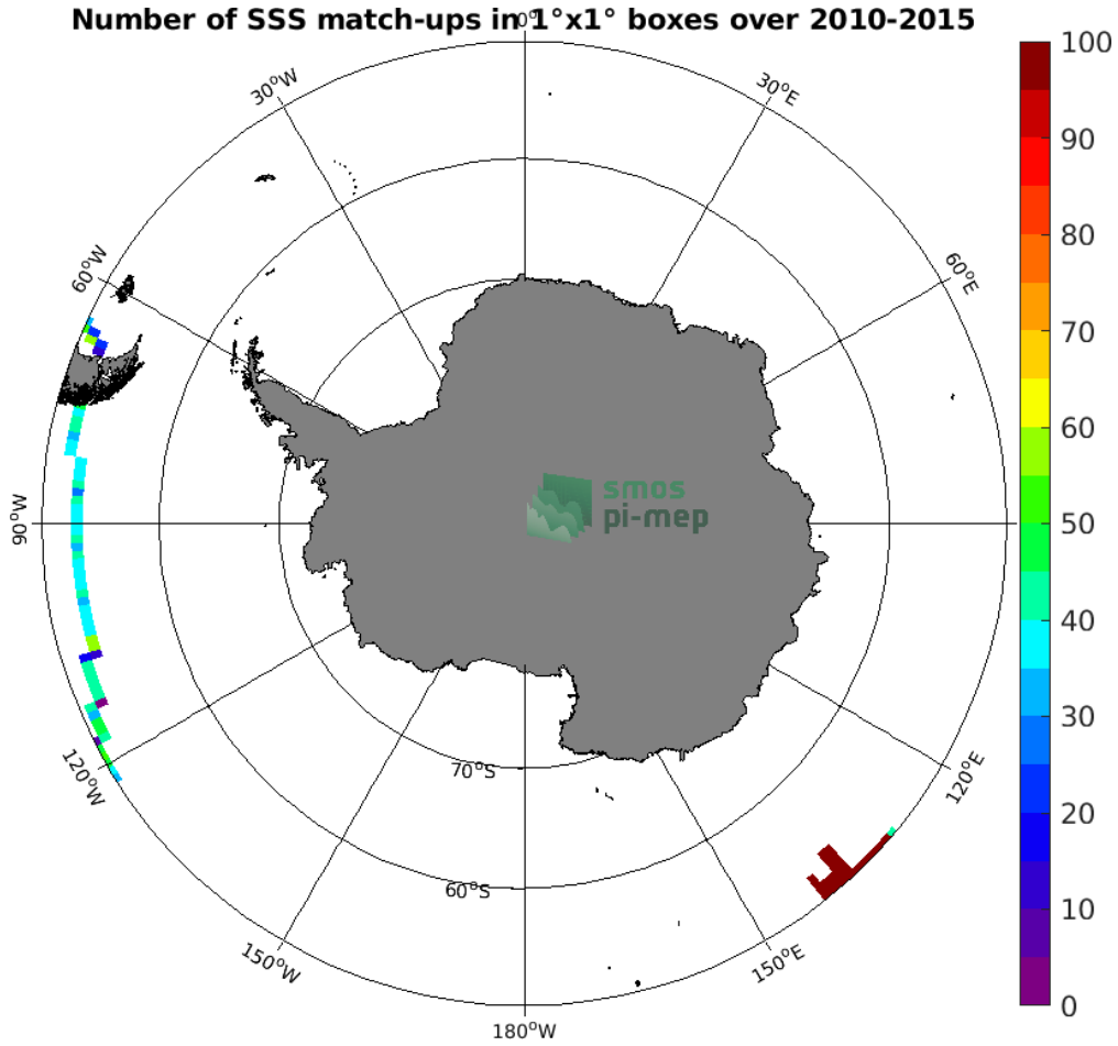
Figure 4: Number of SSS match-ups between TSG (GOSUD-Research-vessel) SSS and the SMOS SSS L3 v5 - 18 Days (CATDS-CECOS-LOCEAN) SSS product for the Southern Ocean Pi-MEP region over 1^\circ \times 1^\circ boxes and for the full satellite product period.
