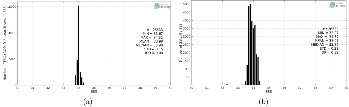
Figure 2: Histograms of SSS from TSG (GOSUD-Research-vessel) (a) and SMOS SSS L3 v5 - 18 Days (CATDS-CECOS-LOCEAN) (b) considering all match-up pairs per bins of 0.1 over the Southern Ocean Pi-MEP region and for the full satellite product period.
