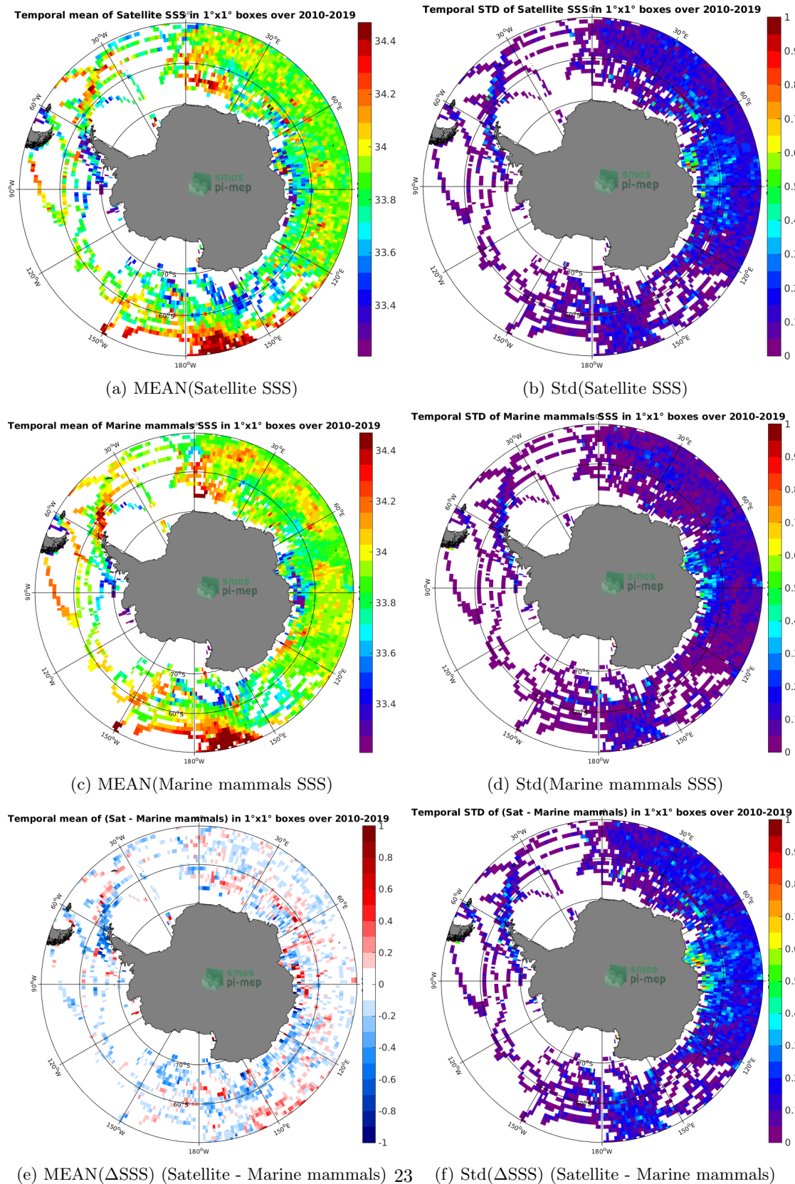
Figure 6: Temporal mean (left) and Std (right) of SSS from SMOS SSS L3 v5 - 18 Days (CATDS-CECOS-LOCEAN) (top), Marine mammals (middle), and of \Delta SSS (Satellite - Marine mammals). Only match-up pairs are used to generate these maps.
