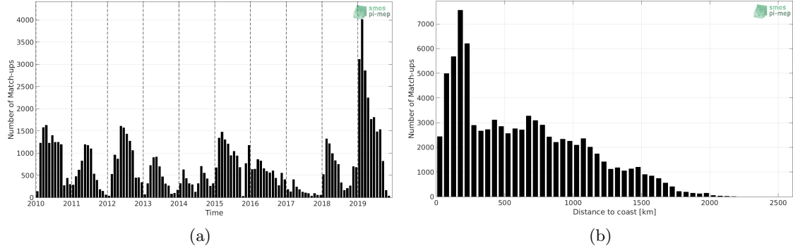
Figure 1: Number of match-ups between Marine mammals and SMOS SSS L3 v5 - 18 Days (CATDS-CECOS-LOCEAN) SSS as a function of time (a) and as function of the distance to coast (b) over the Southern Ocean Pi-MEP region and for the full satellite product period.
