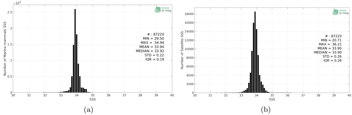
Figure 2: Histograms of SSS from Marine mammals (a) and SMOS SSS L3 v5 - 18 Days (CATDS-CECOS-LOCEAN) (b) considering all match-up pairs per bins of 0.1 over the Southern Ocean Pi-MEP region and for the full satellite product period.
