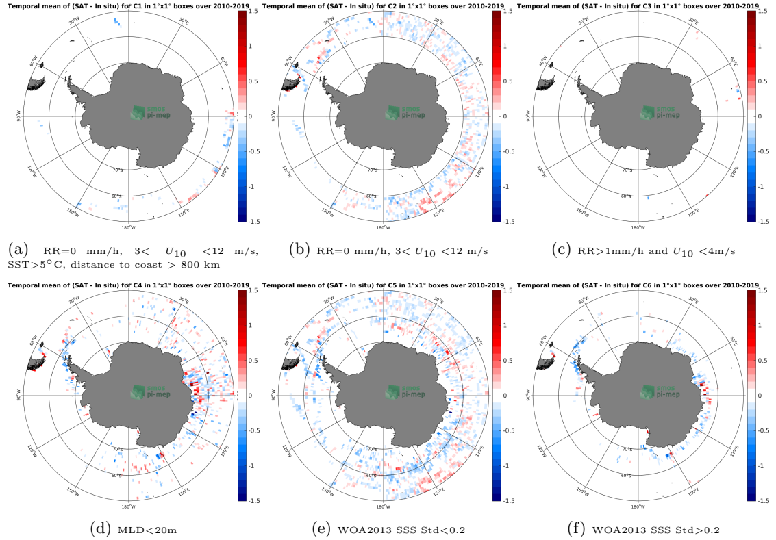
Figure 12: Temporal mean gridded over spatial boxes of size 1^{\circ} \times 1^{\circ} of \Delta\text{SSS} (SMOS SSS L3 v5 - 18 Days (CATDS-CECOS-LOCEAN) - Marine mammals) for 6 different subdatasets corresponding to:RR=0 mm/h, 3 < U_{10} < 12 m/s, SST >5^{\circ}\text{C} , distance to coast > 800 km (a), RR=0 mm/h, 3 < U_{10} < 12 m/s (b), RR >1 mm/h and U_{10} < 4 m/s (c),MLD <20 m (d),WOA2013 SSS Std <0.2 (e),WOA2013 SSS Std >0.2 (f).
