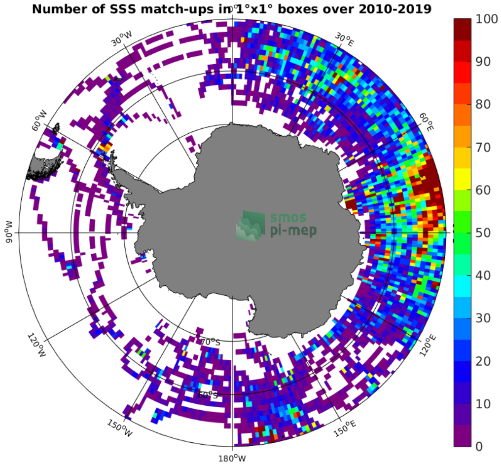
Figure 4: Number of SSS match-ups between Marine mammals SSS and the SMOS SSS L3 v5 - 18 Days (CATDS-CECOS-LOCEAN) SSS product for the Southern Ocean Pi-MEP region over 1^\circ \times 1^\circ boxes and for the full satellite product period.
