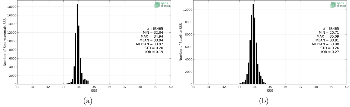
Figure 2: Histograms of SSS from Sea mammals (a) and SMOS SSS L3 v5 - 18 Days (CATDS-CECOS-LOCEAN) (b) considering all match-up pairs per bins of 0.1 over the Southern Ocean Pi-MEP region and for the full satellite product period.
