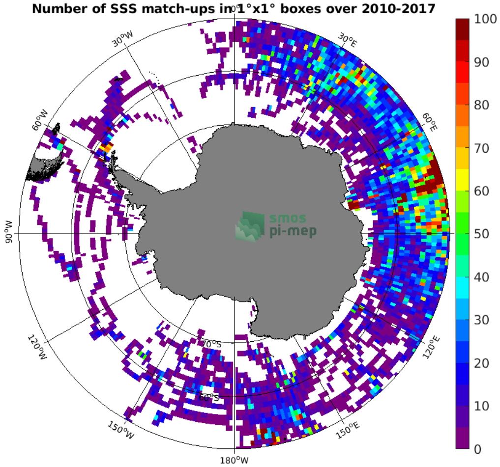
Figure 4: Number of SSS match-ups between Sea mammals SSS and the SMOS SSS L3 v5 - 18 Days (CATDS-CECOS-LOCEAN) SSS product for the Southern Ocean Pi-MEP region over 1^\circ \times 1^\circ boxes and for the full satellite product period.
