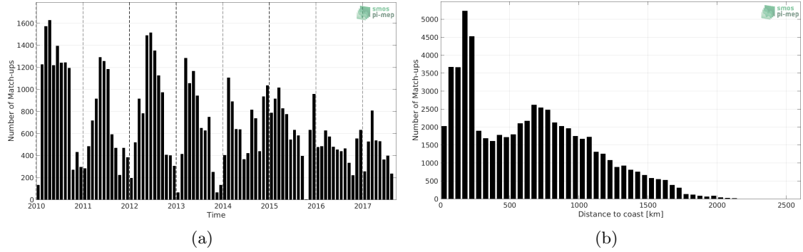
Figure 1: Number of match-ups between Sea mammals and SMOS SSS L3 v5 - 18 Days (CATDS-CECOS-LOCEAN) SSS as a function of time (a) and as function of the distance to coast (b) over the Southern Ocean Pi-MEP region and for the full satellite product period.
