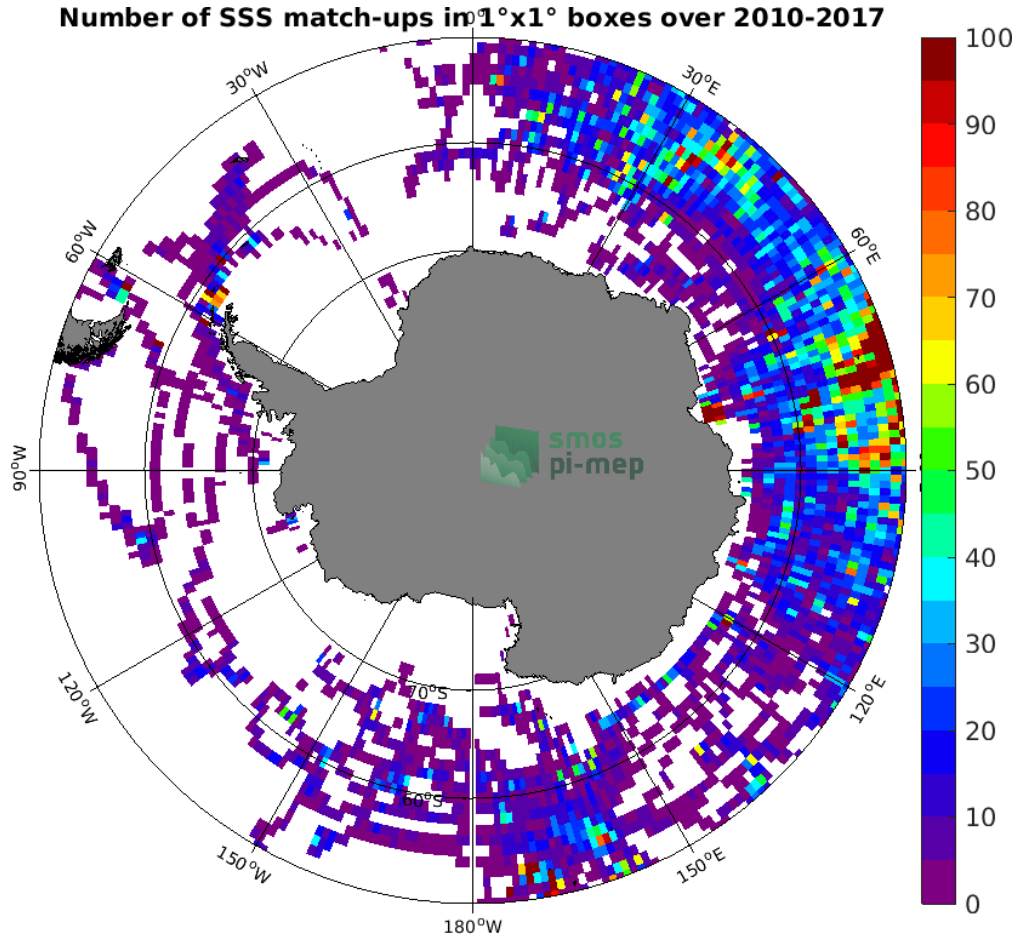
Figure 4: Number of SSS match-ups between Sea mammals SSS and the SMOS SSS L3 v5 - 18 Days (CATDS-CECOS-LOCEAN) SSS product for the Southern Ocean Pi-MEP region over 1^\circ \times 1^\circ boxes and for the full satellite product period.
