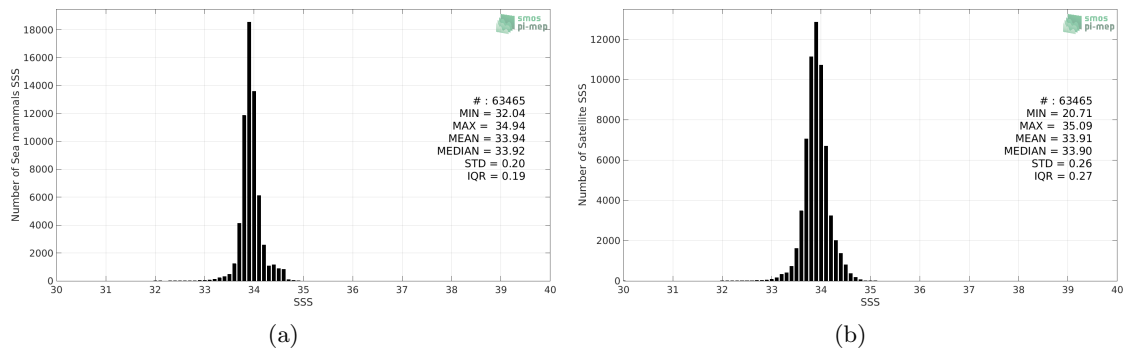
Figure 2: Histograms of SSS from Sea mammals (a) and SMOS SSS L3 v5 - 18 Days (CATDS-CECOS-LOCEAN) (b) considering all match-up pairs per bins of 0.1 over the Southern Ocean Pi-MEP region and for the full satellite product period.
