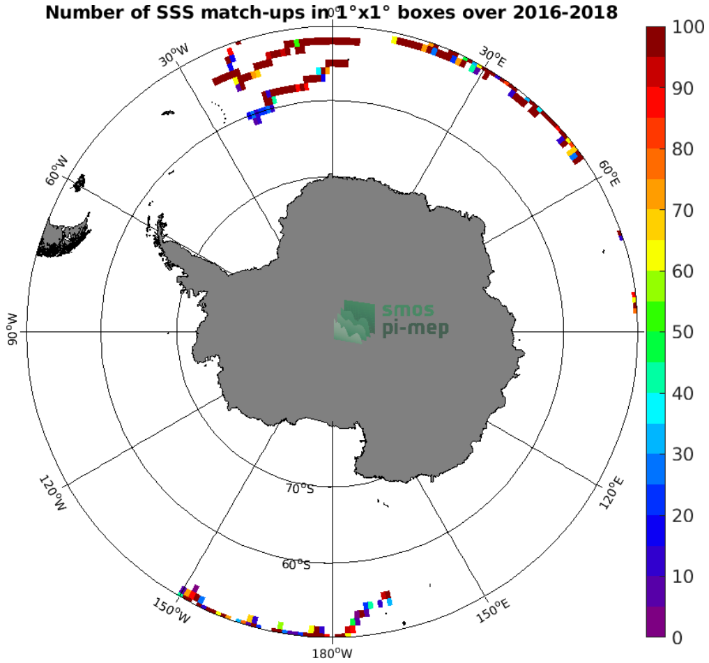
Figure 3: Number of SSS match-ups between Surface drifters SSS and the SMOS SSS L3 v5 - 18 Days (CATDS-CECOS-LOCEAN) SSS product for the Southern Ocean Pi-MEP region over 1^\circ \times 1^\circ boxes and for the full satellite product period.
