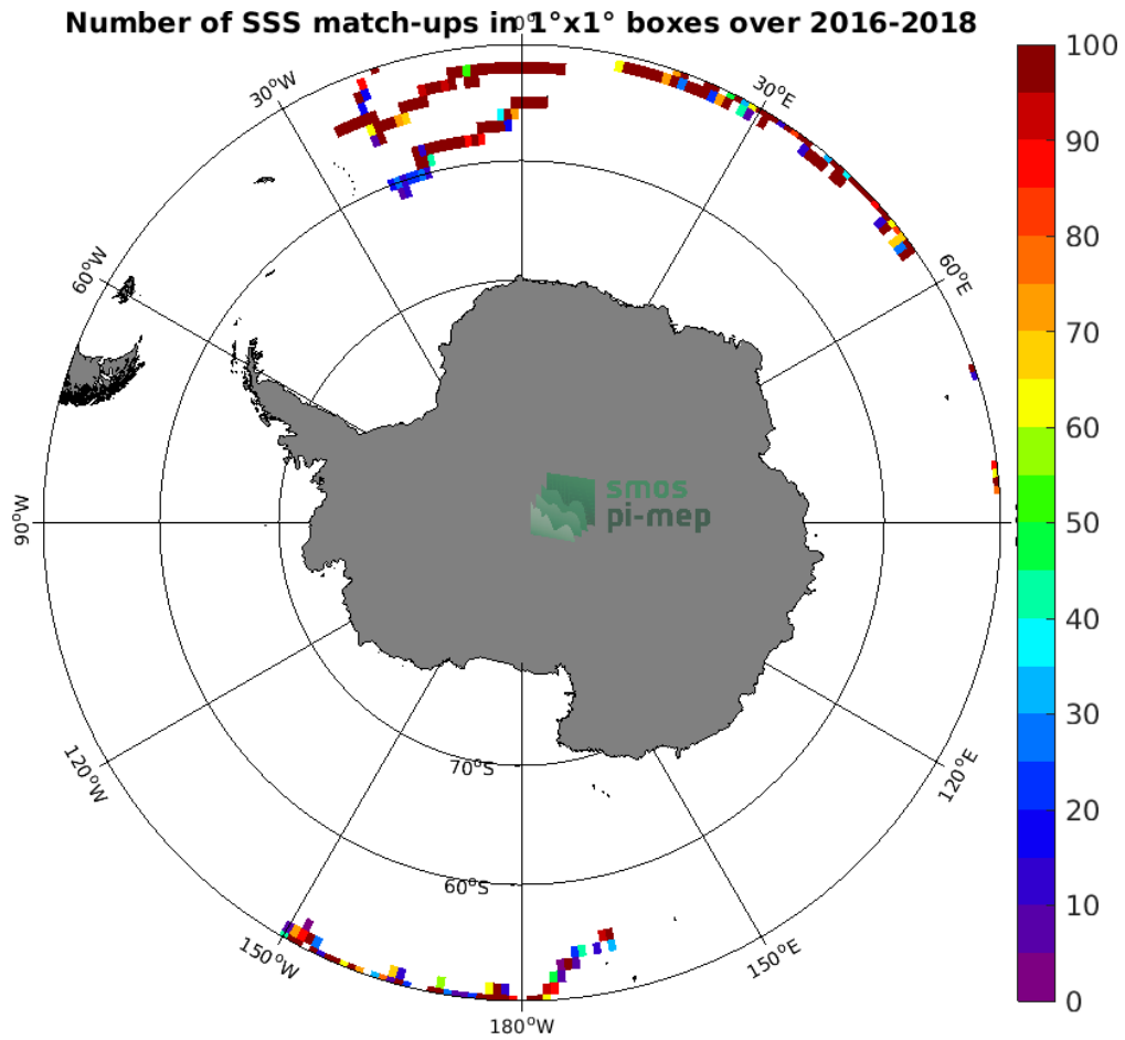
Figure 3: Number of SSS match-ups between Surface drifters SSS and the SMOS SSS L3 v5 - 18 Days (CATDS-CECOS-LOCEAN) SSS product for the Southern Ocean Pi-MEP region over 1^\circ \times 1^\circ boxes and for the full satellite product period.
