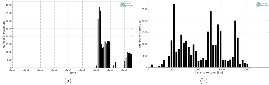
Figure 1: Number of match-ups between Surface drifters and SMOS SSS L3 v5 - 18 Days (CATDS-CECOS-LOCEAN) SSS as a function of time (a) and as function of the distance to coast (b) over the Southern Ocean Pi-MEP region and for the full satellite product period.
