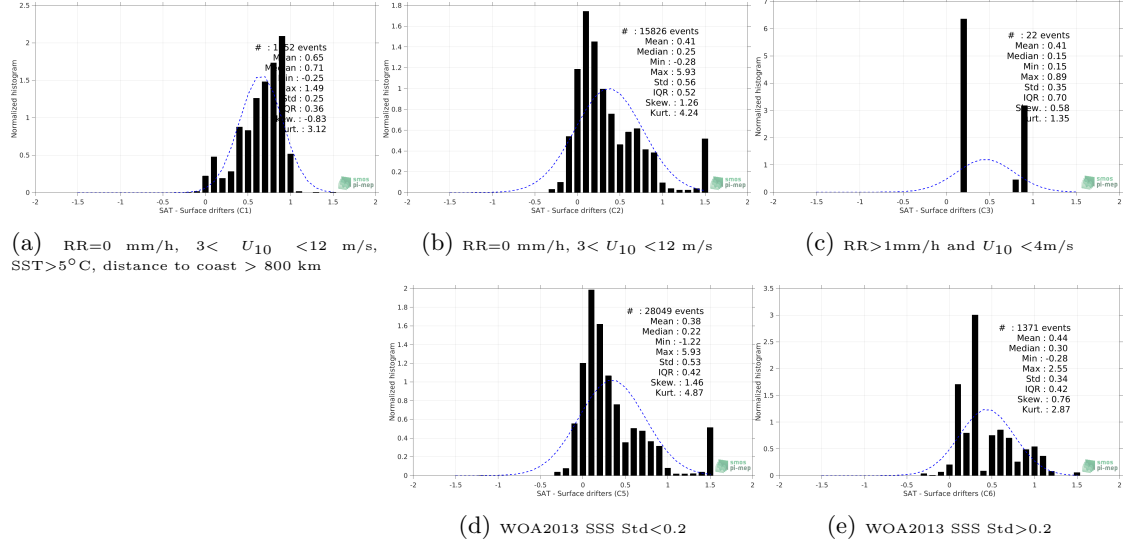
Figure 12: Normalized histogram of \Delta\text{SSS} (SMOS SSS L3 v5 - 18 Days (CATDS-CECOS-LOCEAN) - Surface drifters) for 5 different subdatasets corresponding to: RR=0 mm/h, 3 < U_{10} < 12 m/s, SST > 5^\circ\text{C} , distance to coast > 800 km (a), RR=0 mm/h, 3 < U_{10} < 12 m/s (b), RR > 1\text{mm/h} and U_{10} < 4\text{m/s} (c), WOA2013 SSS \text{Std} < 0.2 (d), WOA2013 SSS \text{Std} > 0.2 (e).
