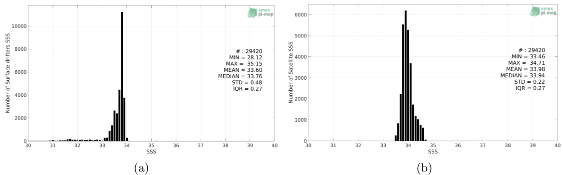
Figure 2: Histograms of SSS from Surface drifters (a) and SMOS SSS L3 v5 - 18 Days (CATDS-CECOS-LOCEAN) (b) considering all match-up pairs per bins of 0.1 over the Southern Ocean Pi-MEP region and for the full satellite product period.
