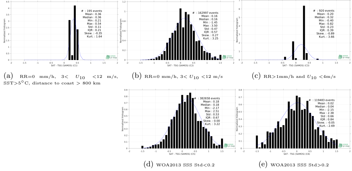
Figure 13: Normalized histogram of \Delta SSS (SMOS SSS L3 v4 - 9 Days (CATDS-CECOS-LOCEAN) - TSG (SAMOS)) for 5 different subdatasets corresponding to: RR=0 mm/h, 3 < U_{10} < 12 m/s, SST>5°C, distance to coast > 800 km (a), RR=0 mm/h, 3 < U_{10} < 12 m/s (b), RR>1mm/h and U_{10} < 4 m/s (c), WOA2013 SSS Std<0.2 (d), WOA2013 SSS Std>0.2 (e).
