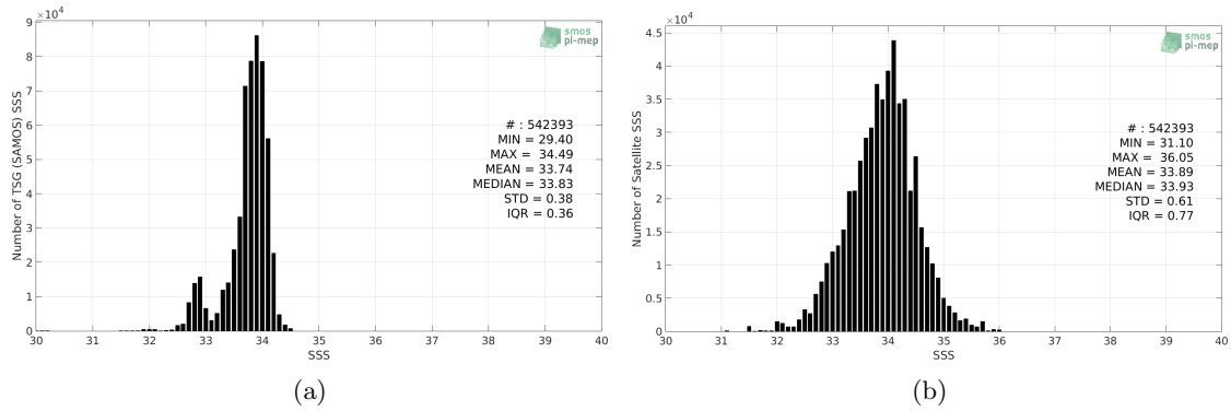
Figure 2: Histograms of SSS from TSG (SAMOS) (a) and SMOS SSS L3 v4 - 9 Days (CATDS-CECOS-LOCEAN) (b) considering all match-up pairs per bins of 0.1 over the Southern Ocean Pi-MEP region and for the full satellite product period.
