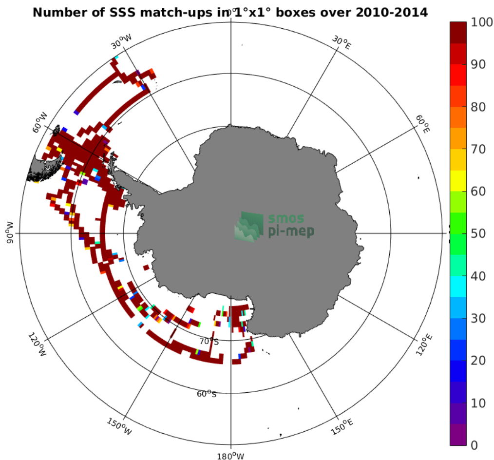
Figure 4: Number of SSS match-ups between TSG (SAMOS) SSS and the SMOS SSS L3 v4 - 9 Days (CATDS-CECOS-LOCEAN) SSS product for the Southern Ocean Pi-MEP region over 1^\circ \times 1^\circ boxes and for the full satellite product period.
