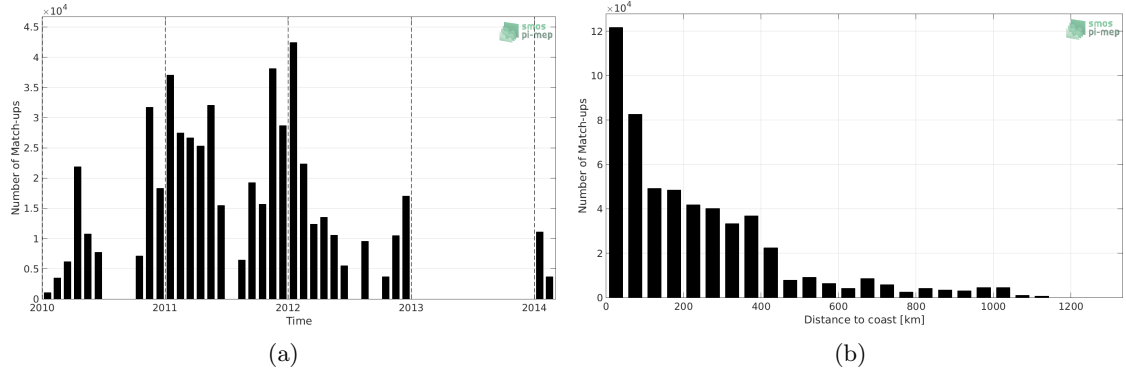
Figure 1: Number of match-ups between TSG (SAMOS) and SMOS SSS L3 v4 - 9 Days (CATDS-CECOS-LOCEAN) SSS as a function of time (a) and as function of the distance to coast (b) over the Southern Ocean Pi-MEP region and for the full satellite product period.
