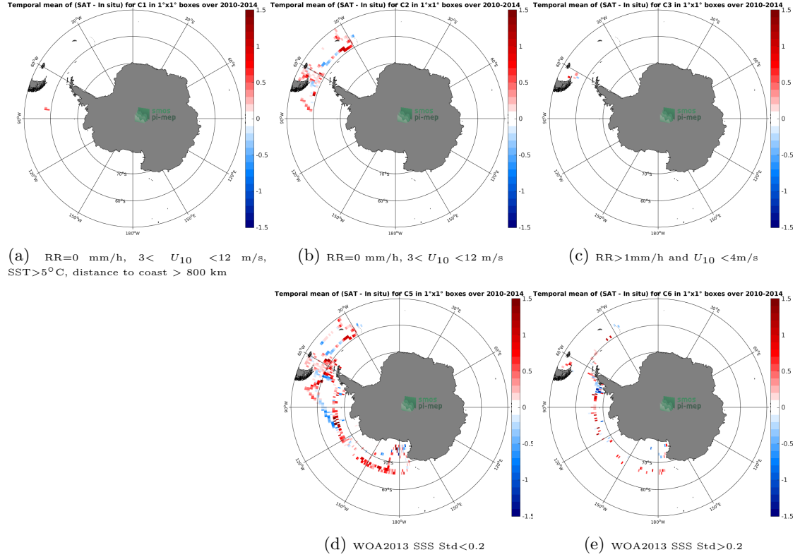
Figure 12: Temporal mean gridded over spatial boxes of size 1^{\circ}\times 1^{\circ} of \Delta\text{SSS} (SMOS SSS L3 v4 - 9 Days (CATDS-CECOS-LOCEAN) - TSG (SAMOS)) for 5 different subdatasets corresponding to: \text{RR}=0 mm/h, 3 < U_{10} < 12 m/s, \text{SST} > 5^{\circ}\text{C} , distance to coast > 800 km (a), \text{RR}=0 mm/h, 3 < U_{10} < 12 m/s (b), \text{RR} > 1 mm/h and U_{10} < 4 m/s (c), WOA2013 SSS Std < 0.2 (d), WOA2013 SSS Std > 0.2 (e).
