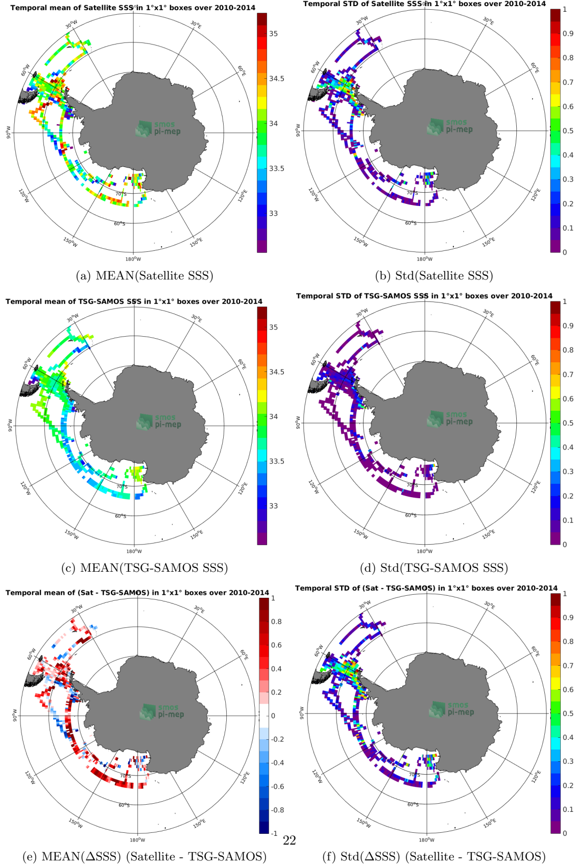
Figure 6: Temporal mean (left) and Std (right) of SSS from SMOS-L3-CATDS-CECOS-LOCEAN-V4-9DAYS-25KM (top), TSG-SAMOS (middle), and of \Delta SSS (Satellite - TSG-SAMOS). Only match-up pairs are used to generate these maps.
