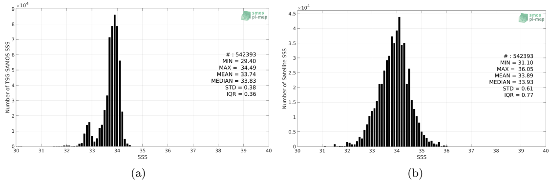
Figure 2: Histograms of SSS from TSG-SAMOS (a) and SMOS-L3-CATDS-CECOS-LOCEAN-V4-9DAYS-25KM (b) considering all match-up pairs per bins of 0.1 over the Southern Ocean Pi-MEP region and for the full satellite product period.
