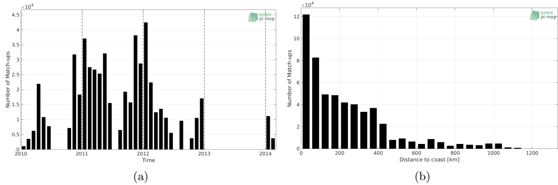
Figure 1: Number of match-ups between TSG-SAMOS and SMOS-L3-CATDS-CECOS-LOCEAN-V4-9DAYS-25KM SSS as a function of time (a) and as function of the distance to coast (b) over the Southern Ocean Pi-MEP region and for the full satellite product period.
