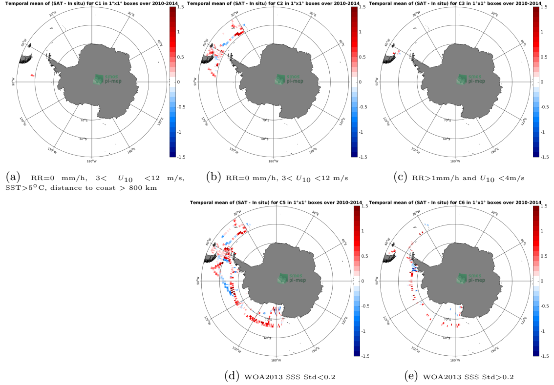
Figure 12: Temporal mean gridded over spatial boxes of size 1^{\circ}\times 1^{\circ} of \Delta\text{SSS} (SMOS-L3-CATDS-CECOS-LOCEAN-V4-9DAYS-25KM - TSG-SAMOS) for 5 different subdatasets corresponding to: \text{RR}=0 mm/h, 3 < U_{10} < 12 m/s, \text{SST}>5^{\circ}\text{C} , distance to coast > 800 km (a), \text{RR}=0 mm/h, 3 < U_{10} < 12 m/s (b), \text{RR}>1 mm/h and U_{10} < 4 m/s (c), WOA2013 SSS Std <0.2 (d), WOA2013 SSS Std >0.2 (e).
