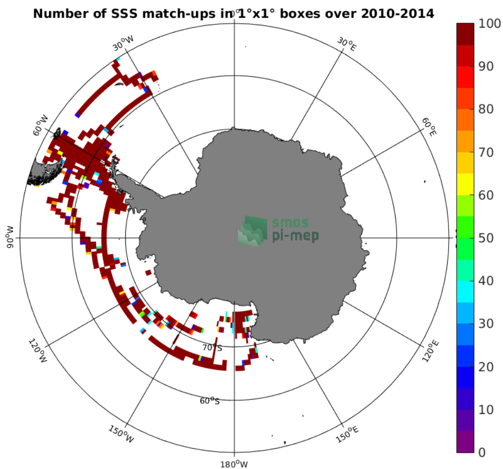
Figure 4: Number of SSS match-ups between TSG-SAMOS SSS and the SMOS-L3-CATDS-CECOS-LOCEAN-V4-9DAYS-25KM SSS product for the Southern Ocean Pi-MEP region over 1^\circ \times 1^\circ boxes and for the full satellite product period.
