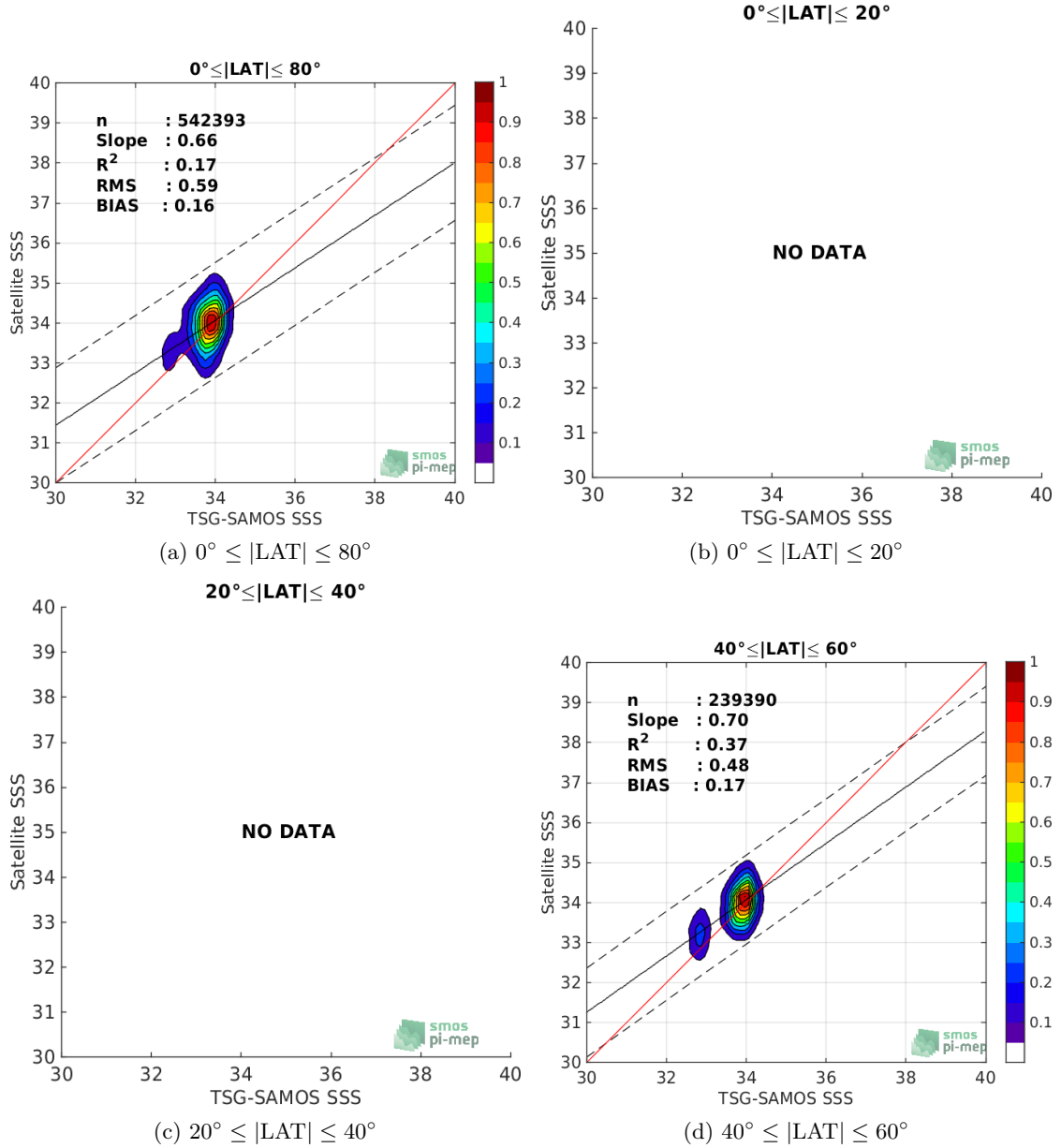
Figure 9: Contour maps of the concentration of SMOS-L3-CATDS-CECOS-LOCEAN-V4-9DAYS-25KM SSS (y-axis) versus TSG-SAMOS SSS (x-axis) at match-up pairs for different latitude bands. For each plot, the red line shows x=y . The black thin and dashed lines indicate a linear fit through the data cloud and the \pm 95\% confidence levels, respectively. The number match-up pairs n , the slope and R^2 coefficient of the linear fit, the root mean square (RMS) and the mean bias between satellite and in situ data are indicated for each latitude band in each plots.
