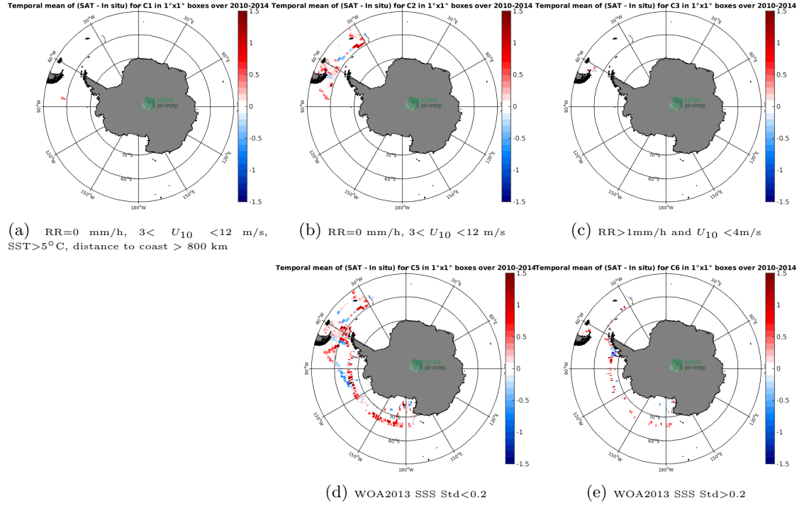
Figure 12: Temporal mean gridded over spatial boxes of size 1^\circ \times 1^\circ of \Delta SSS (SMOS-L3-CATDS-CECOS-LOCEAN-V4-9DAYS-25KM - TSG-SAMOS) for 5 different subdatasets corresponding to: RR=0 mm/h, 3 < U_{10} < 12 m/s, SST > 5^\circ\text{C} , distance to coast > 800 km (a), RR=0 mm/h, 3 < U_{10} < 12 m/s (b), RR > 1 mm/h and U_{10} < 4 m/s (c), WOA2013 SSS Std < 0.2 (d), WOA2013 SSS Std > 0.2 (e).
