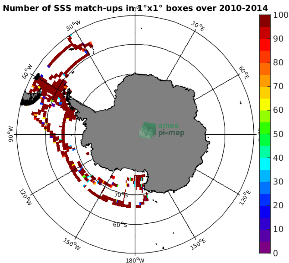
Figure 4: Number of SSS match-ups between TSG-SAMOS SSS and the SMOS-L3-CATDS-CECOS-LOCEAN-V4-9DAYS-25KM SSS product for the Southern Ocean Pi-MEP region over 1^\circ \times 1^\circ boxes and for the full satellite product period.
