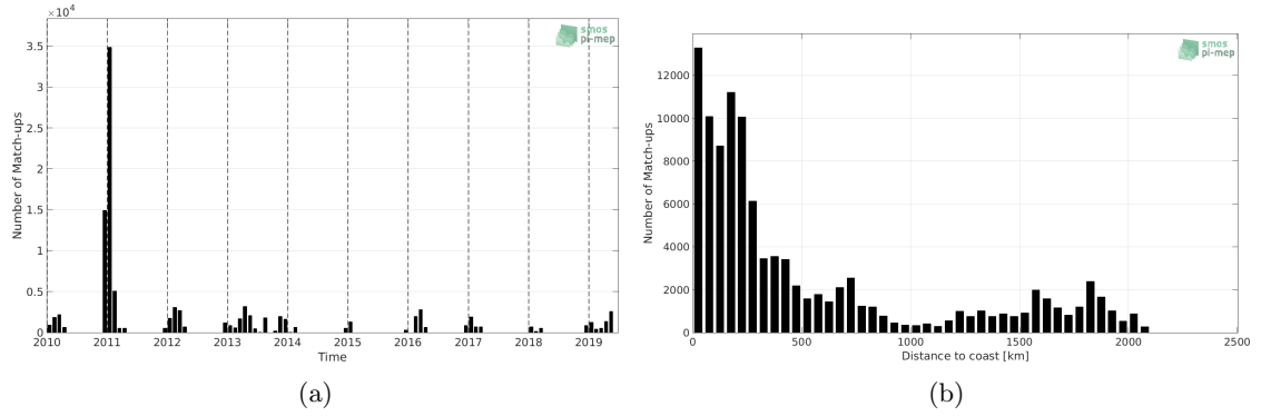
Figure 1: Number of match-ups between TSG (Polarstern) and SMOS SSS L3 v4 - 9 Days (CATDS-CECOS-LOCEAN) SSS as a function of time (a) and as function of the distance to coast (b) over the Southern Ocean Pi-MEP region and for the full satellite product period.
