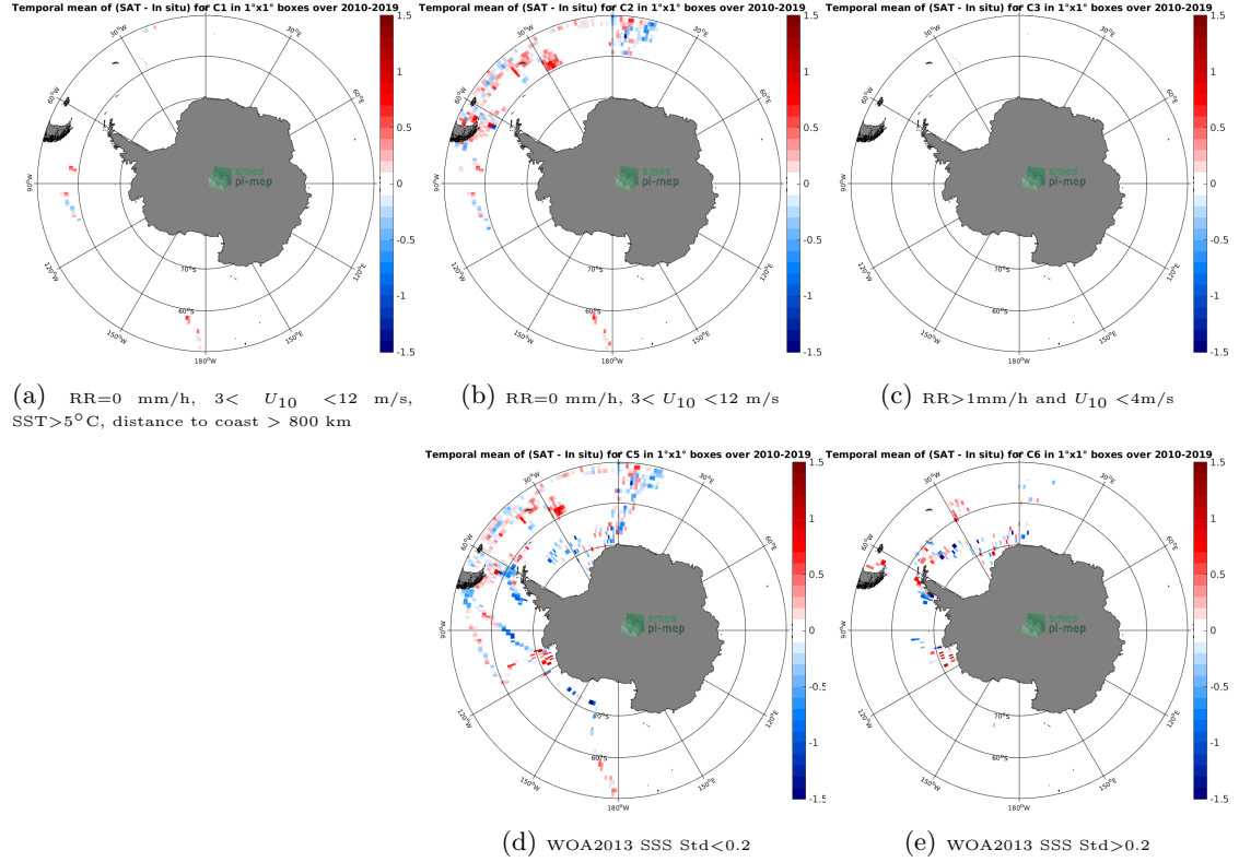
Figure 12: Temporal mean gridded over spatial boxes of size 1^{\circ}\times 1^{\circ} of \Delta\text{SSS} (SMOS SSS L3 v4 - 9 Days (CATDS-CECOS-LOCEAN) - TSG (Polarstern)) for 5 different subdatasets corresponding to: RR=0 mm/h, 3 < U_{10} < 12 m/s, SST > 5^{\circ}\text{C} , distance to coast > 800 km (a), RR=0 mm/h, 3 < U_{10} < 12 m/s (b), RR > 1 mm/h and U_{10} < 4 m/s (c), WOA2013 SSS Std < 0.2 (d), WOA2013 SSS Std > 0.2 (e).
