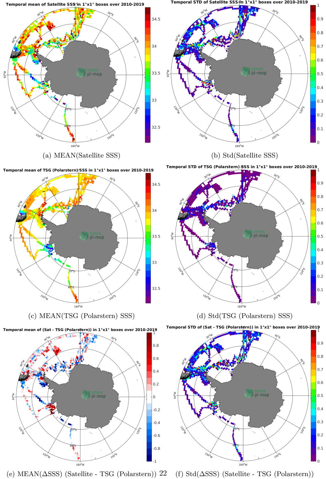
Figure 6: Temporal mean (left) and Std (right) of SSS from SMOS SSS L3 v4 - 9 Days (CATDS-CECOS-LOCEAN) (top), TSG (Polarstern) (middle), and of \Delta SSS (Satellite - TSG (Polarstern)). Only match-up pairs are used to generate these maps.
