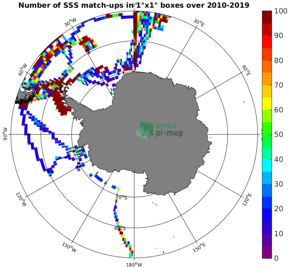
Figure 4: Number of SSS match-ups between TSG (Polarstern) SSS and the SMOS SSS L3 v4 - 9 Days (CATDS-CECOS-LOCEAN) SSS product for the Southern Ocean Pi-MEP region over 1^\circ \times 1^\circ boxes and for the full satellite product period.
