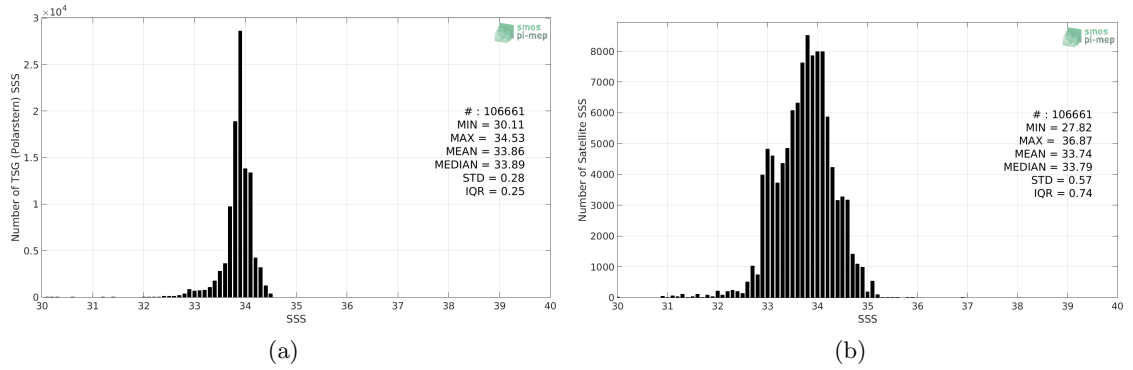
Figure 2: Histograms of SSS from TSG (Polarstern) (a) and SMOS SSS L3 v4 - 9 Days (CATDS-CECOS-LOCEAN) (b) considering all match-up pairs per bins of 0.1 over the Southern Ocean Pi-MEP region and for the full satellite product period.
