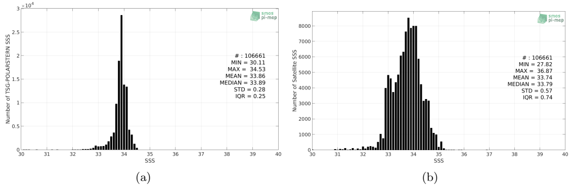
Figure 2: Histograms of SSS from TSG-POLARSTERN (a) and SMOS-L3-CATDS-CECOS-LOCEAN-V4-9DAYS-25KM (b) considering all match-up pairs per bins of 0.1 over the Southern Ocean Pi-MEP region and for the full satellite product period.
