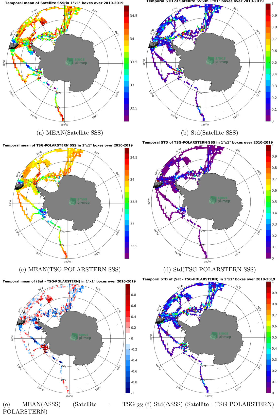
Figure 6: Temporal mean (left) and Std (right) of SSS from SMOS-L3-CATDS-CECOS-LOCEAN-V4-9DAYS-25KM (top), TSG-POLARSTERN (middle), and of \Delta SSS (Satellite - TSG-POLARSTERN). Only match-up pairs are used to generate these maps.
