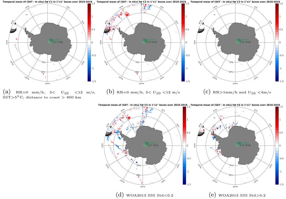
Figure 12: Temporal mean gridded over spatial boxes of size 1^{\circ}\times 1^{\circ} of \Delta\text{SSS} (SMOS-L3-CATDS-CECOS-LOCEAN-V4-9DAYS-25KM - TSG-POLARSTERN) for 5 different subdatasets corresponding to:RR=0 mm/h, 3 < U_{10} < 12 m/s, SST >5^{\circ}\text{C} , distance to coast > 800 km (a), RR=0 mm/h, 3 < U_{10} < 12 m/s (b), RR >1 mm/h and U_{10} < 4 m/s (c), WOA2013 SSS Std <0.2 (d), WOA2013 SSS Std >0.2 (e).
