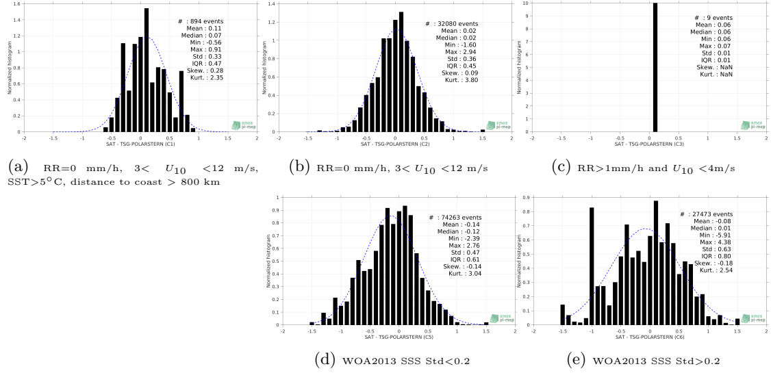
Figure 13: Normalized histogram of \Delta SSS (SMOS-L3-CATDS-CECOS-LOCEAN-V4-9DAYS-25KM - TSG-POLARSTERN) for 5 different subdatasets corresponding to: RR=0 mm/h, 3 < U_{10} < 12 m/s, SST > 5°C, distance to coast > 800 km (a), RR=0 mm/h, 3 < U_{10} < 12 m/s (b), RR > 1mm/h and U_{10} < 4 m/s (c), WOA2013 SSS Std < 0.2 (d), WOA2013 SSS Std > 0.2 (e).
