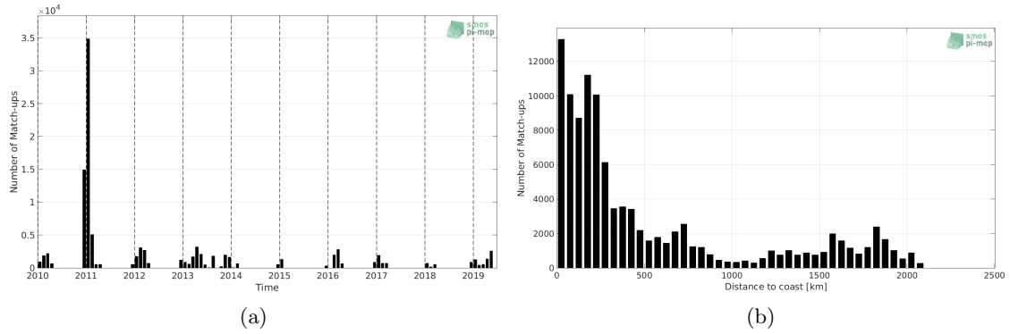
Figure 1: Number of match-ups between TSG-POLARSTERN and SMOS-L3-CATDS-CECOS-LOCEAN-V4-9DAYS-25KM SSS as a function of time (a) and as function of the distance to coast (b) over the Southern Ocean Pi-MEP region and for the full satellite product period.
