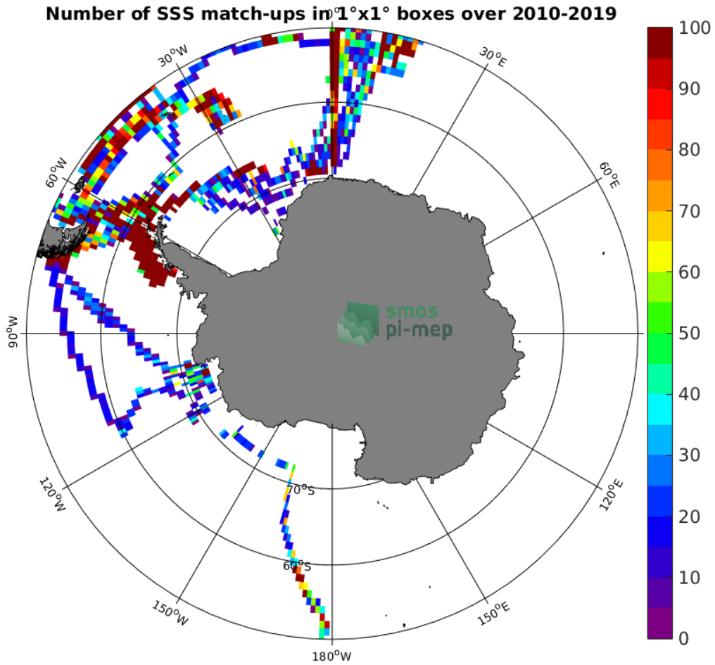
Figure 4: Number of SSS match-ups between TSG-POLARSTERN SSS and the SMOS-L3-CATDS-CECOS-LOCEAN-V4-9DAYS-25KM SSS product for the Southern Ocean Pi-MEP region over 1^\circ \times 1^\circ boxes and for the full satellite product period.
