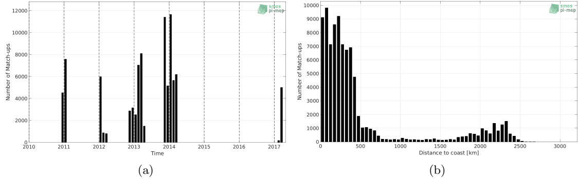
Figure 1: Number of match-ups between TSG (GOSUD-Sailing-ship) and SMOS SSS L3 v4 - 9 Days (CATDS-CECOS-LOCEAN) SSS as a function of time (a) and as function of the distance to coast (b) over the Southern Ocean Pi-MEP region and for the full satellite product period.
