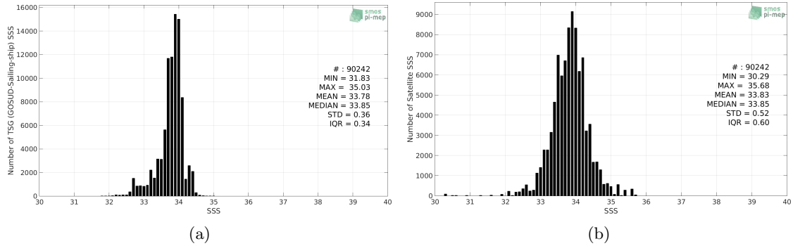
Figure 2: Histograms of SSS from TSG (GOSUD-Sailing-ship) (a) and SMOS SSS L3 v4 - 9 Days (CATDS-CECOS-LOCEAN) (b) considering all match-up pairs per bins of 0.1 over the Southern Ocean Pi-MEP region and for the full satellite product period.
