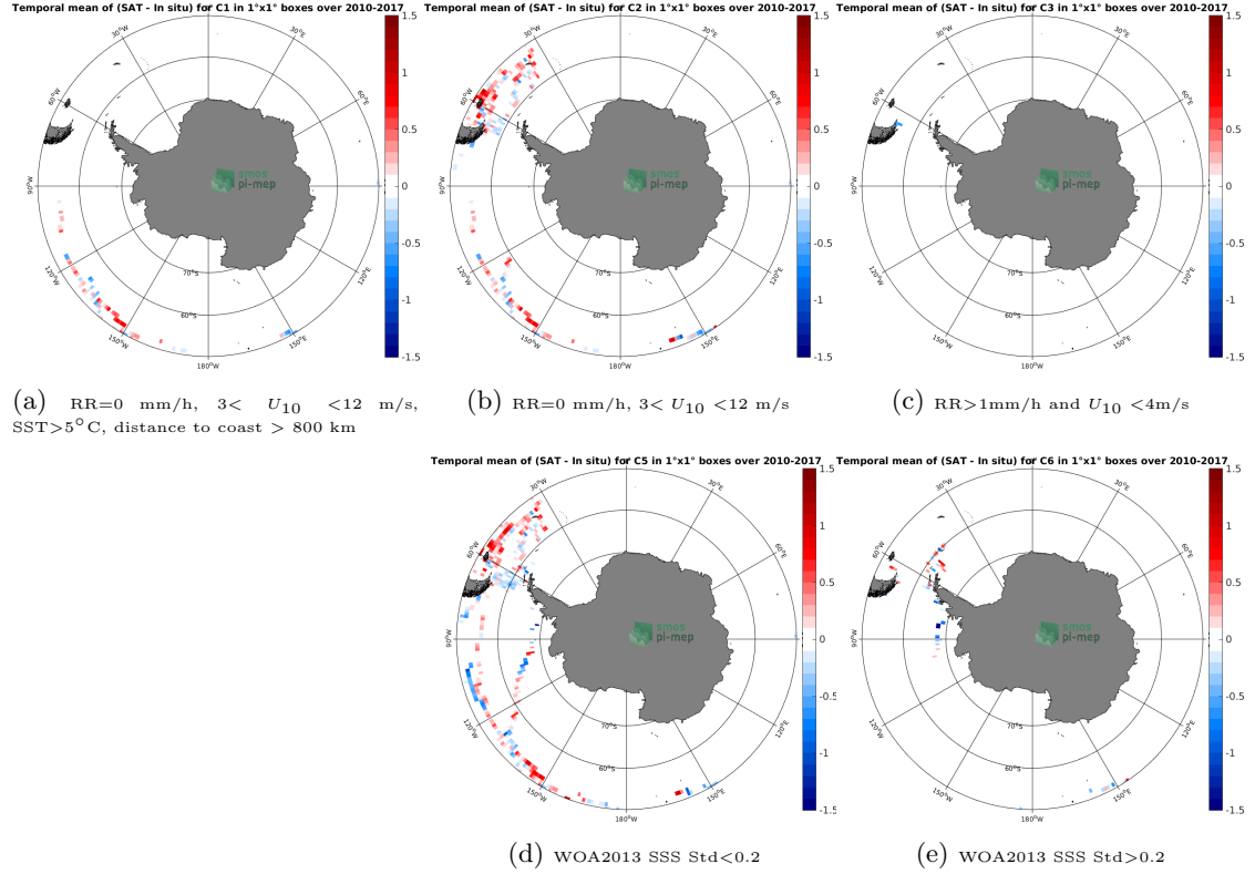
Figure 12: Temporal mean gridded over spatial boxes of size 1°x1° of \Delta SSS (SMOS SSS L3 v4 - 9 Days (CATDS-CECOS-LOCEAN) - TSG (GOSUD-Sailing-ship)) for 5 different subdatasets corresponding to: RR=0 mm/h, 3 < U_{10} < 12 m/s, SST>5°C, distance to coast > 800 km (a), RR=0 mm/h, 3 < U_{10} < 12 m/s (b), RR>1mm/h and U_{10} < 4 m/s (c), WOA2013 SSS Std<0.2 (d), WOA2013 SSS Std>0.2 (e).
