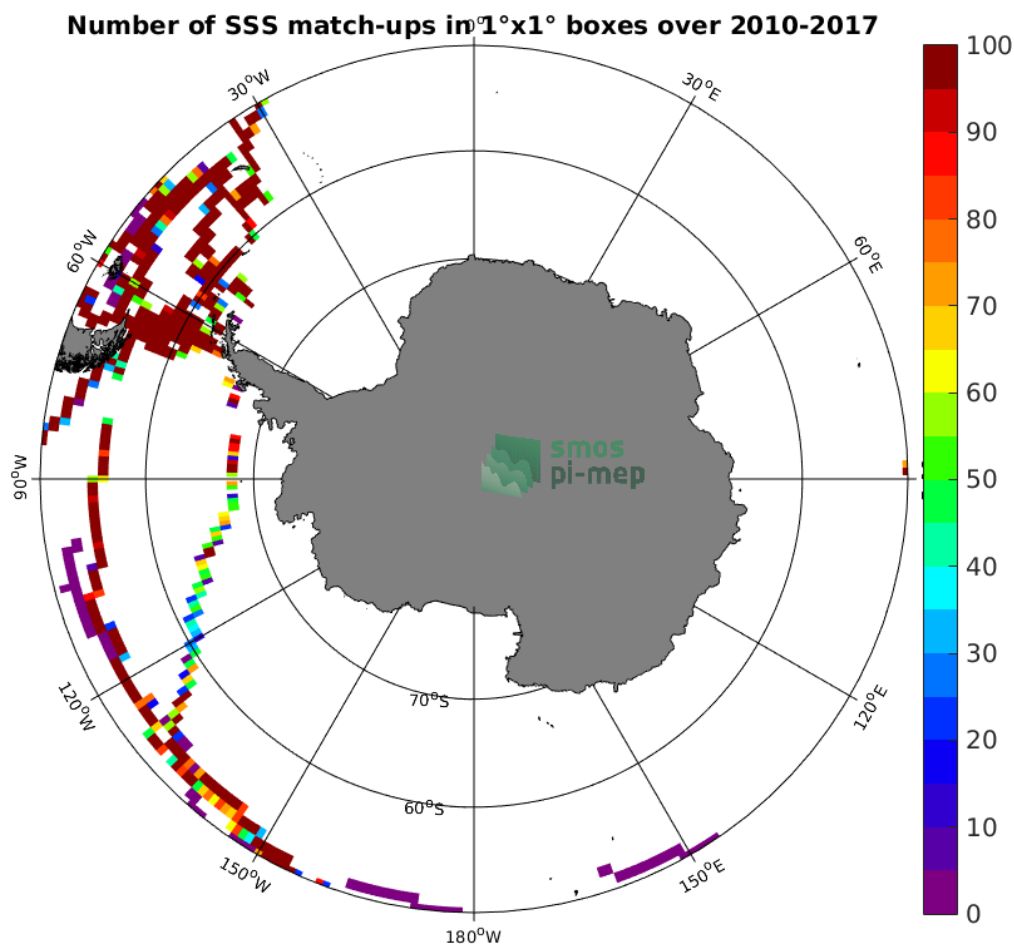
Figure 4: Number of SSS match-ups between TSG (GOSUD-Sailing-ship) SSS and the SMOS SSS L3 v4 - 9 Days (CATDS-CECOS-LOCEAN) SSS product for the Southern Ocean Pi-MEP region over 1^\circ \times 1^\circ boxes and for the full satellite product period.
