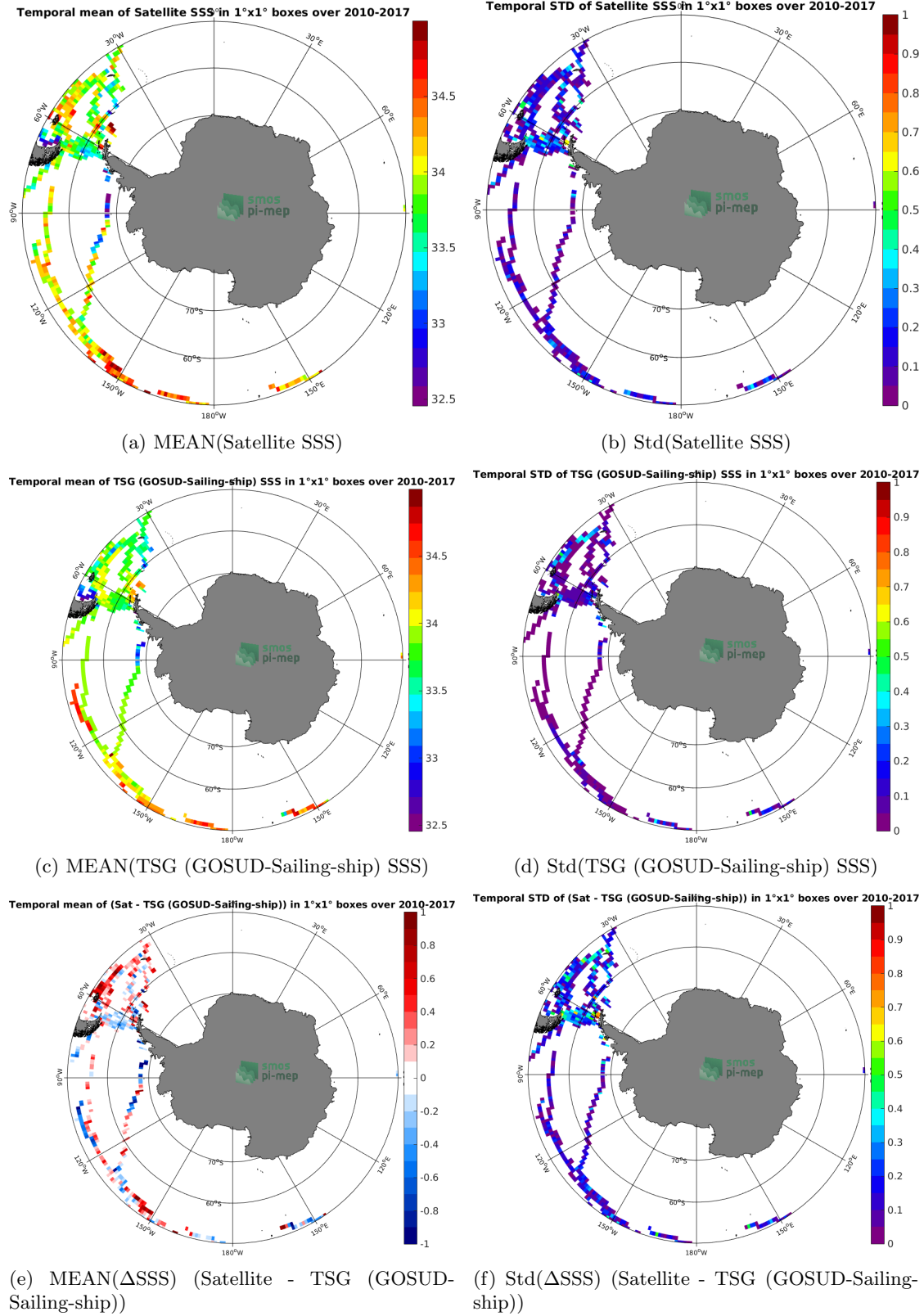
Figure 6: Temporal mean (left) and Std (right) of SSS from SMOS SSS L3 v4 - 9 Days (CATDS-CECOS-LOCEAN) (top), TSG (GOSUD-Sailing-ship) (middle), and of \Delta SSS (Satellite - TSG (GOSUD-Sailing-ship)). Only match-up pairs are used to generate these maps.
