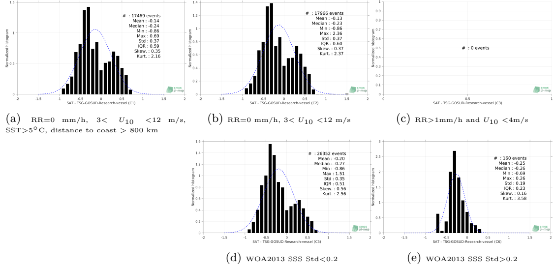
Figure 13: Normalized histogram of \Delta\text{SSS} (SMOS-L3-CATDS-CECOS-LOCEAN-V4-9DAYS-25KM - TSG-GOSUD-Research-vessel) for 5 different subdatasets corresponding to: RR=0 mm/h, 3 < U_{10} < 12 m/s, SST > 5^\circ\text{C} , distance to coast > 800 km (a), RR=0 mm/h, 3 < U_{10} < 12 m/s (b), RR > 1\text{mm/h} and U_{10} < 4\text{m/s} (c), WOA2013 SSS Std < 0.2 (d), WOA2013 SSS Std > 0.2 (e).
