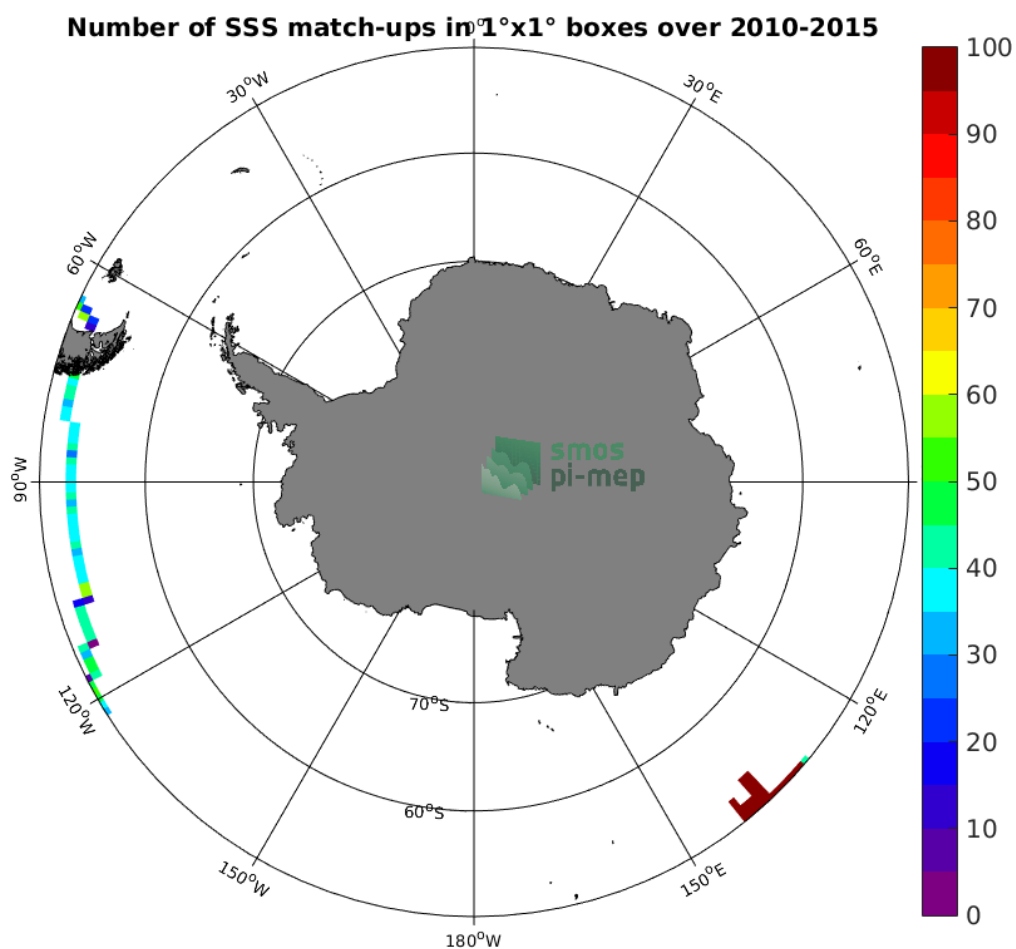
Figure 4: Number of SSS match-ups between TSG-GOSUD-Research-vessel SSS and the SMOS-L3-CATDS-CECOS-LOCEAN-V4-9DAYS-25KM SSS product for the Southern Ocean Pi-MEP region over 1^\circ \times 1^\circ boxes and for the full satellite product period.
