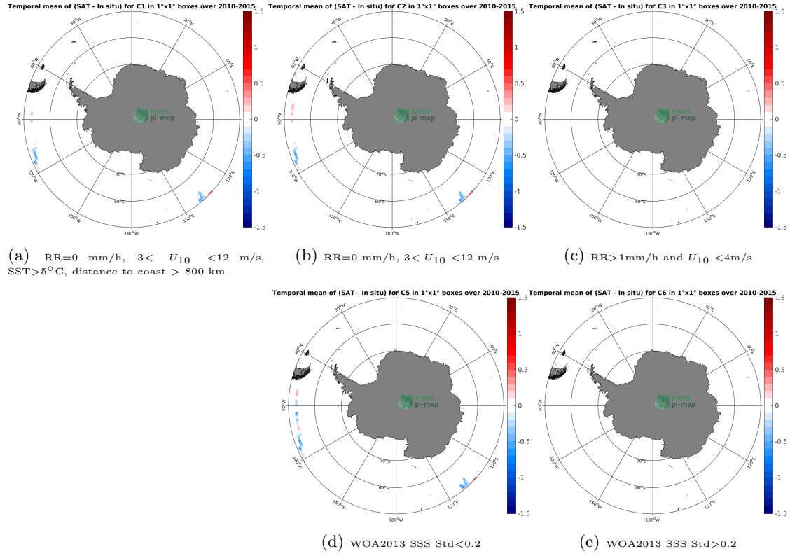
Figure 12: Temporal mean gridded over spatial boxes of size 1°x1° of \Delta\text{SSS} (SMOS-L3-CATDS-CECOS-LOCEAN-V4-9DAYS-25KM - TSG-GOSUD-Research-vessel) for 5 different subdatasets corresponding to: RR=0 mm/h, 3 < U_{10} < 12 m/s, SST > 5^\circ\text{C} , distance to coast > 800 km (a), RR=0 mm/h, 3 < U_{10} < 12 m/s (b), RR > 1 mm/h and U_{10} < 4 m/s (c), WOA2013 SSS Std < 0.2 (d), WOA2013 SSS Std > 0.2 (e).
