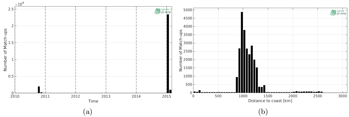
Figure 1: Number of match-ups between TSG-GOSUD-Research-vessel and SMOS-L3-CATDS-CECOS-LOCEAN-V4-9DAYS-25KM SSS as a function of time (a) and as function of the distance to coast (b) over the Southern Ocean Pi-MEP region and for the full satellite product period.
