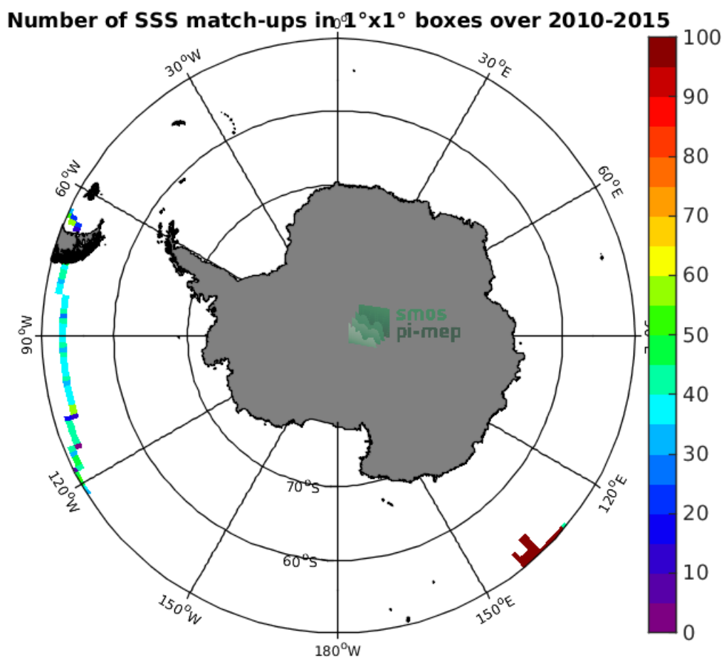
Figure 4: Number of SSS match-ups between TSG-GOSUD-Research-vessel SSS and the SMOS-L3-CATDS-CECOS-LOCEAN-V4-9DAYS-25KM SSS product for the Southern Ocean Pi-MEP region over 1^\circ \times 1^\circ boxes and for the full satellite product period.
