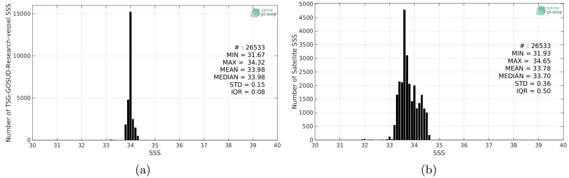
Figure 2: Histograms of SSS from TSG-GOSUD-Research-vessel (a) and SMOS-L3-CATDS-CECOS-LOCEAN-V4-9DAYS-25KM (b) considering all match-up pairs per bins of 0.1 over the Southern Ocean Pi-MEP region and for the full satellite product period.
