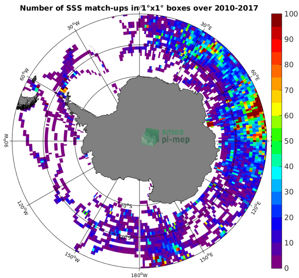
Figure 4: Number of SSS match-ups between Sea mammals SSS and the SMOS-L3-CATDS-CECOS-LOCEAN-V4-9DAYS-25KM SSS product for the Southern Ocean Pi-MEP region over 1^\circ \times 1^\circ boxes and for the full satellite product period.
