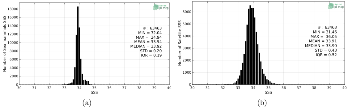
Figure 2: Histograms of SSS from Sea mammals (a) and SMOS-L3-CATDS-CECOS-LOCEAN-V4-9DAYS-25KM (b) considering all match-up pairs per bins of 0.1 over the Southern Ocean Pi-MEP region and for the full satellite product period.
