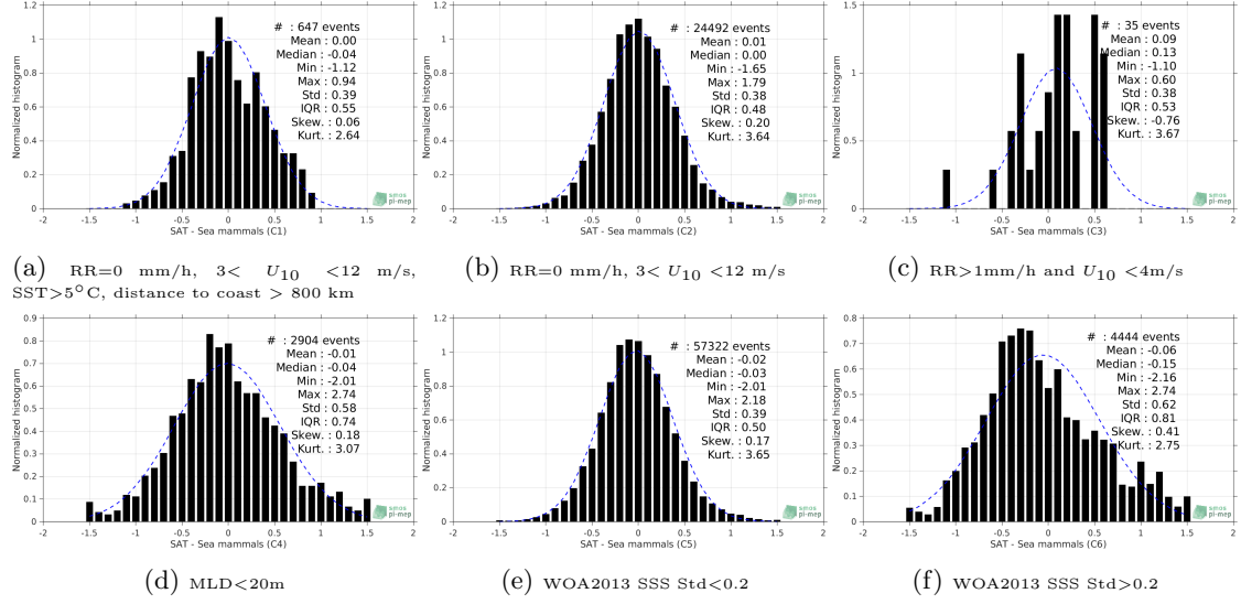
Figure 13: Normalized histogram of \Delta SSS (SMOS-L3-CATDS-CECOS-LOCEAN-V4-9DAYS-25KM - Sea mammals) for 6 different subdatasets corresponding to: RR=0 mm/h, 3 < U_{10} < 12 m/s, SST>5°C, distance to coast > 800 km (a), RR=0 mm/h, 3 < U_{10} < 12 m/s (b), RR>1mm/h and U_{10} < 4 m/s (c), MLD<20m (d), WOA2013 SSS Std<0.2 (e), WOA2013 SSS Std>0.2 (f).
