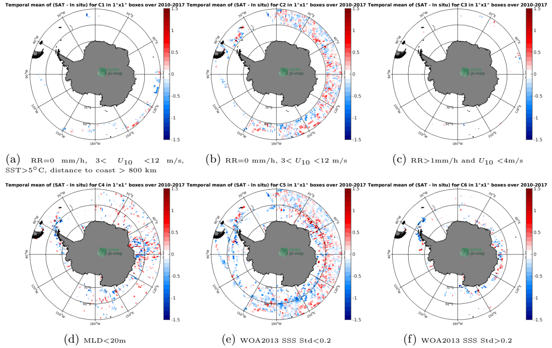
Figure 12: Temporal mean gridded over spatial boxes of size 1^\circ \times 1^\circ of \Delta SSS (SMOS-L3-CATDS-CECOS-LOCEAN-V4-9DAYS-25KM - Sea mammals) for 6 different subdatasets corresponding to:RR=0 mm/h, 3 < U_{10} < 12 m/s, SST >5^\circ C, distance to coast > 800 km (a), RR=0 mm/h, 3 < U_{10} < 12 m/s (b), RR >1 mm/h and U_{10} < 4 m/s (c),MLD <20 m (d),WOA2013 SSS Std <0.2 (e),WOA2013 SSS Std >0.2 (f).
