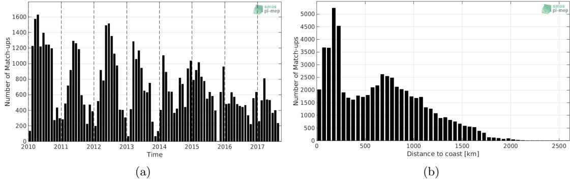
Figure 1: Number of match-ups between Sea mammals and SMOS-L3-CATDS-CECOS-LOCEAN-V4-9DAYS-25KM SSS as a function of time (a) and as function of the distance to coast (b) over the Southern Ocean Pi-MEP region and for the full satellite product period.
