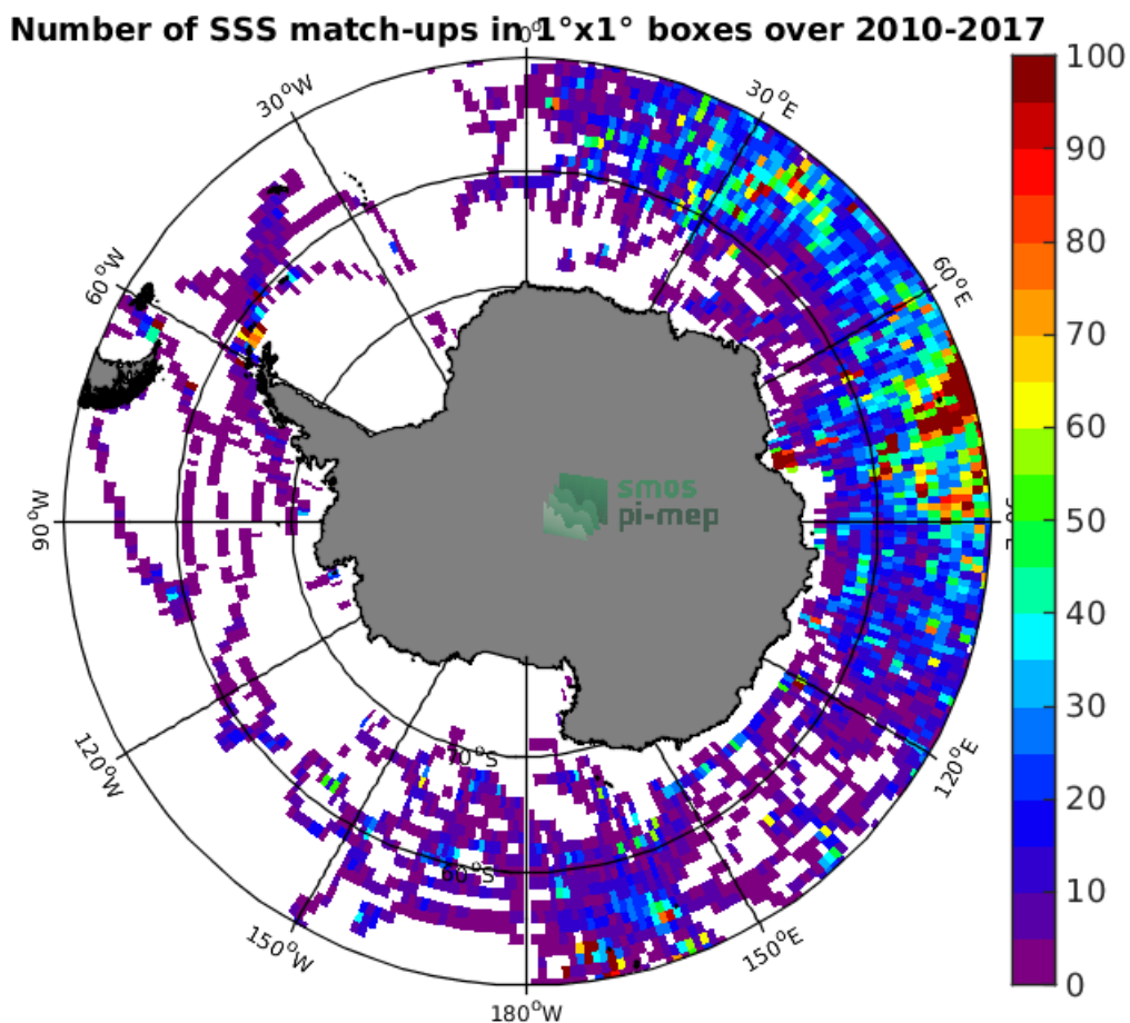
Figure 4: Number of SSS match-ups between Sea mammals SSS and the SMOS-L3-CATDS-CECOS-LOCEAN-V4-9DAYS-25KM SSS product for the Southern Ocean Pi-MEP region over 1^\circ \times 1^\circ boxes and for the full satellite product period.
