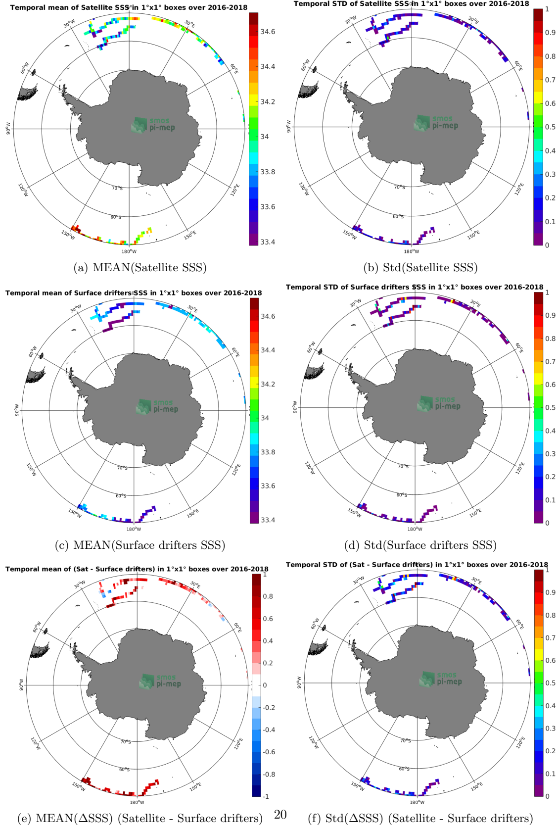
Figure 5: Temporal mean (left) and Std (right) of SSS from SMOS SSS L3 v4 - 9 Days (CATDS-CECOS-LOCEAN) (top), Surface drifters (middle), and of \Delta SSS (Satellite - Surface drifters). Only match-up pairs are used to generate these maps.
