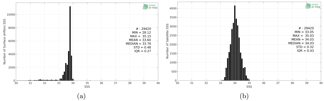
Figure 2: Histograms of SSS from Surface drifters (a) and SMOS SSS L3 v4 - 9 Days (CATDS-CECOS-LOCEAN) (b) considering all match-up pairs per bins of 0.1 over the Southern Ocean Pi-MEP region and for the full satellite product period.
