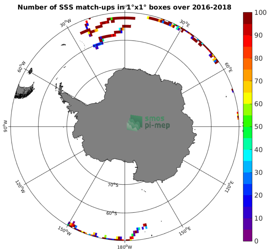
Figure 3: Number of SSS match-ups between Surface drifters SSS and the SMOS SSS L3 v4 - 9 Days (CATDS-CECOS-LOCEAN) SSS product for the Southern Ocean Pi-MEP region over 1^\circ \times 1^\circ boxes and for the full satellite product period.
