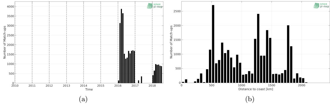
Figure 1: Number of match-ups between Surface drifters and SMOS SSS L3 v4 - 9 Days (CATDS-CECOS-LOCEAN) SSS as a function of time (a) and as function of the distance to coast (b) over the Southern Ocean Pi-MEP region and for the full satellite product period.
