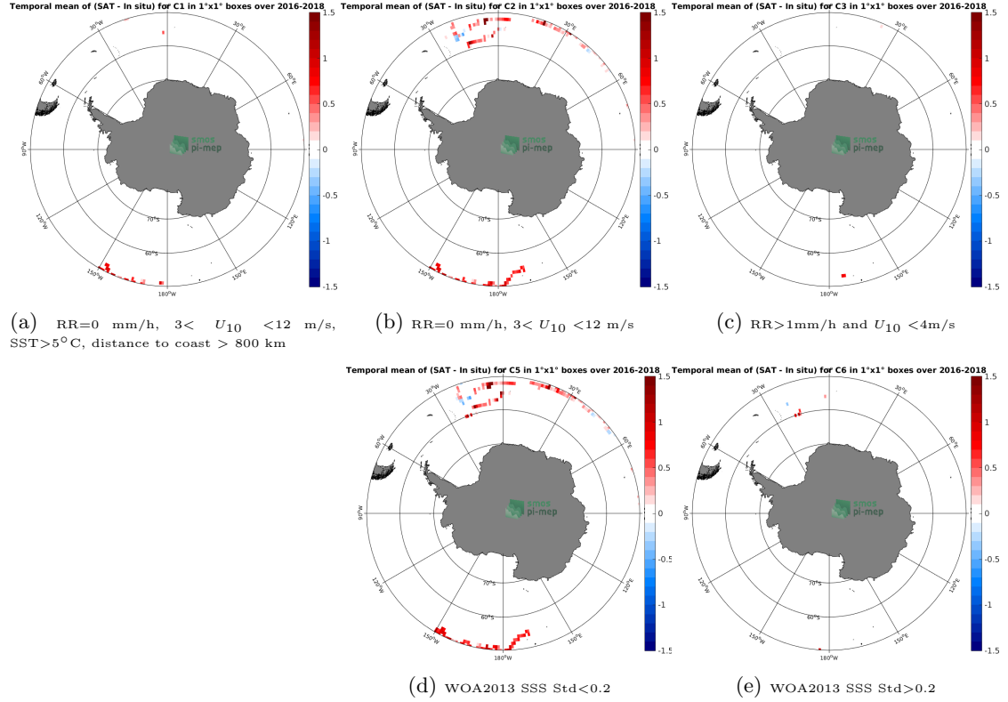
Figure 11: Temporal mean gridded over spatial boxes of size 1^{\circ}\times 1^{\circ} of \Delta\text{SSS} (SMOS SSS L3 v4 - 9 Days (CATDS-CECOS-LOCEAN) - Surface drifters) for 5 different subdatasets corresponding to: RR=0 mm/h, 3 < U_{10} < 12 m/s, SST > 5^{\circ}\text{C} , distance to coast > 800 km (a), RR=0 mm/h, 3 < U_{10} < 12 m/s (b), RR > 1 mm/h and U_{10} < 4 m/s (c), WOA2013 SSS Std < 0.2 (d), WOA2013 SSS Std > 0.2 (e).
