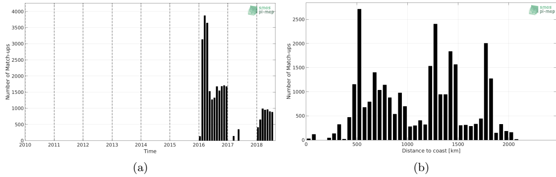
Figure 1: Number of match-ups between Surface drifters and SMOS-L3-CATDS-CECOS-LOCEAN-V4-9DAYS-25KM SSS as a function of time (a) and as function of the distance to coast (b) over the Southern Ocean Pi-MEP region and for the full satellite product period.
