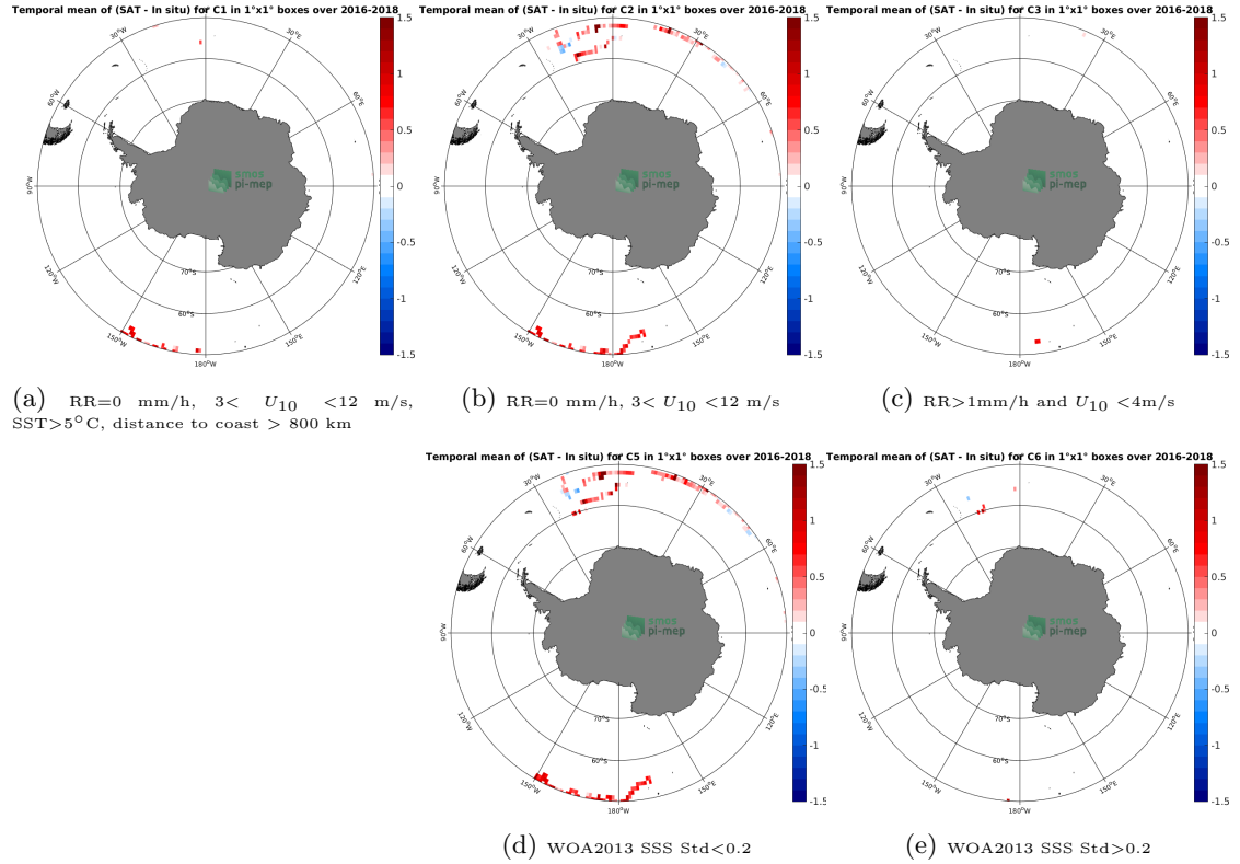
Figure 11: Temporal mean gridded over spatial boxes of size 1^{\circ}\times 1^{\circ} of \Delta\text{SSS} (SMOS-L3-CATDS-CECOS-LOCEAN-V4-9DAYS-25KM - Surface drifters) for 5 different subdatasets corresponding to: RR=0 mm/h, 3 < U_{10} < 12 m/s, SST >5^{\circ}\text{C} , distance to coast > 800 km (a), RR=0 mm/h, 3 < U_{10} < 12 m/s (b), RR >1 mm/h and U_{10} < 4 m/s (c), WOA2013 SSS Std <0.2 (d), WOA2013 SSS Std >0.2 (e).
