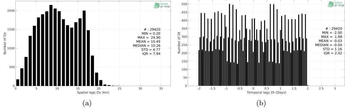
Figure 4: Histograms of the spatial (a) and temporal (b) lags between the time of the Surface drifters measurements and the date of the corresponding SMOS-L3-CATDS-CECOS-LOCEAN-V4-9DAYS-25KM SSS product.
