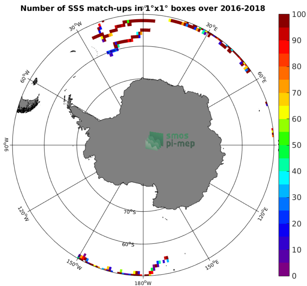
Figure 3: Number of SSS match-ups between Surface drifters SSS and the SMOS-L3-CATDS-CECOS-LOCEAN-V4-9DAYS-25KM SSS product for the Southern Ocean Pi-MEP region over 1^\circ \times 1^\circ boxes and for the full satellite product period.
