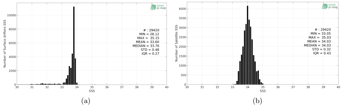
Figure 2: Histograms of SSS from Surface drifters (a) and SMOS-L3-CATDS-CECOS-LOCEAN-V4-9DAYS-25KM (b) considering all match-up pairs per bins of 0.1 over the Southern Ocean Pi-MEP region and for the full satellite product period.
