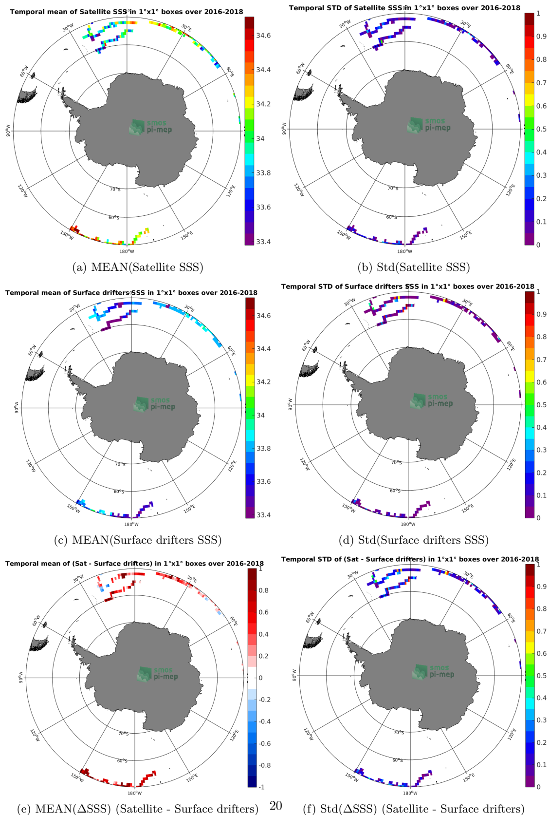
Figure 5: Temporal mean (left) and Std (right) of SSS from SMOS-L3-CATDS-CECOS-LOCEAN-V4-9DAYS-25KM (top), Surface drifters (middle), and of \Delta SSS (Satellite - Surface drifters). Only match-up pairs are used to generate these maps.
