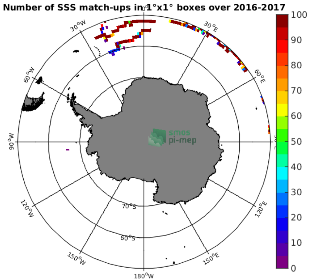
Figure 3: Number of SSS match-ups between Surface drifters SSS and the SMOS-L3-CATDS-CECOS-LOCEAN-V4-9DAYS-25KM SSS product for the Southern Ocean Pi-MEP region over 1^\circ \times 1^\circ boxes and for the full satellite product period.
