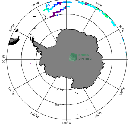
(c) MEAN(Surface drifters SSS)
