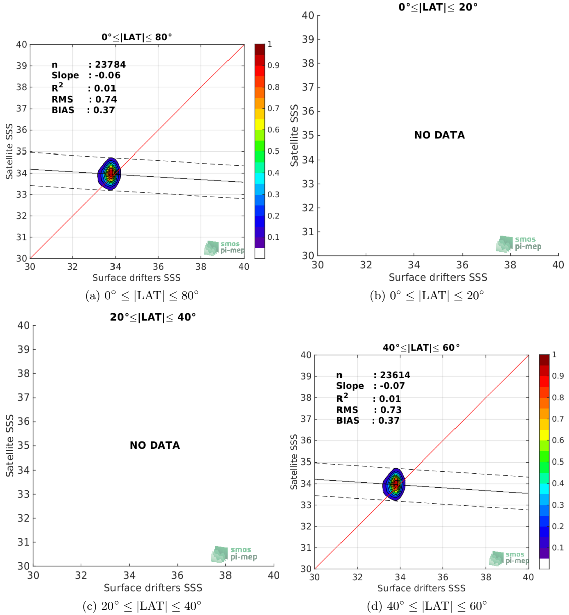
Figure 8: Contour maps of the concentration of SMOS-L3-CATDS-CECOS-LOCEAN-V4-9DAYS-25KM SSS (y-axis) versus Surface drifters SSS (x-axis) at match-up pairs for different latitude bands. For each plot, the red line shows x=y . The black thin and dashed lines indicate a linear fit through the data cloud and the \pm 95\% confidence levels, respectively. The number match-up pairs n , the slope and R^2 coefficient of the linear fit, the root mean square (RMS) and the mean bias between satellite and in situ data are indicated for each latitude band in each plots.
