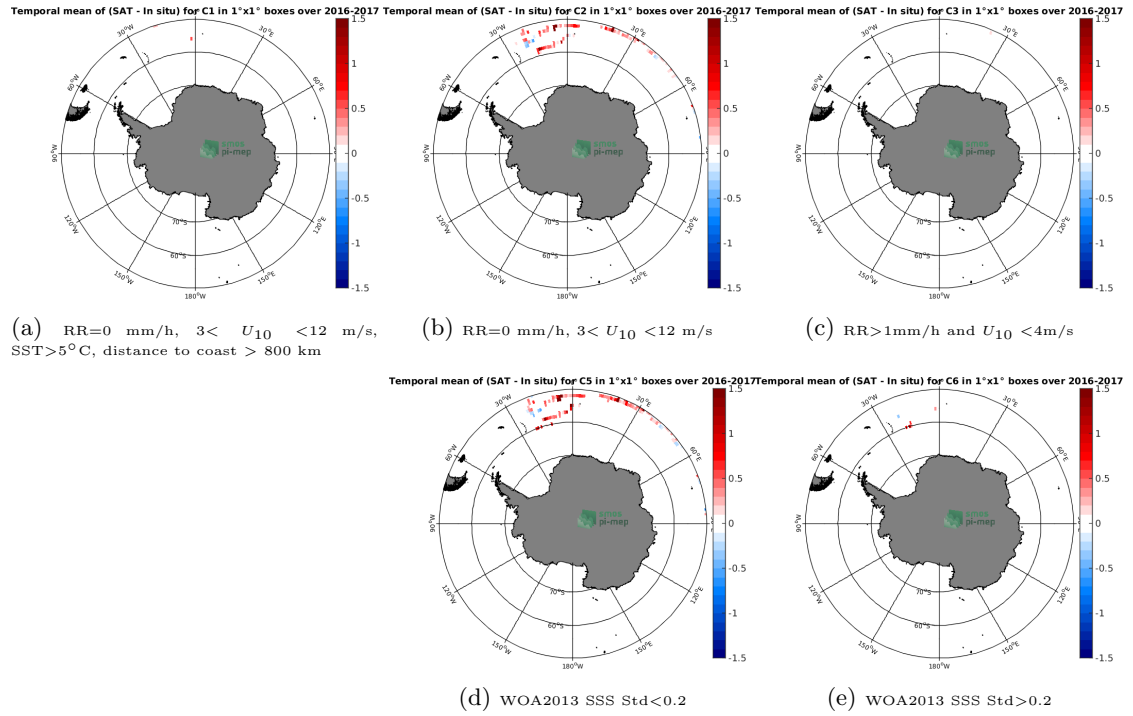
Figure 11: Temporal mean gridded over spatial boxes of size 1^\circ \times 1^\circ of \Delta SSS (SMOS-L3-CATDS-CECOS-LOCEAN-V4-9DAYS-25KM - Surface drifters) for 5 different subdatasets corresponding to: RR=0 mm/h, 3 < U_{10} < 12 m/s, SST > 5^\circ\text{C} , distance to coast > 800 km (a), RR=0 mm/h, 3 < U_{10} < 12 m/s (b), RR > 1 mm/h and U_{10} < 4 m/s (c), WOA2013 SSS Std < 0.2 (d), WOA2013 SSS Std > 0.2 (e).
