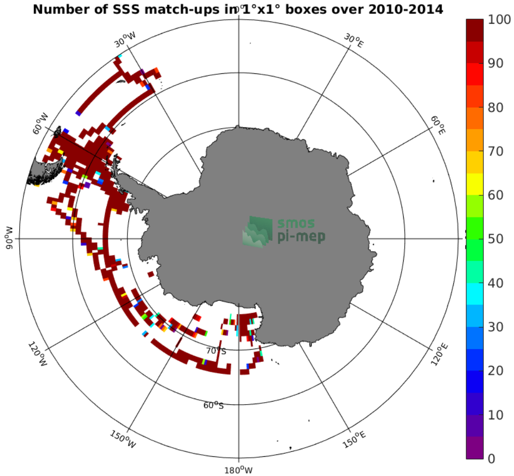
Figure 4: Number of SSS match-ups between TSG (SAMOS) SSS and the SMOS SSS L3 v4 - 18 Days (CATDS-CECOS-LOCEAN) SSS product for the Southern Ocean Pi-MEP region over 1°x1° boxes and for the full satellite product period.
