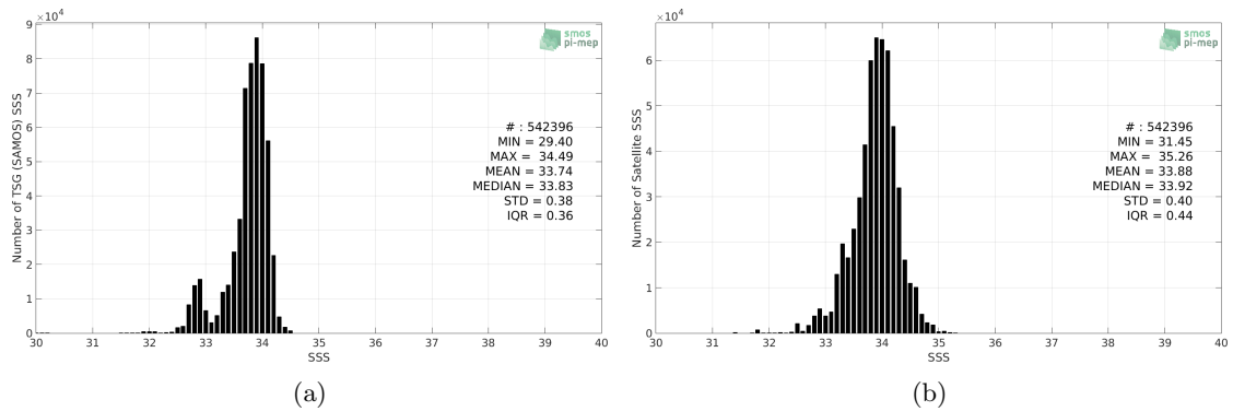
Figure 2: Histograms of SSS from TSG (SAMOS) (a) and SMOS SSS L3 v4 - 18 Days (CATDS-CECOS-LOCEAN) (b) considering all match-up pairs per bins of 0.1 over the Southern Ocean Pi-MEP region and for the full satellite product period.
