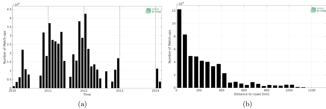
Figure 1: Number of match-ups between TSG (SAMOS) and SMOS SSS L3 v4 - 18 Days (CATDS-CECOS-LOCEAN) SSS as a function of time (a) and as function of the distance to coast (b) over the Southern Ocean Pi-MEP region and for the full satellite product period.
