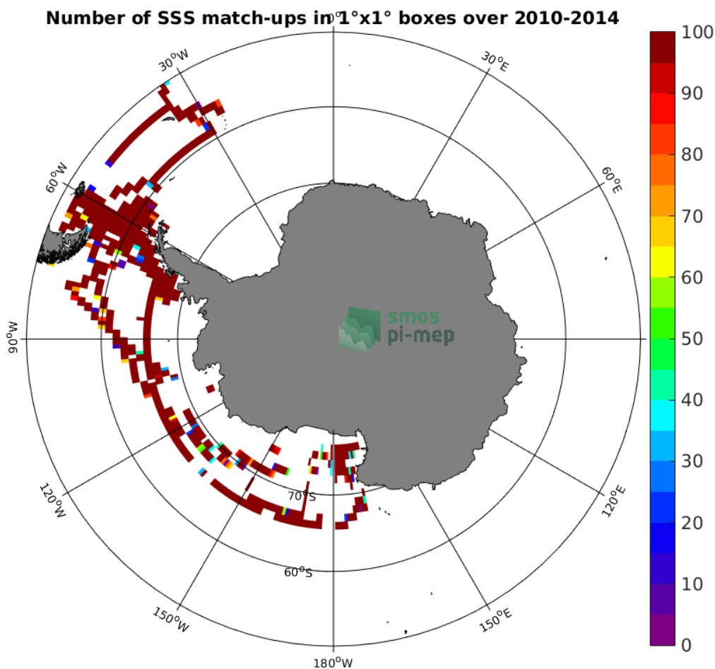
Figure 4: Number of SSS match-ups between TSG-SAMOS SSS and the SMOS-L3-CATDS-CECOS-LOCEAN-V4-18DAYS-25KM SSS product for the Southern Ocean Pi-MEP region over 1°x1° boxes and for the full satellite product period.
