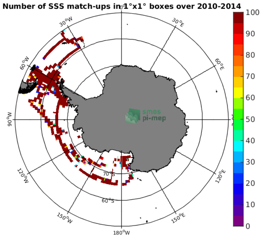
Figure 4: Number of SSS match-ups between TSG-SAMOS SSS and the SMOS-L3-CATDS-CECOS-LOCEAN-V4-18DAYS-25KM SSS product for the Southern Ocean Pi-MEP region over 1°x1° boxes and for the full satellite product period.
