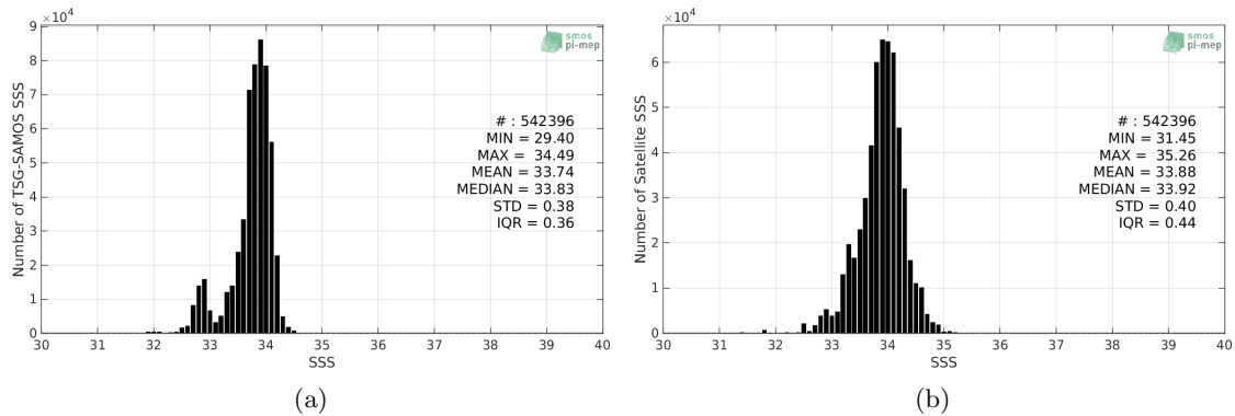
Figure 2: Histograms of SSS from TSG-SAMOS (a) and SMOS-L3-CATDS-CECOS-LOCEAN-V4-18DAYS-25KM (b) considering all match-up pairs per bins of 0.1 over the Southern Ocean Pi-MEP region and for the full satellite product period.
