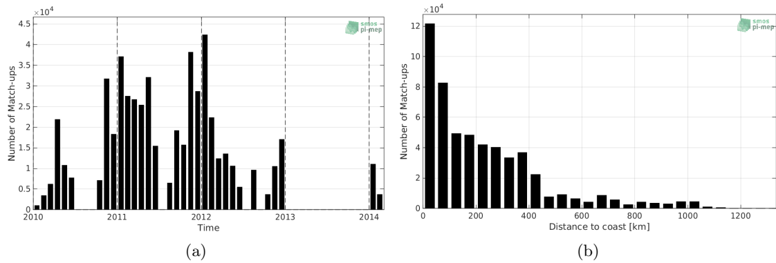
Figure 1: Number of match-ups between TSG-SAMOS and SMOS-L3-CATDS-CECOS-LOCEAN-V4-18DAYS-25KM SSS as a function of time (a) and as function of the distance to coast (b) over the Southern Ocean Pi-MEP region and for the full satellite product period.
