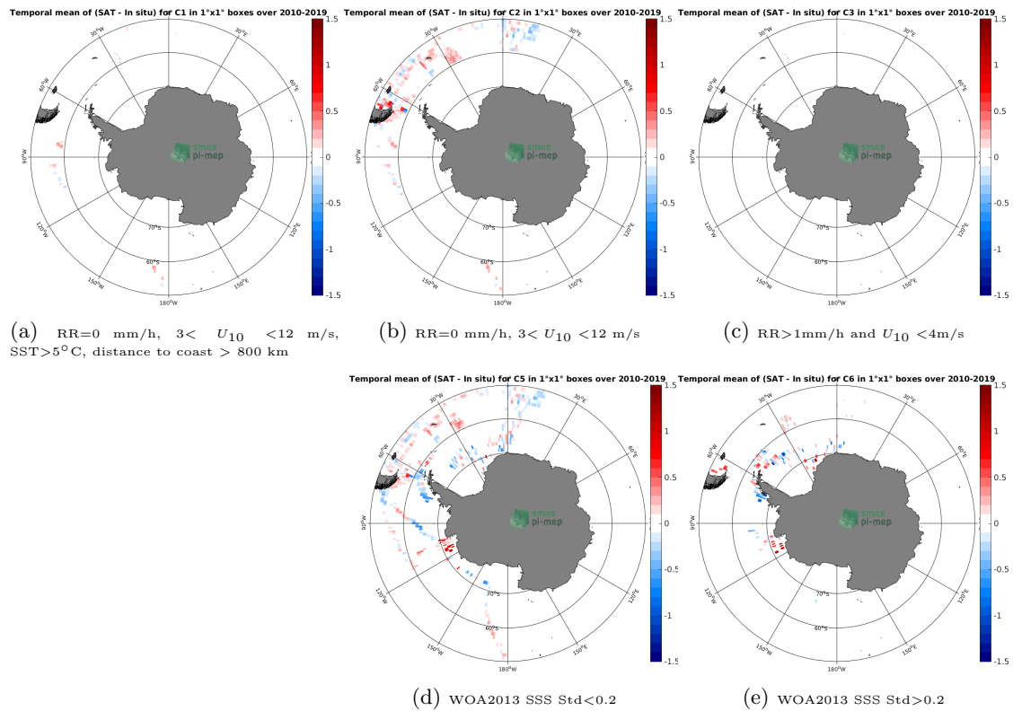
Figure 12: Temporal mean gridded over spatial boxes of size 1^{\circ}\times 1^{\circ} of \Delta\text{SSS} (SMOS-L3-CATDS-CECOS-LOCEAN-V4-18DAYS-25KM - TSG-POLARSTERN) for 5 different subdatasets corresponding to:RR=0 mm/h, 3 < U_{10} < 12 m/s, SST >5^{\circ}\text{C} , distance to coast > 800 km (a), RR=0 mm/h, 3 < U_{10} < 12 m/s (b), RR >1 mm/h and U_{10} < 4 m/s (c), WOA2013 SSS Std <0.2 (d), WOA2013 SSS Std >0.2 (e).
