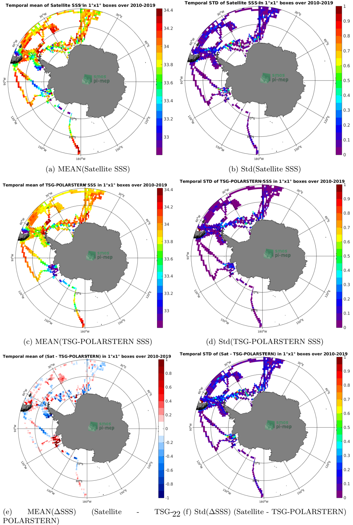
Figure 6: Temporal mean (left) and Std (right) of SSS from SMOS-L3-CATDS-CECOS-LOCEAN-V4-18DAYS-25KM (top), TSG-POLARSTERN (middle), and of \Delta SSS (Satellite - TSG-POLARSTERN). Only match-up pairs are used to generate these maps.
