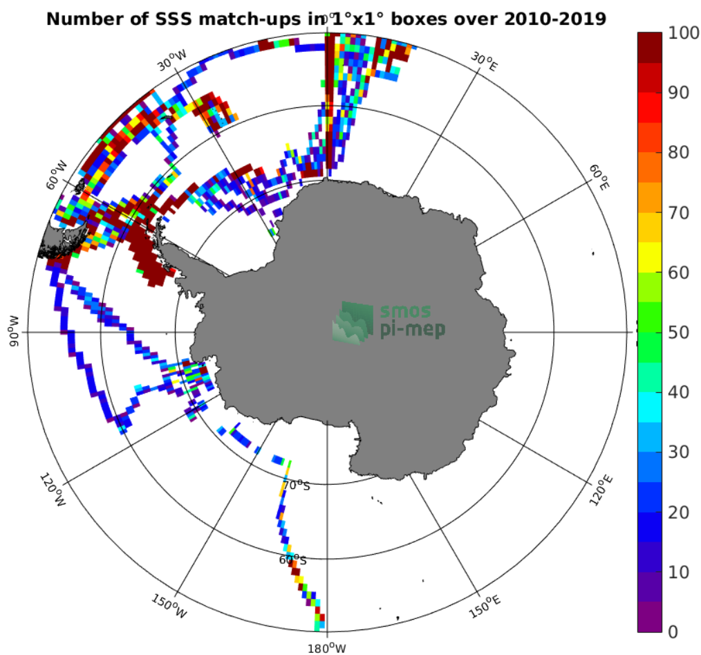
Figure 4: Number of SSS match-ups between TSG-POLARSTERN SSS and the SMOS-L3-CATDS-CECOS-LOCEAN-V4-18DAYS-25KM SSS product for the Southern Ocean Pi-MEP region over 1°x1° boxes and for the full satellite product period.
