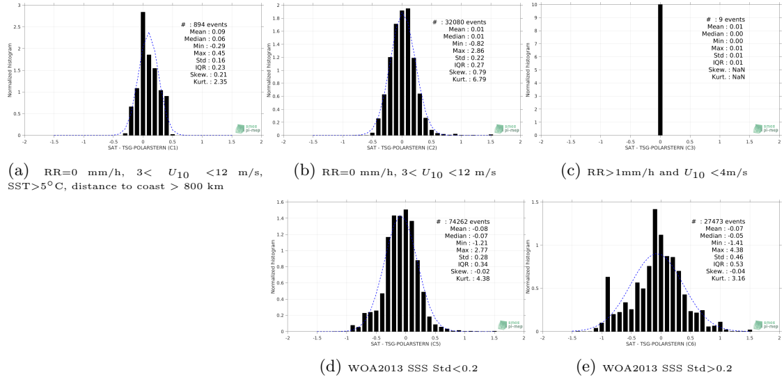
Figure 13: Normalized histogram of \Delta SSS (SMOS-L3-CATDS-CECOS-LOCEAN-V4-18DAYS-25KM - TSG-POLARSTERN) for 5 different subdatasets corresponding to: RR=0 mm/h, 3 < U_{10} < 12 m/s, SST>5°C, distance to coast > 800 km (a), RR=0 mm/h, 3 < U_{10} < 12 m/s (b), RR>1mm/h and U_{10} < 4 m/s (c), WOA2013 SSS Std<0.2 (d), WOA2013 SSS Std>0.2 (e).
