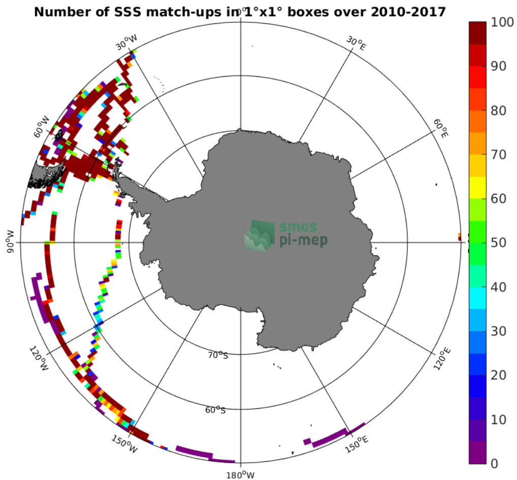
Figure 4: Number of SSS match-ups between TSG (GOSUD-Sailing-ship) SSS and the SMOS SSS L3 v4 - 18 Days (CATDS-CECOS-LOCEAN) SSS product for the Southern Ocean Pi-MEP region over 1^\circ \times 1^\circ boxes and for the full satellite product period.
