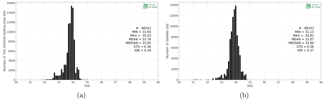
Figure 2: Histograms of SSS from TSG (GOSUD-Sailing-ship) (a) and SMOS SSS L3 v4 - 18 Days (CATDS-CECOS-LOCEAN) (b) considering all match-up pairs per bins of 0.1 over the Southern Ocean Pi-MEP region and for the full satellite product period.
