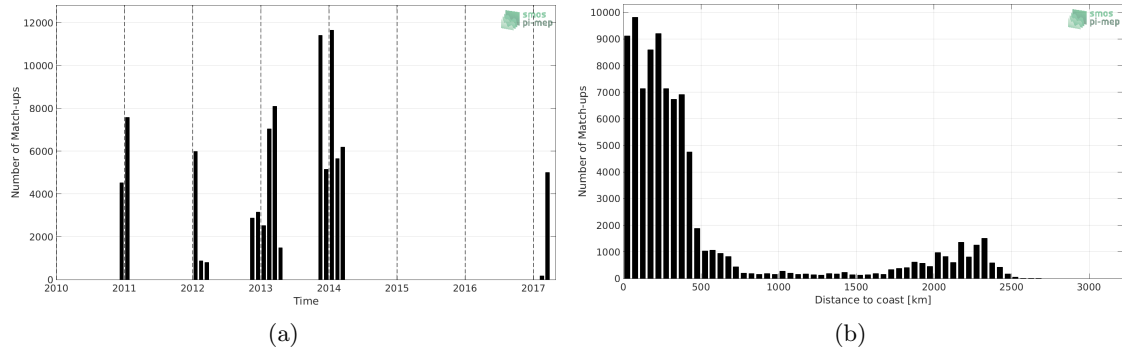
Figure 1: Number of match-ups between TSG (GOSUD-Sailing-ship) and SMOS SSS L3 v4 - 18 Days (CATDS-CECOS-LOCEAN) SSS as a function of time (a) and as function of the distance to coast (b) over the Southern Ocean Pi-MEP region and for the full satellite product period.
