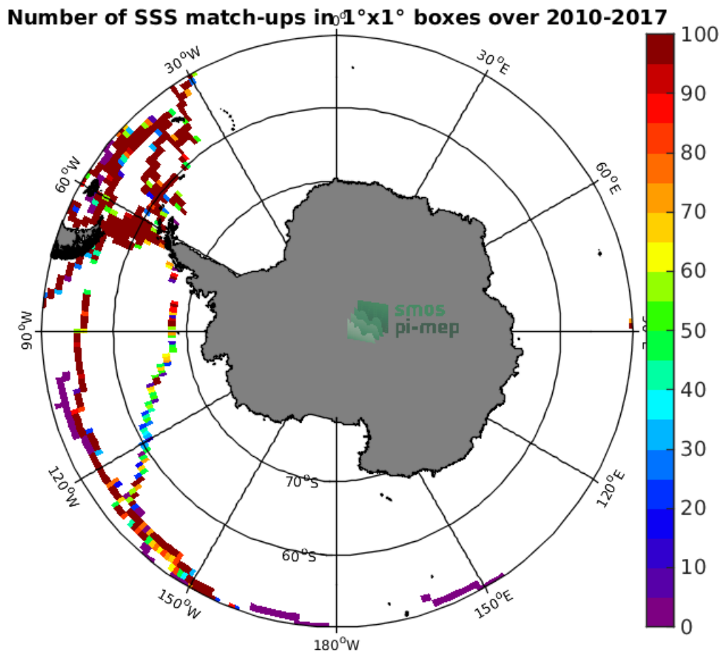
Figure 4: Number of SSS match-ups between TSG-GOSUD-Sailing-ship SSS and the SMOS-L3-CATDS-CECOS-LOCEAN-V4-18DAYS-25KM SSS product for the Southern Ocean Pi-MEP region over 1°x1° boxes and for the full satellite product period.
