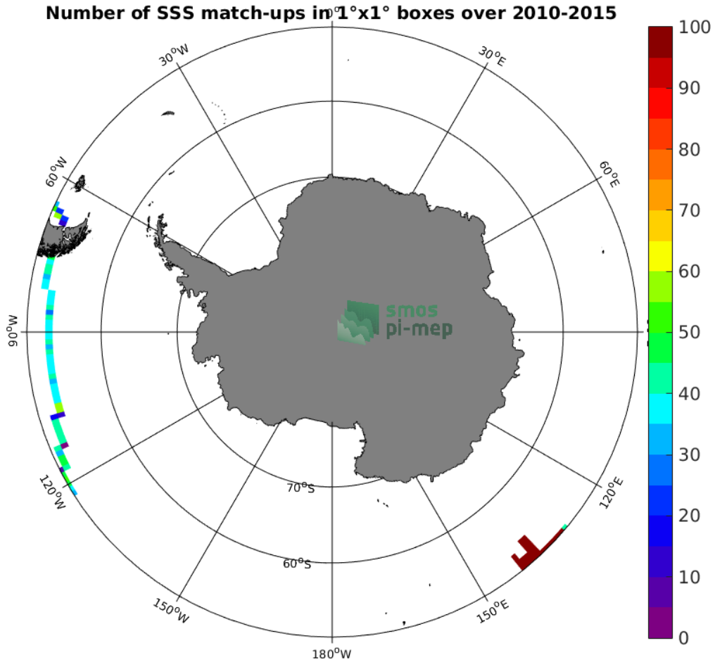
Figure 4: Number of SSS match-ups between TSG (GOSUD-Research-vessel) SSS and the SMOS SSS L3 v4 - 18 Days (CATDS-CECOS-LOCEAN) SSS product for the Southern Ocean Pi-MEP region over 1°x1° boxes and for the full satellite product period.
