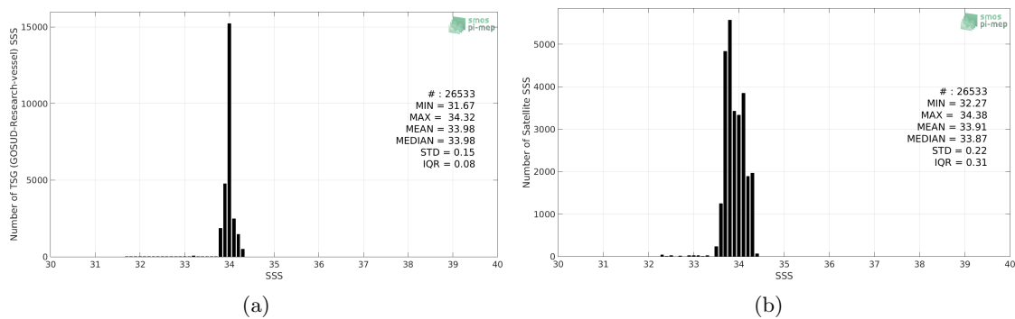
Figure 2: Histograms of SSS from TSG (GOSUD-Research-vessel) (a) and SMOS SSS L3 v4 - 18 Days (CATDS-CECOS-LOCEAN) (b) considering all match-up pairs per bins of 0.1 over the Southern Ocean Pi-MEP region and for the full satellite product period.
