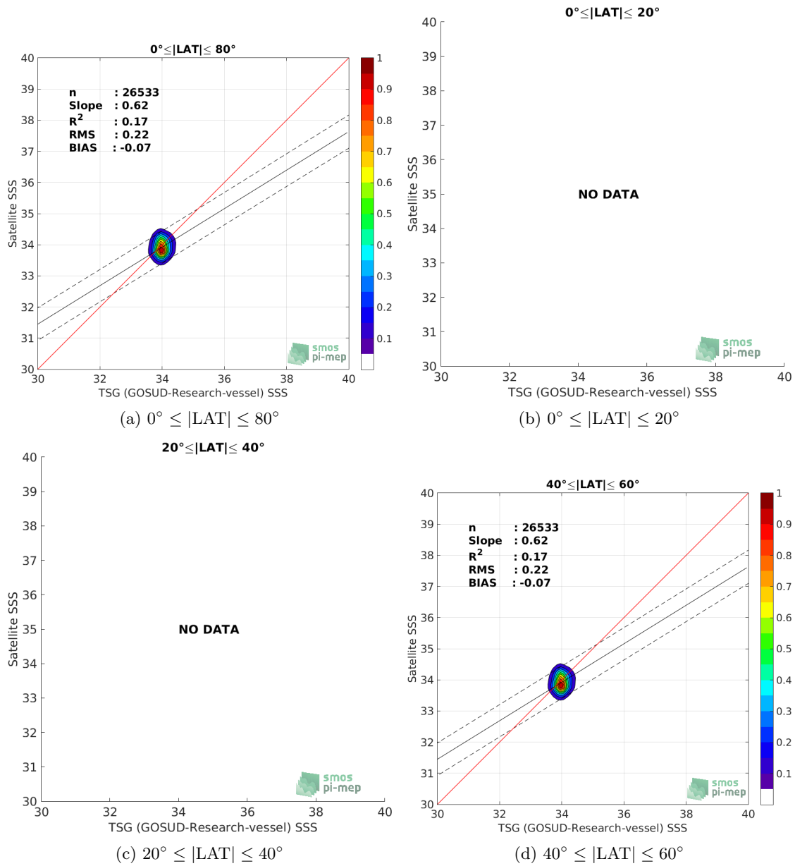
Figure 9: Contour maps of the concentration of SMOS SSS L3 v4 - 18 Days (CATDS-CECOS-LOCEAN) SSS ( y -axis) versus TSG (GOSUD-Research-vessel) SSS ( x -axis) at match-up pairs for different latitude bands. For each plot, the red line shows x=y . The black thin and dashed lines indicate a linear fit through the data cloud and the \pm 95\% confidence levels, respectively. The number match-up pairs n , the slope and R^2 coefficient of the linear fit, the root mean square (RMS) and the mean bias between satellite and in situ data are indicated for each latitude band in each plots.
