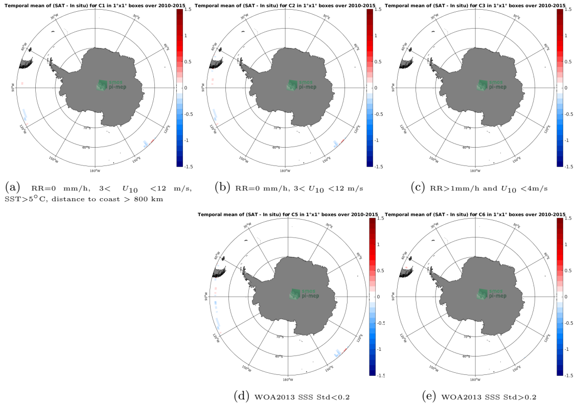
Figure 12: Temporal mean gridded over spatial boxes of size 1°x1° of \Delta SSS (SMOS SSS L3 v4 - 18 Days (CATDS-CECOS-LOCEAN) - TSG (GOSUD-Research-vessel)) for 5 different subdatasets corresponding to: RR=0 mm/h, 3 < U_{10} < 12 m/s, SST > 5°C, distance to coast > 800 km (a), RR=0 mm/h, 3 < U_{10} < 12 m/s (b), RR > 1mm/h and U_{10} < 4 m/s (c), WOA2013 SSS Std < 0.2 (d), WOA2013 SSS Std > 0.2 (e).
