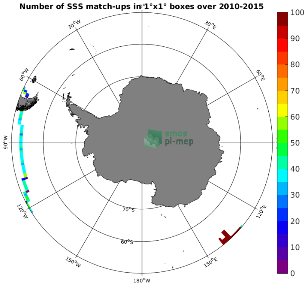
Figure 4: Number of SSS match-ups between TSG-GOSUD-Research-vessel SSS and the SMOS-L3-CATDS-CECOS-LOCEAN-V4-18DAYS-25KM SSS product for the Southern Ocean Pi-MEP region over 1°x1° boxes and for the full satellite product period.
