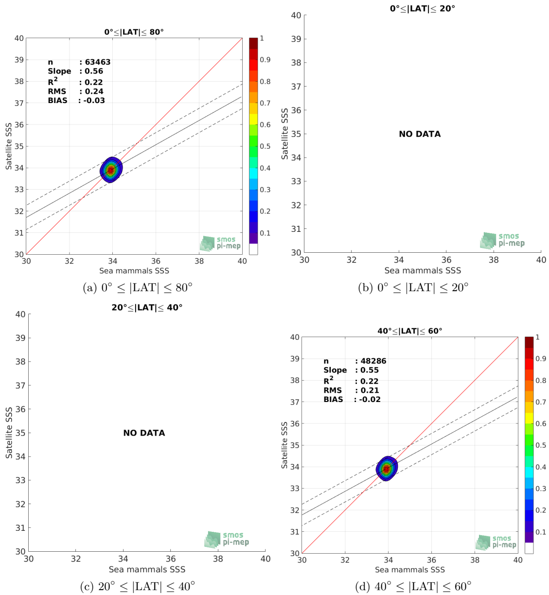
Figure 9: Contour maps of the concentration of SMOS SSS L3 v4 - 18 Days (CATDS-CECOS-LOCEAN) SSS (y-axis) versus Sea mammals SSS (x-axis) at match-up pairs for different latitude bands. For each plot, the red line shows x=y . The black thin and dashed lines indicate a linear fit through the data cloud and the \pm 95\% confidence levels, respectively. The number match-up pairs n , the slope and R^2 coefficient of the linear fit, the root mean square (RMS) and the mean bias between satellite and in situ data are indicated for each latitude band in each plots.
