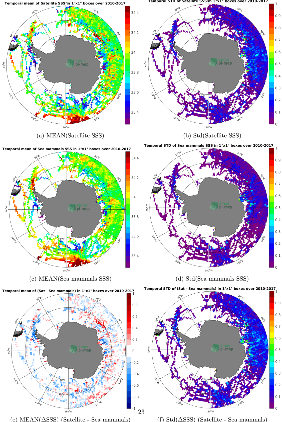
Figure 6: Temporal mean (left) and Std (right) of SSS from SMOS SSS L3 v4 - 18 Days (CATDS-CECOS-LOCEAN) (top), Sea mammals (middle), and of \Delta SSS (Satellite - Sea mammals). Only match-up pairs are used to generate these maps.
