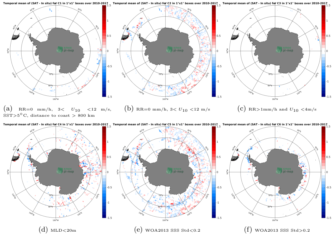
Figure 12: Temporal mean gridded over spatial boxes of size 1^{\circ}\times 1^{\circ} of \Delta\text{SSS} (SMOS SSS L3 v4 - 18 Days (CATDS-CECOS-LOCEAN) - Sea mammals) for 6 different subdatasets corresponding to: RR=0 mm/h, 3 < U_{10} < 12 m/s, SST > 5^{\circ}\text{C} , distance to coast > 800 km (a), RR=0 mm/h, 3 < U_{10} < 12 m/s (b), RR > 1 mm/h and U_{10} < 4 m/s (c), MLD < 20 m (d), WOA2013 SSS Std < 0.2 (e), WOA2013 SSS Std > 0.2 (f).
