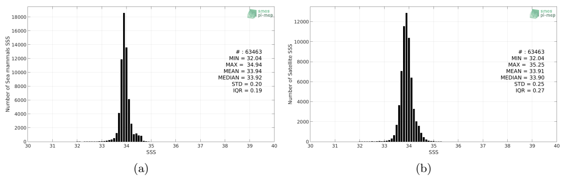
Figure 2: Histograms of SSS from Sea mammals (a) and SMOS SSS L3 v4 - 18 Days (CATDS-CECOS-LOCEAN) (b) considering all match-up pairs per bins of 0.1 over the Southern Ocean Pi-MEP region and for the full satellite product period.
