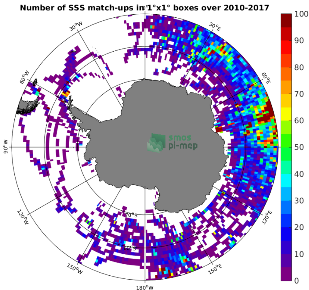
Figure 4: Number of SSS match-ups between Sea mammals SSS and the SMOS SSS L3 v4 - 18 Days (CATDS-CECOS-LOCEAN) SSS product for the Southern Ocean Pi-MEP region over 1°x1° boxes and for the full satellite product period.
