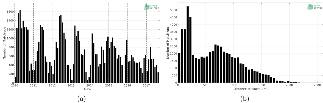
Figure 1: Number of match-ups between Sea mammals and SMOS SSS L3 v4 - 18 Days (CATDS-CECOS-LOCEAN) SSS as a function of time (a) and as function of the distance to coast (b) over the Southern Ocean Pi-MEP region and for the full satellite product period.
