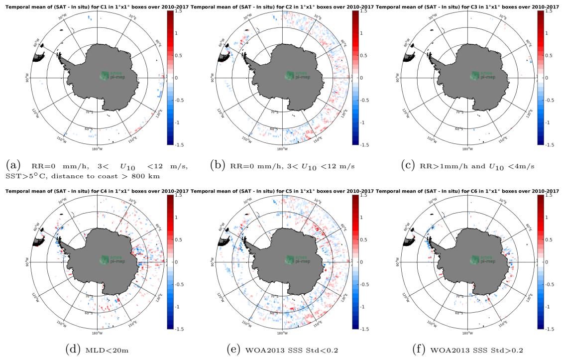
Figure 12: Temporal mean gridded over spatial boxes of size 1^\circ \times 1^\circ of \Delta SSS (SMOS-L3-CATDS-CECOS-LOCEAN-V4-18DAYS-25KM - Sea mammals) for 6 different subdatasets corresponding to:RR=0 mm/h, 3 < U_{10} < 12 m/s, SST>5°C, distance to coast > 800 km (a), RR=0 mm/h, 3 < U_{10} < 12 m/s (b), RR>1mm/h and U_{10} < 4 m/s (c),MLD<20m (d),WOA2013 SSS Std<0.2 (e),WOA2013 SSS Std>0.2 (f).
