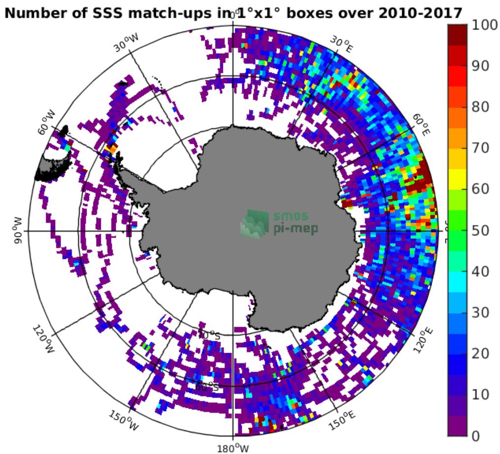
Figure 4: Number of SSS match-ups between Sea mammals SSS and the SMOS-L3-CATDS-CECOS-LOCEAN-V4-18DAYS-25KM SSS product for the Southern Ocean Pi-MEP region over 1^\circ \times 1^\circ boxes and for the full satellite product period.
