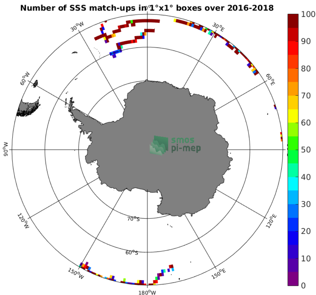
Figure 3: Number of SSS match-ups between Surface drifters SSS and the SMOS SSS L3 v4 - 18 Days (CATDS-CECOS-LOCEAN) SSS product for the Southern Ocean Pi-MEP region over 1^\circ \times 1^\circ boxes and for the full satellite product period.
