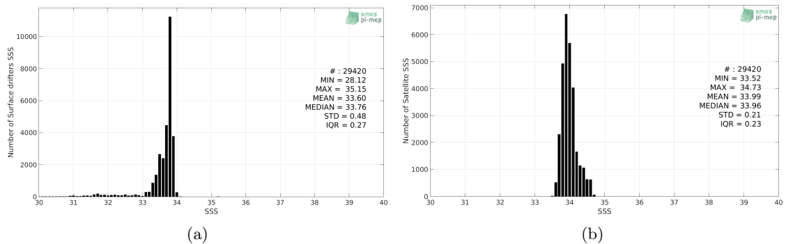
Figure 2: Histograms of SSS from Surface drifters (a) and SMOS SSS L3 v4 - 18 Days (CATDS-CECOS-LOCEAN) (b) considering all match-up pairs per bins of 0.1 over the Southern Ocean Pi-MEP region and for the full satellite product period.
