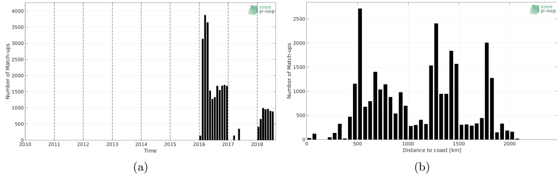
Figure 1: Number of match-ups between Surface drifters and SMOS SSS L3 v4 - 18 Days (CATDS-CECOS-LOCEAN) SSS as a function of time (a) and as function of the distance to coast (b) over the Southern Ocean Pi-MEP region and for the full satellite product period.
