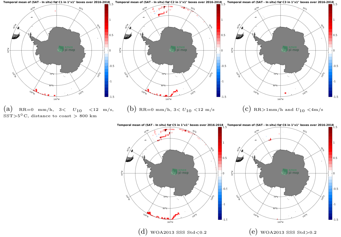
Figure 11: Temporal mean gridded over spatial boxes of size 1^{\circ}\times 1^{\circ} of \Delta\text{SSS} (SMOS SSS L3 v4 - 18 Days (CATDS-CECOS-LOCEAN) - Surface drifters) for 5 different subdatasets corresponding to:RR=0 mm/h, 3 < U_{10} < 12 m/s, SST >5^{\circ}\text{C} , distance to coast > 800 km (a), RR=0 mm/h, 3 < U_{10} < 12 m/s (b), RR >1 mm/h and U_{10} < 4 m/s (c), WOA2013 SSS Std <0.2 (d), WOA2013 SSS Std >0.2 (e).
