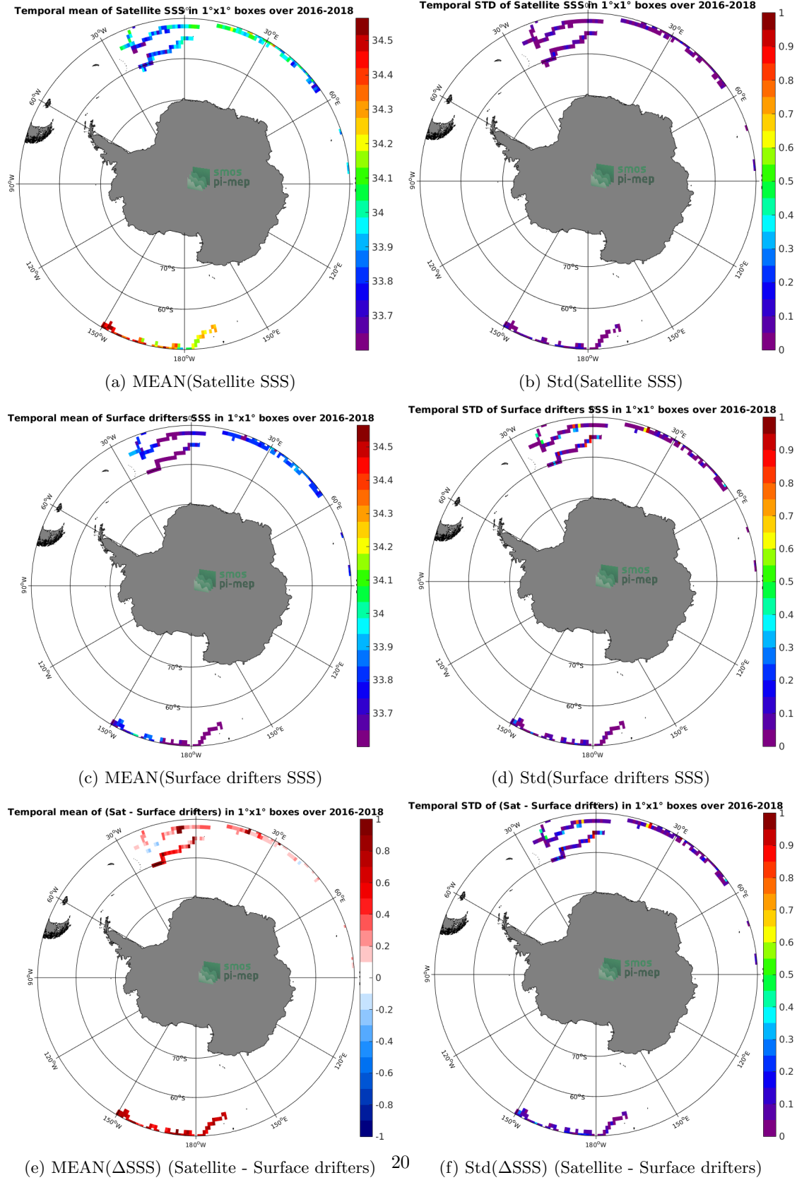
Figure 5: Temporal mean (left) and Std (right) of SSS from SMOS SSS L3 v4 - 18 Days (CATDS-CECOS-LOCEAN) (top), Surface drifters (middle), and of \Delta SSS (Satellite - Surface drifters). Only match-up pairs are used to generate these maps.
