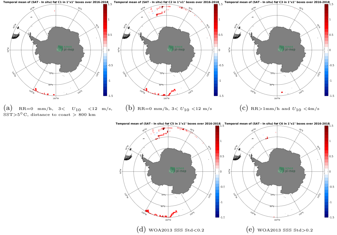
Figure 11: Temporal mean gridded over spatial boxes of size 1^{\circ}\times 1^{\circ} of \Delta\text{SSS} (SMOS-L3-CATDS-CECOS-LOCEAN-V4-18DAYS-25KM - Surface drifters) for 5 different subdatasets corresponding to: RR=0 mm/h, 3 < U_{10} < 12 m/s, SST >5^{\circ}\text{C} , distance to coast > 800 km (a), RR=0 mm/h, 3 < U_{10} < 12 m/s (b), RR >1 mm/h and U_{10} < 4 m/s (c), WOA2013 SSS Std <0.2 (d), WOA2013 SSS Std >0.2 (e).
