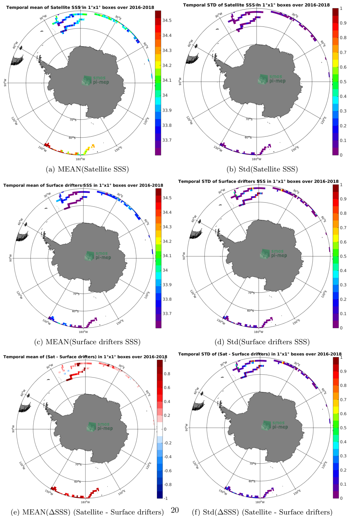
Figure 5: Temporal mean (left) and Std (right) of SSS from SMOS-L3-CATDS-CECOS-LOCEAN-V4-18DAYS-25KM (top), Surface drifters (middle), and of \Delta SSS (Satellite - Surface drifters). Only match-up pairs are used to generate these maps.
