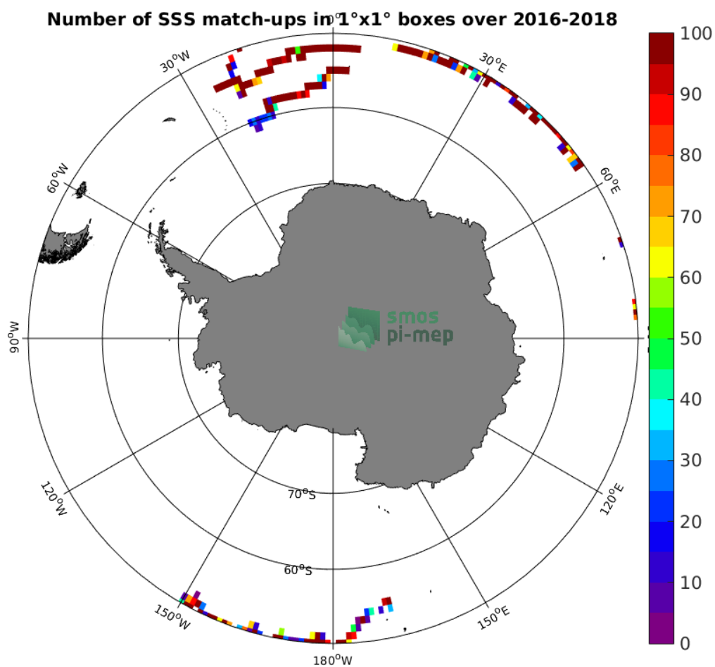
Figure 3: Number of SSS match-ups between Surface drifters SSS and the SMOS-L3-CATDS-CECOS-LOCEAN-V4-18DAYS-25KM SSS product for the Southern Ocean Pi-MEP region over 1^\circ \times 1^\circ boxes and for the full satellite product period.
