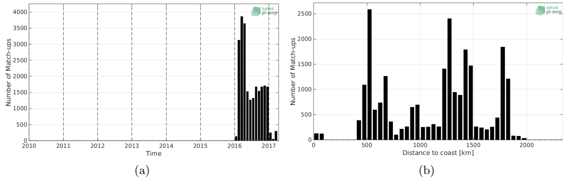
Figure 1: Number of match-ups between Surface drifters and SMOS-L3-CATDS-CECOS-LOCEAN-V4-18DAYS-25KM SSS as a function of time (a) and as function of the distance to coast (b) over the Southern Ocean Pi-MEP region and for the full satellite product period.
