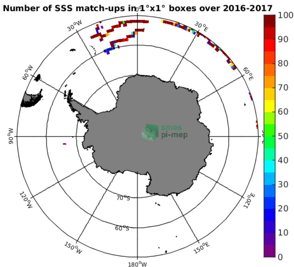
Figure 3: Number of SSS match-ups between Surface drifters SSS and the SMOS-L3-CATDS-CECOS-LOCEAN-V4-18DAYS-25KM SSS product for the Southern Ocean Pi-MEP region over 1^\circ \times 1^\circ boxes and for the full satellite product period.
