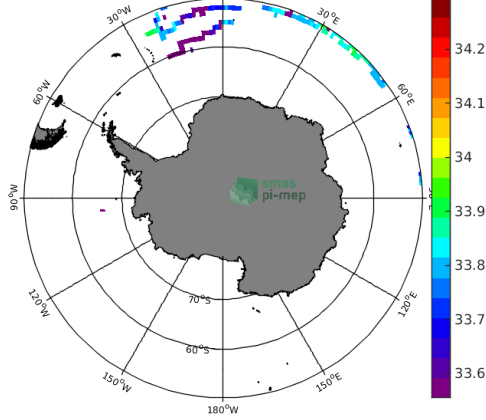
(c) MEAN(Surface drifters SSS)
