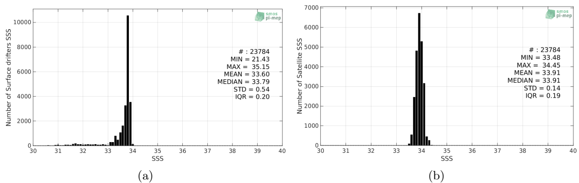
Figure 2: Histograms of SSS from Surface drifters (a) and SMOS-L3-CATDS-CECOS-LOCEAN-V4-18DAYS-25KM (b) considering all match-up pairs per bins of 0.1 over the Southern Ocean Pi-MEP region and for the full satellite product period.
